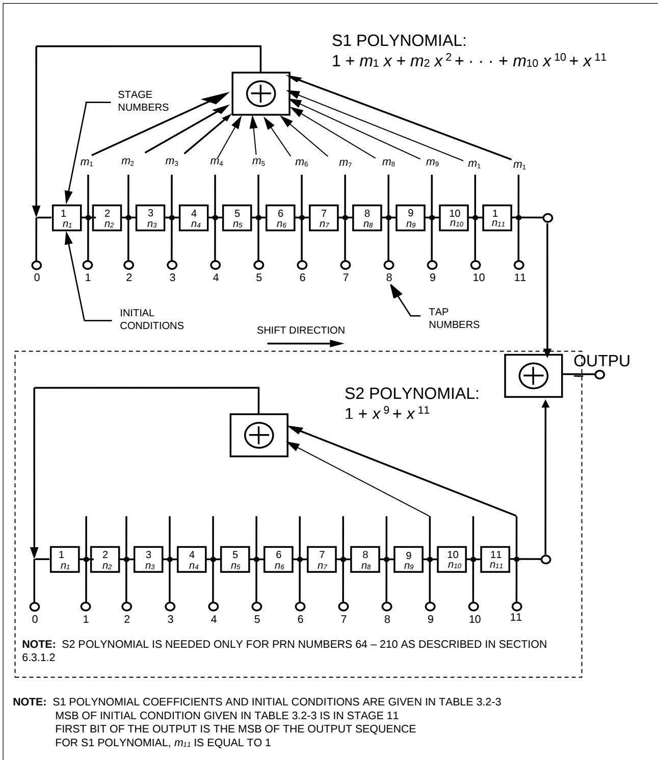
Figure 3.2-2. L1Co-Code Generator Configuration
