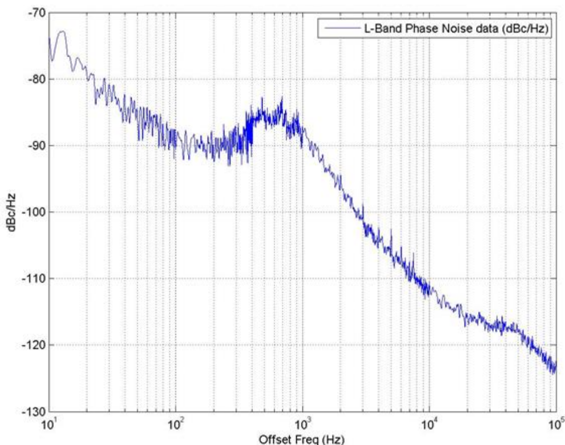
Figure 6-1 Typical GPS III and GPS IIIIF L1C Carrier Phase Noise Spectral Density
