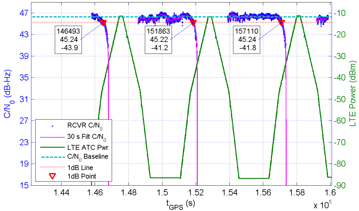
Receiver 131 Average C/N_0 for All Channels and LTE ATC Power at Receiver for TE1
