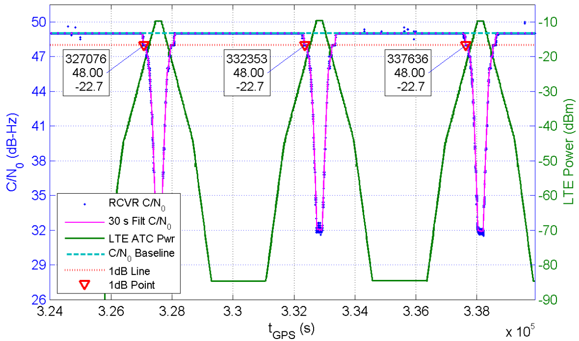
Receiver 109 Average C/N_0 for All Channels and LTE ATC Power at Receiver for TE10
