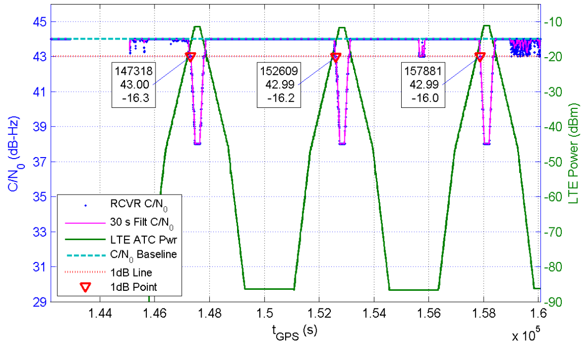
Receiver 386 Average C/N_0 for All Channels and LTE ATC Power at Receiver for TE1
