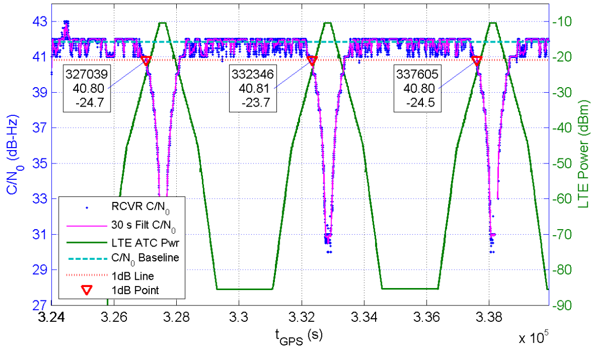
Receiver 100 Average C/N_0 for All Channels and LTE ATC Power at Receiver for TE10
