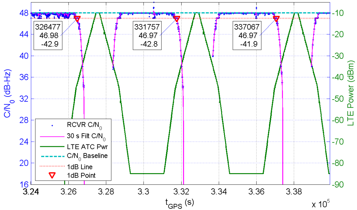
Receiver 367 Average C/N_0 for All Channels and LTE ATC Power at Receiver for TE10
