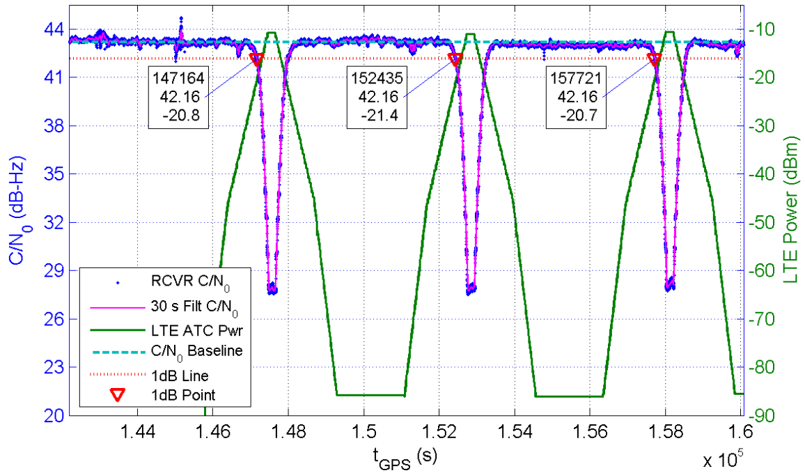
Receiver 342 Average C/N_0 for All Channels and LTE ATC Power at Receiver for TE1
