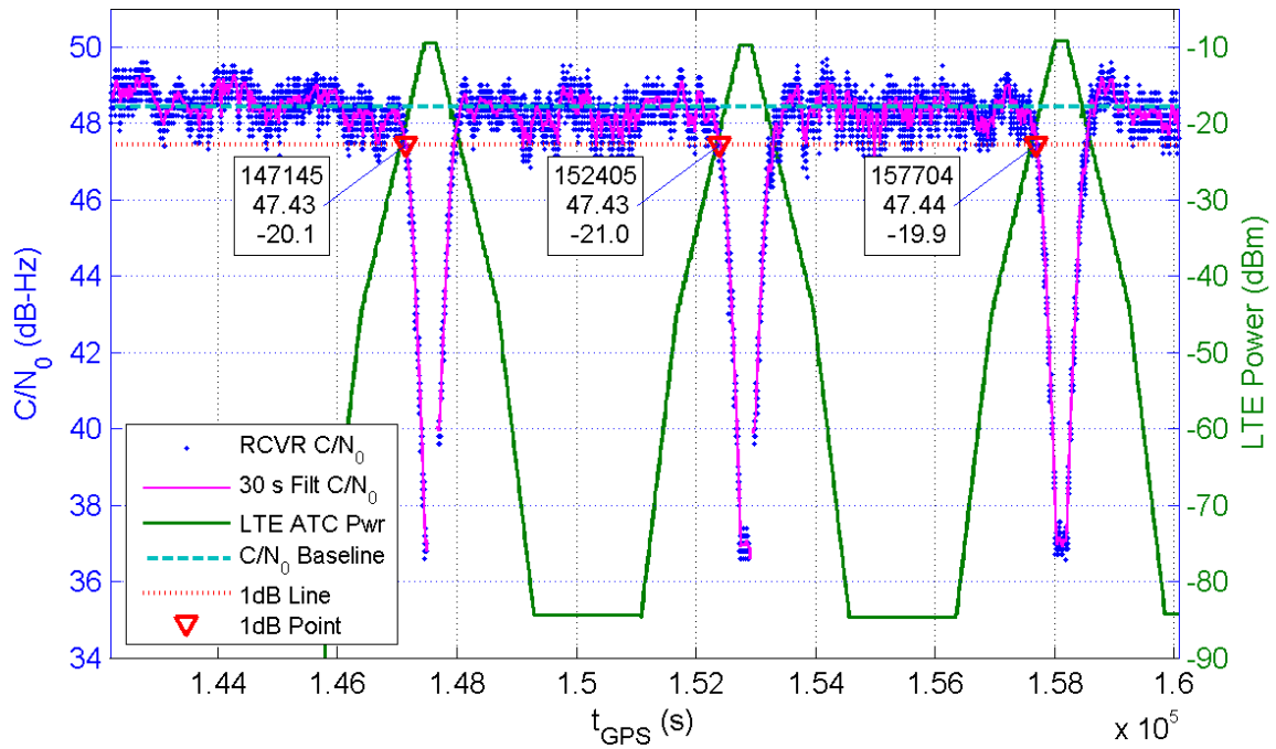
Receiver 123 Average C/N_0 for All Channels and LTE ATC Power at Receiver for TE1
