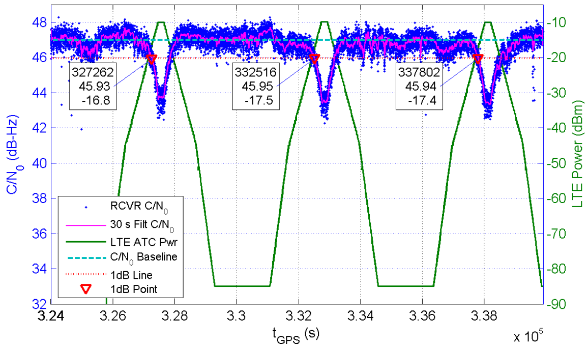
Receiver 120 Average C/N_0 for All Channels and LTE ATC Power at Receiver for TE10
