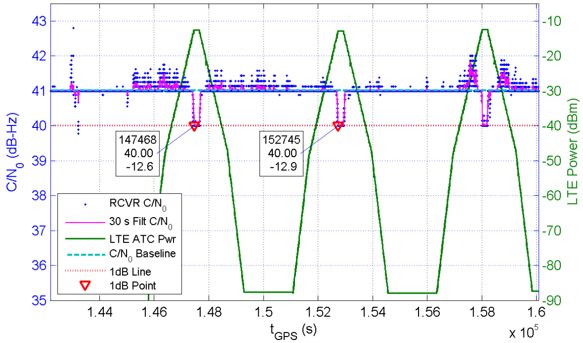
Receiver 133 Average C/N_0 for All Channels and LTE ATC Power at Receiver for TE1
