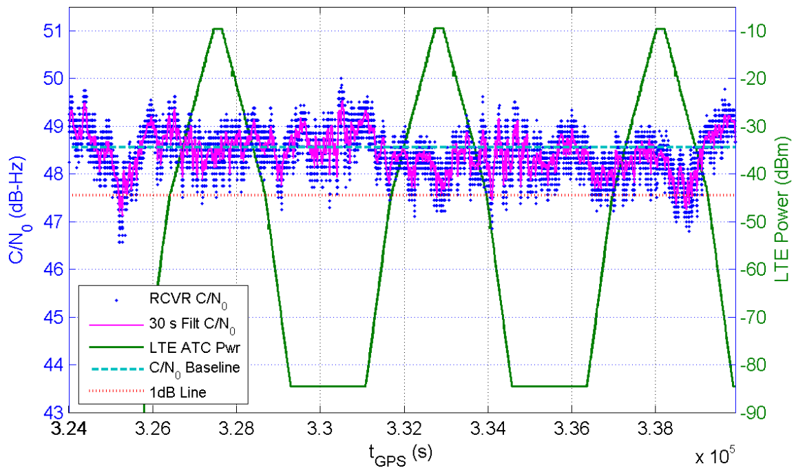
Receiver 351 Average C/N_0 for All Channels and LTE ATC Power at Receiver for TE10
