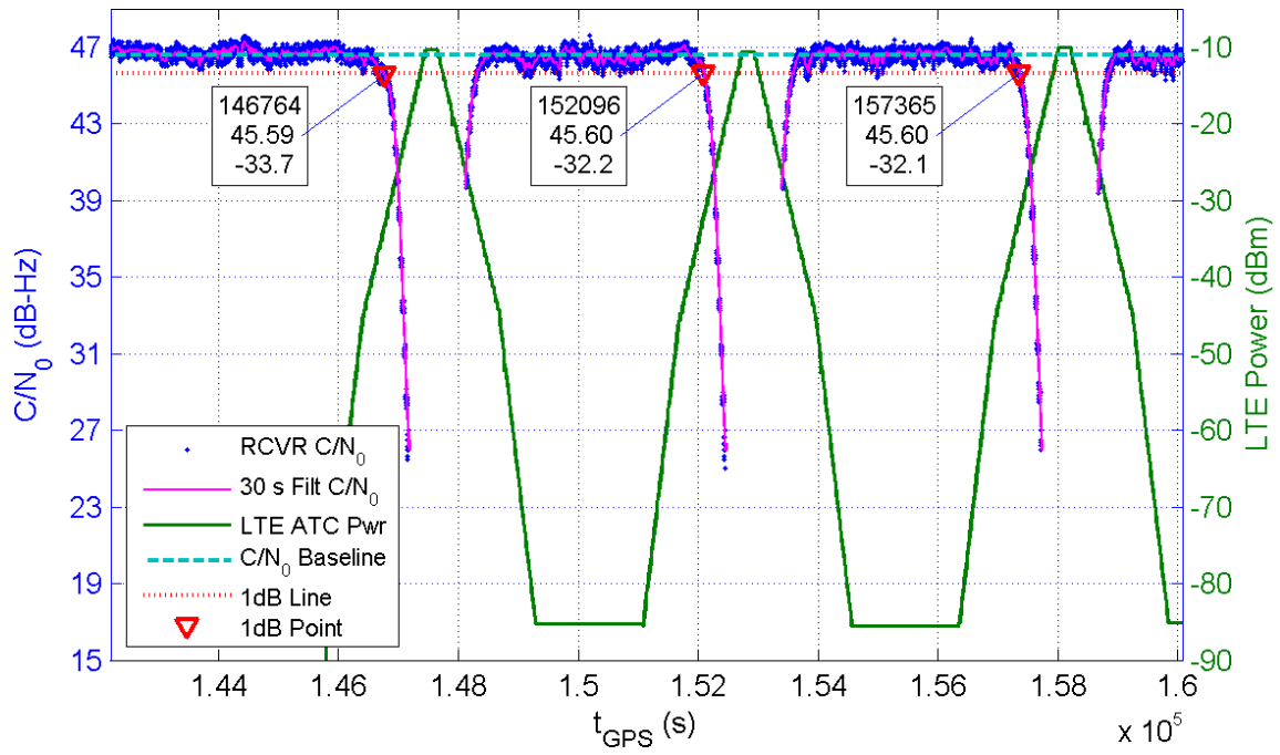
Receiver 359 Average C/N_0 for All Channels and LTE ATC Power at Receiver for TE1
