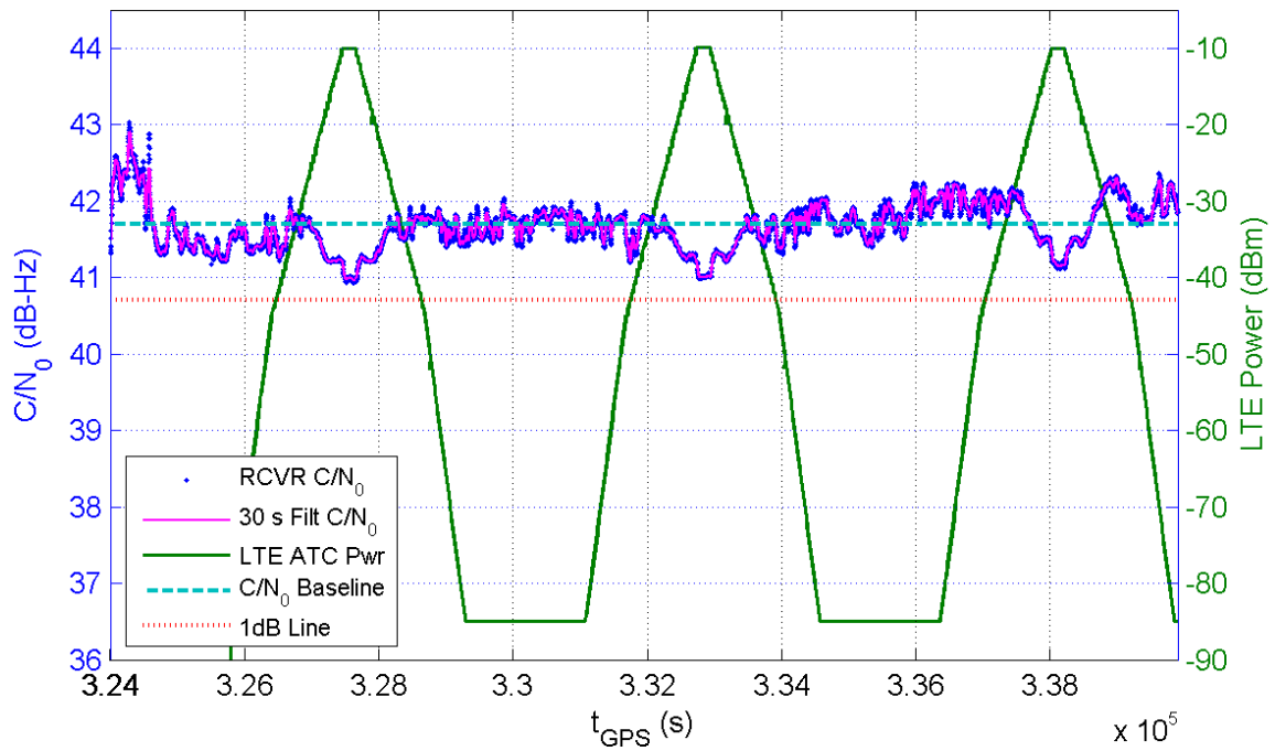
Receiver 214 Average C/N_0 for All Channels and LTE ATC Power at Receiver for TE10
