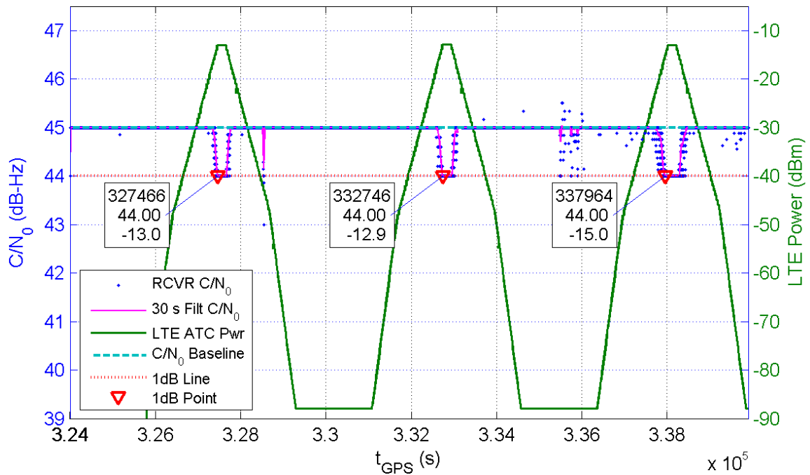
Receiver 212 Average C/N_0 for All Channels and LTE ATC Power at Receiver for TE10
