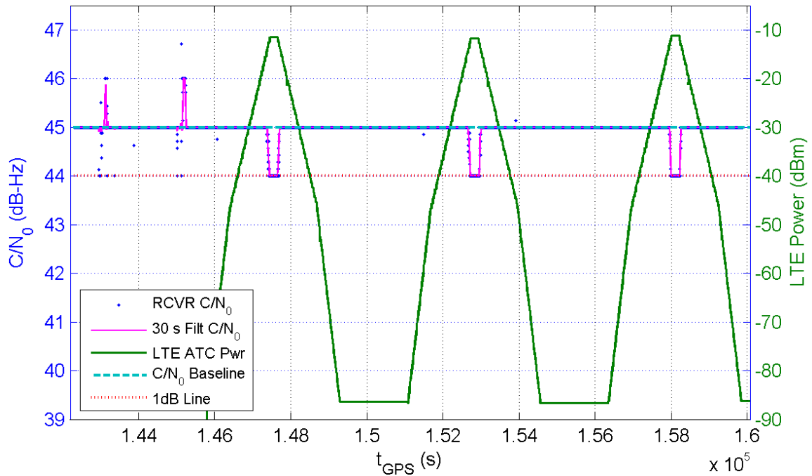
Receiver 319 Average C/N_0 for All Channels and LTE ATC Power at Receiver for TE1
