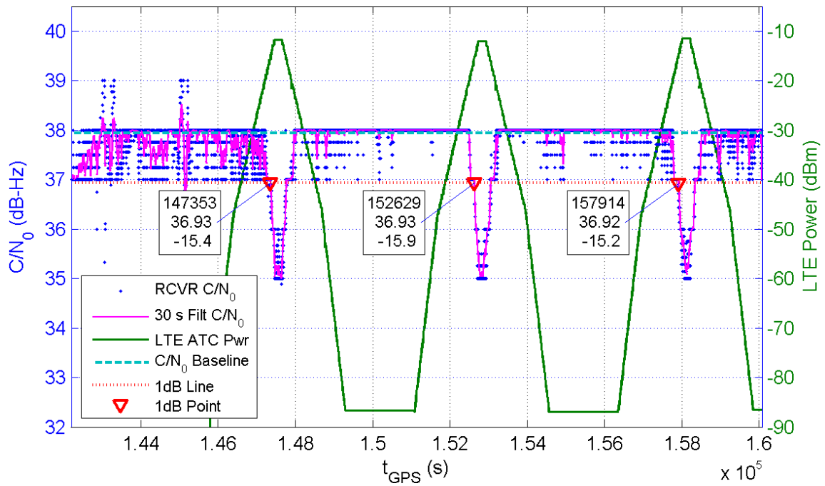
Receiver 383 Average C/N_0 for All Channels and LTE ATC Power at Receiver for TE1
