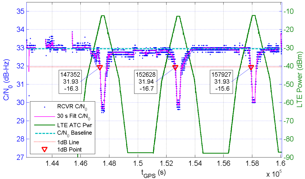
Receiver 204 Average C/N_0 for All Channels and LTE ATC Power at Receiver for TE1
