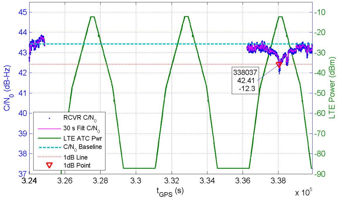
Receiver 310 Average C/N_0 for All Channels and LTE ATC Power at Receiver for TE10
