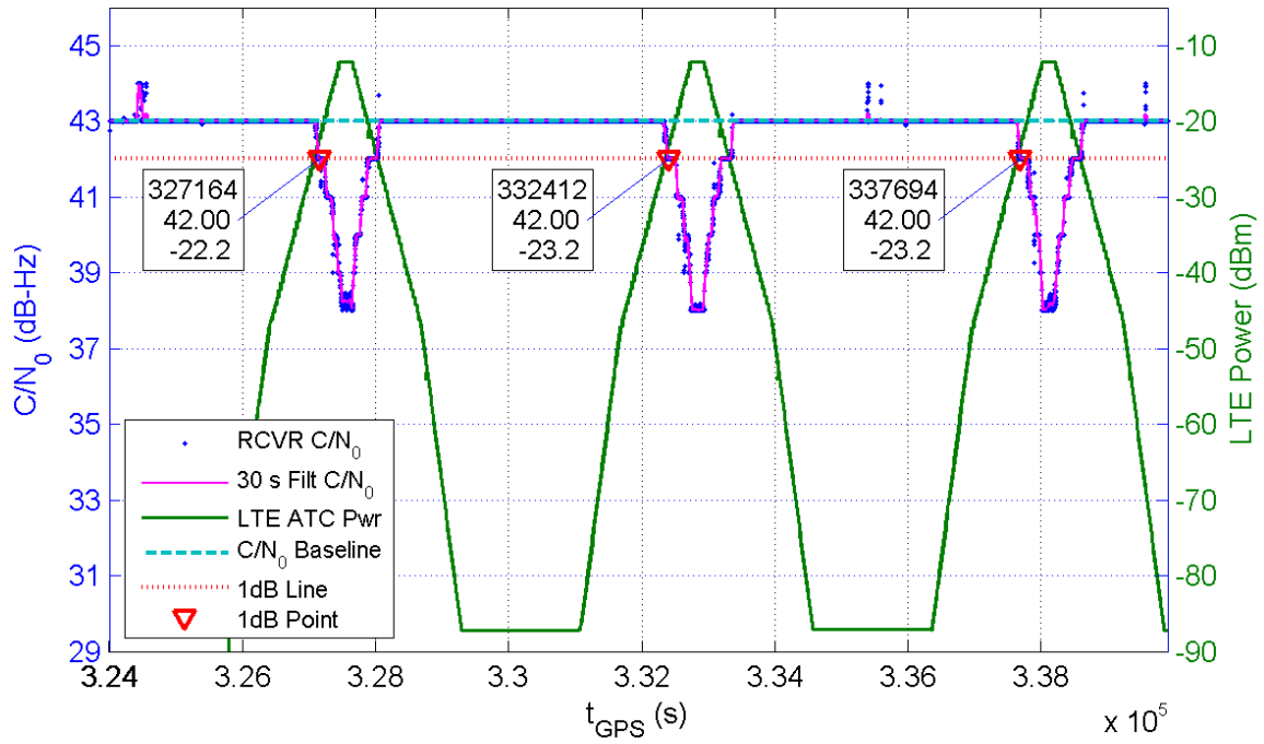
Receiver 105 Average C/N_0 for All Channels and LTE ATC Power at Receiver for TE10
