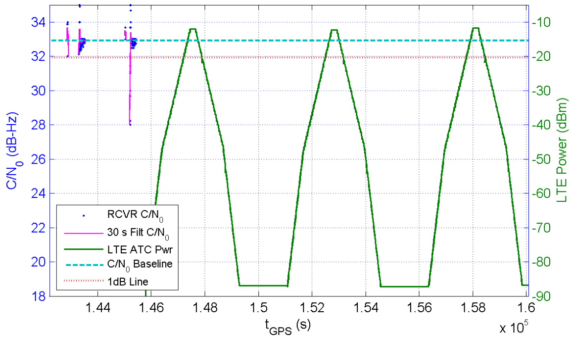
Receiver 315 Average C/N_0 for All Channels and LTE ATC Power at Receiver for TE1
