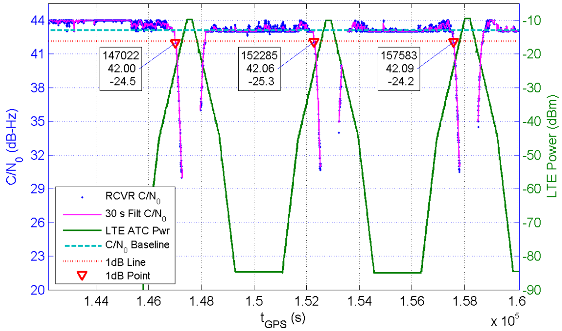
Receiver 358 Average C/N_0 for All Channels and LTE ATC Power at Receiver for TE1
