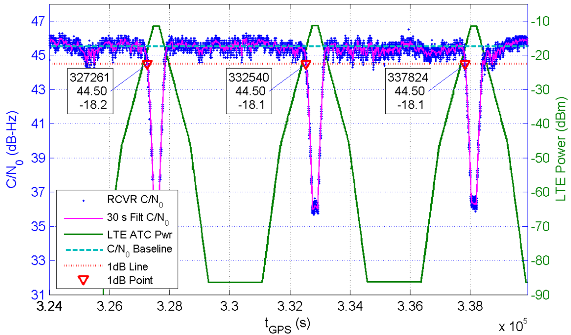
Receiver 396 Average C/N_0 for All Channels and LTE ATC Power at Receiver for TE10
