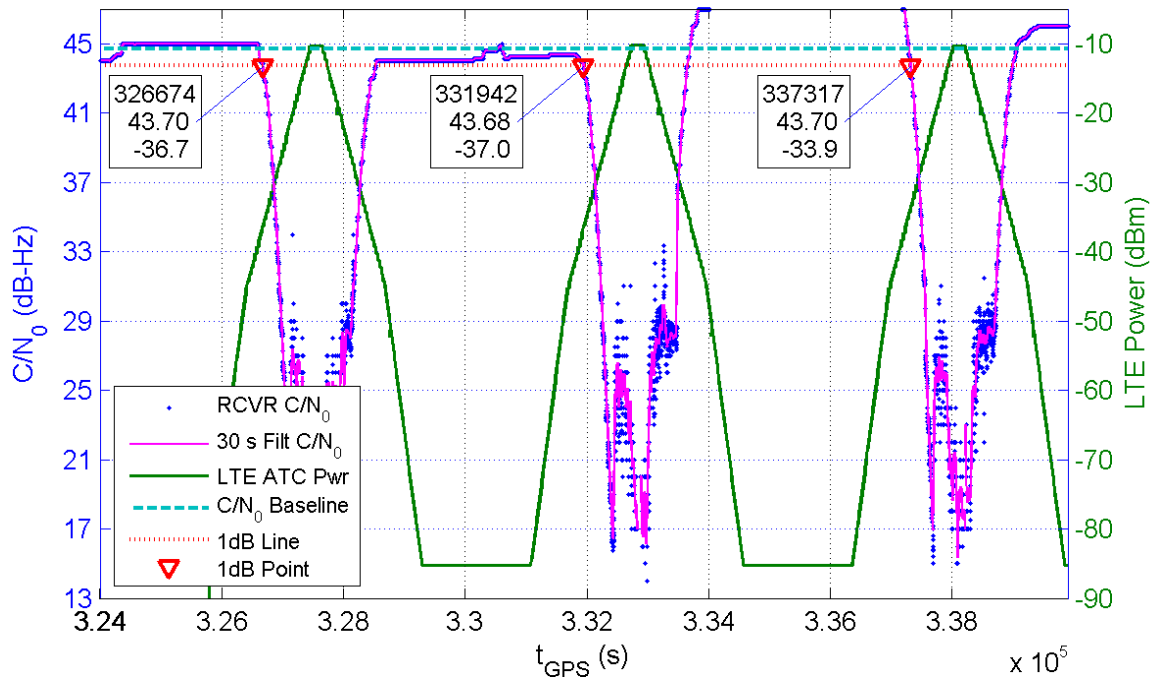
Receiver 206 Average C/N_0 for All Channels and LTE ATC Power at Receiver for TE10
