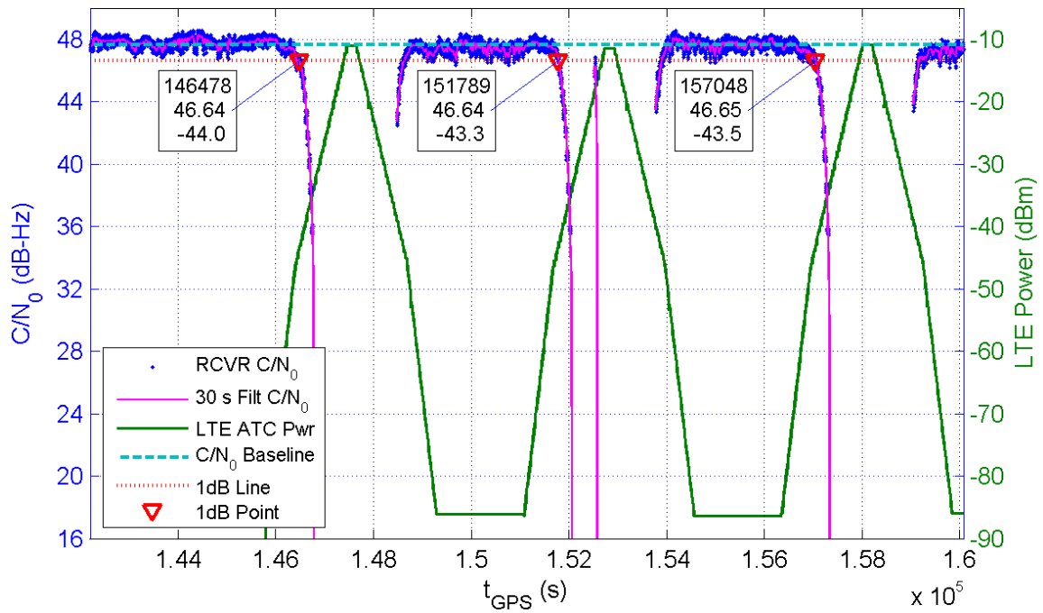
Receiver 117 Average C/N_0 for All Channels and LTE ATC Power at Receiver for TE1
