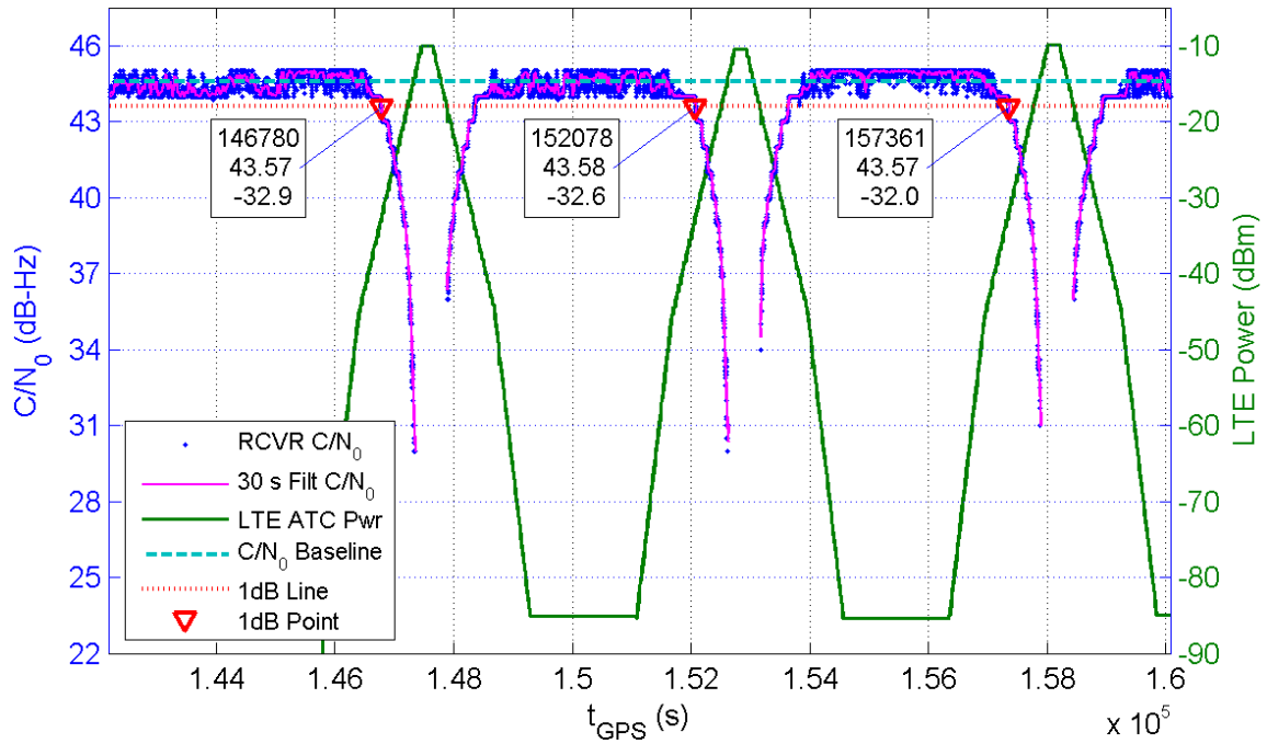
Receiver 313 Average C/N_0 for All Channels and LTE ATC Power at Receiver for TE1
