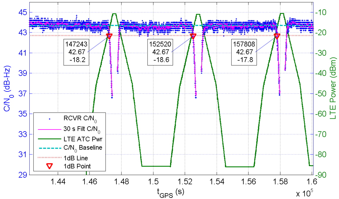
Receiver 390 Average C/N_0 for All Channels and LTE ATC Power at Receiver for TE1
