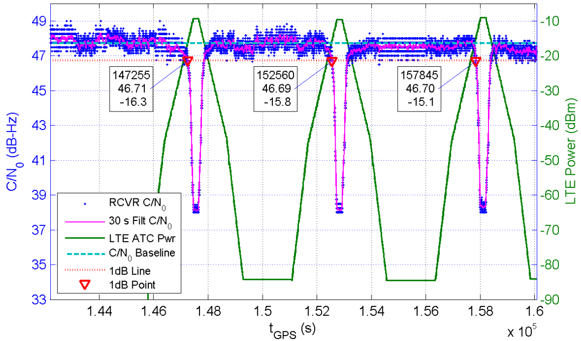
Receiver 356 Average C/N_0 for All Channels and LTE ATC Power at Receiver for TE1
