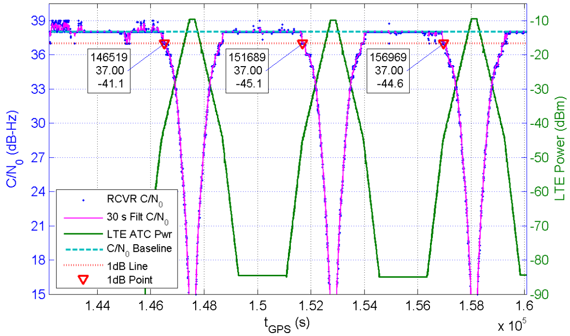
Receiver 347 Average C/N_0 for All Channels and LTE ATC Power at Receiver for TE1
