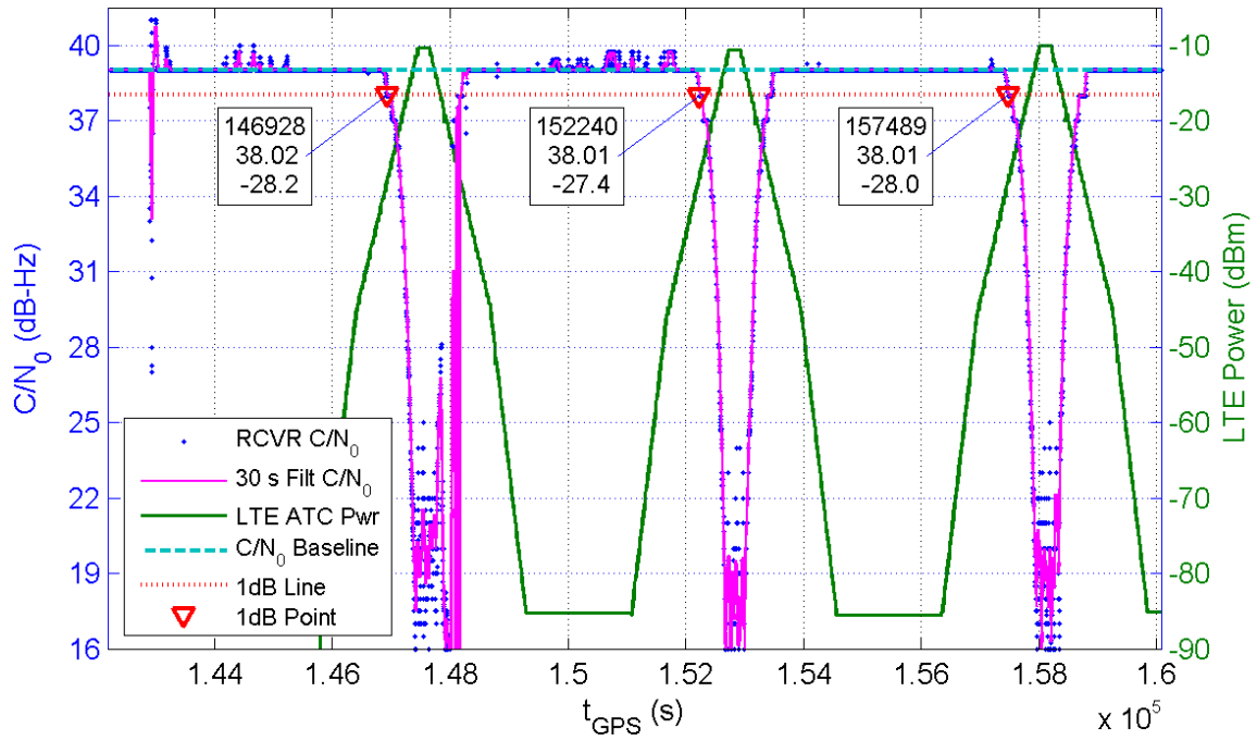
Receiver 208 Average C/N_0 for All Channels and LTE ATC Power at Receiver for TE1
