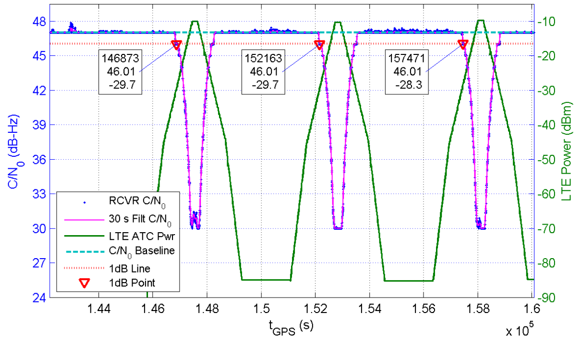
Receiver 248 Average C/N_0 for All Channels and LTE ATC Power at Receiver for TE1
