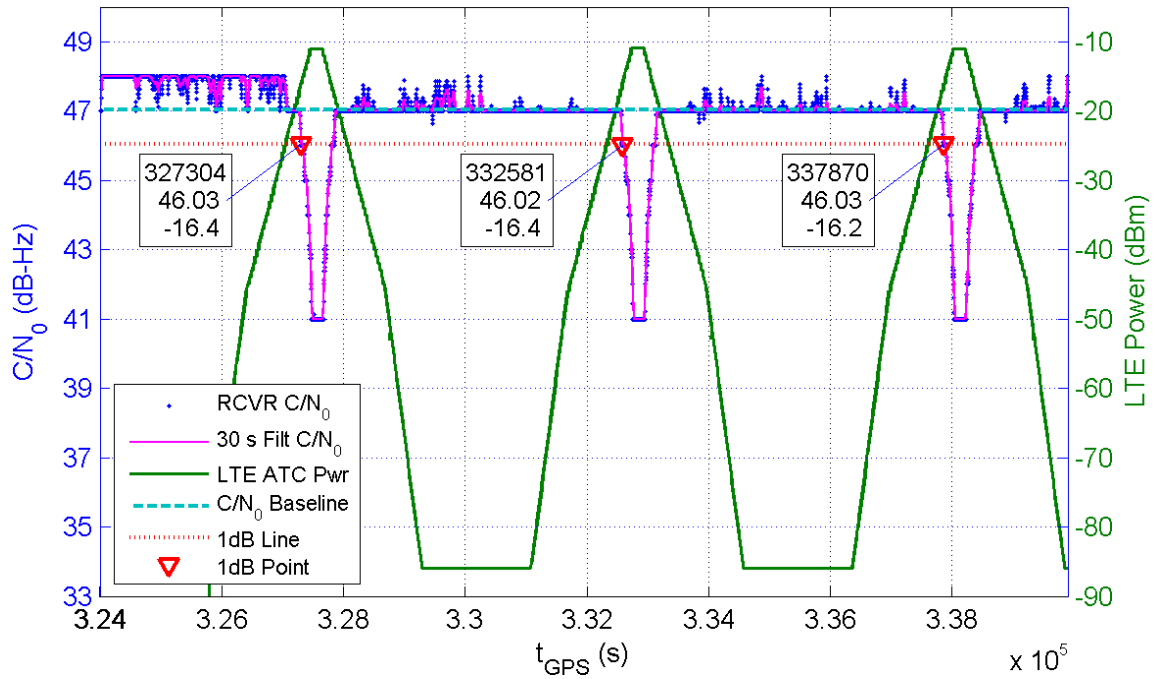
Receiver 375 Average C/N_0 for All Channels and LTE ATC Power at Receiver for TE10
