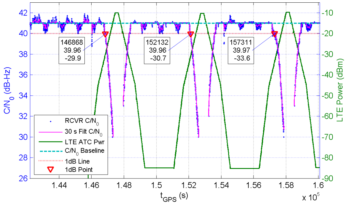
Receiver 393 Average C/N_0 for All Channels and LTE ATC Power at Receiver for TE1
