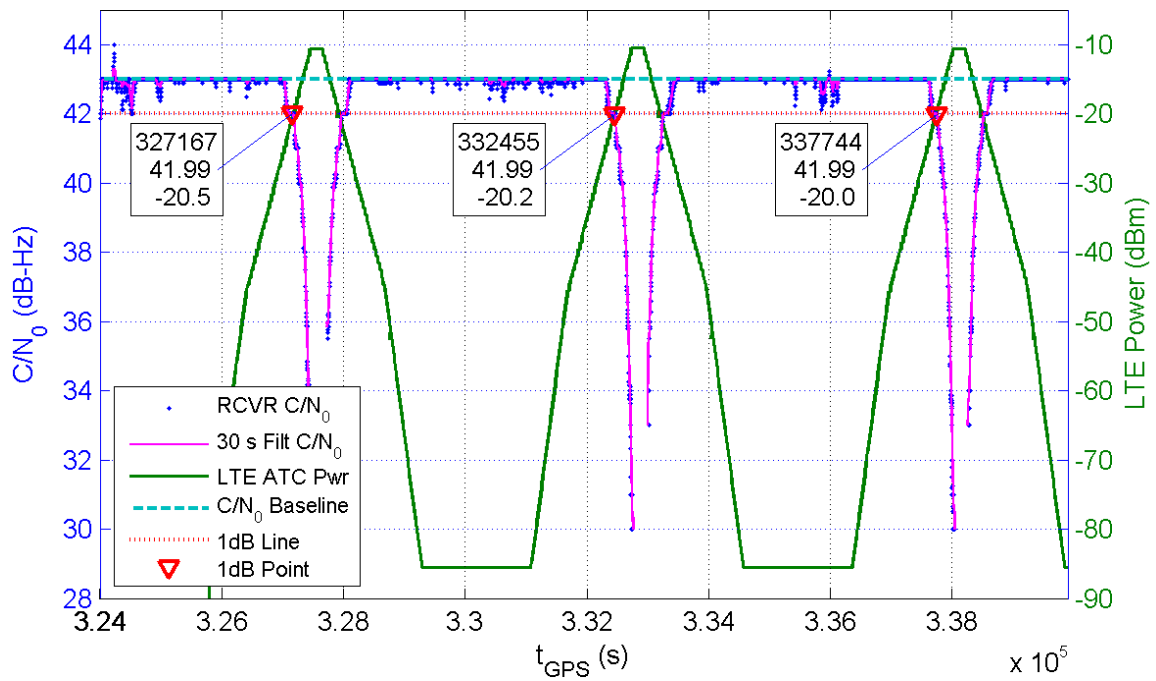
Receiver 354 Average C/N_0 for All Channels and LTE ATC Power at Receiver for TE10
