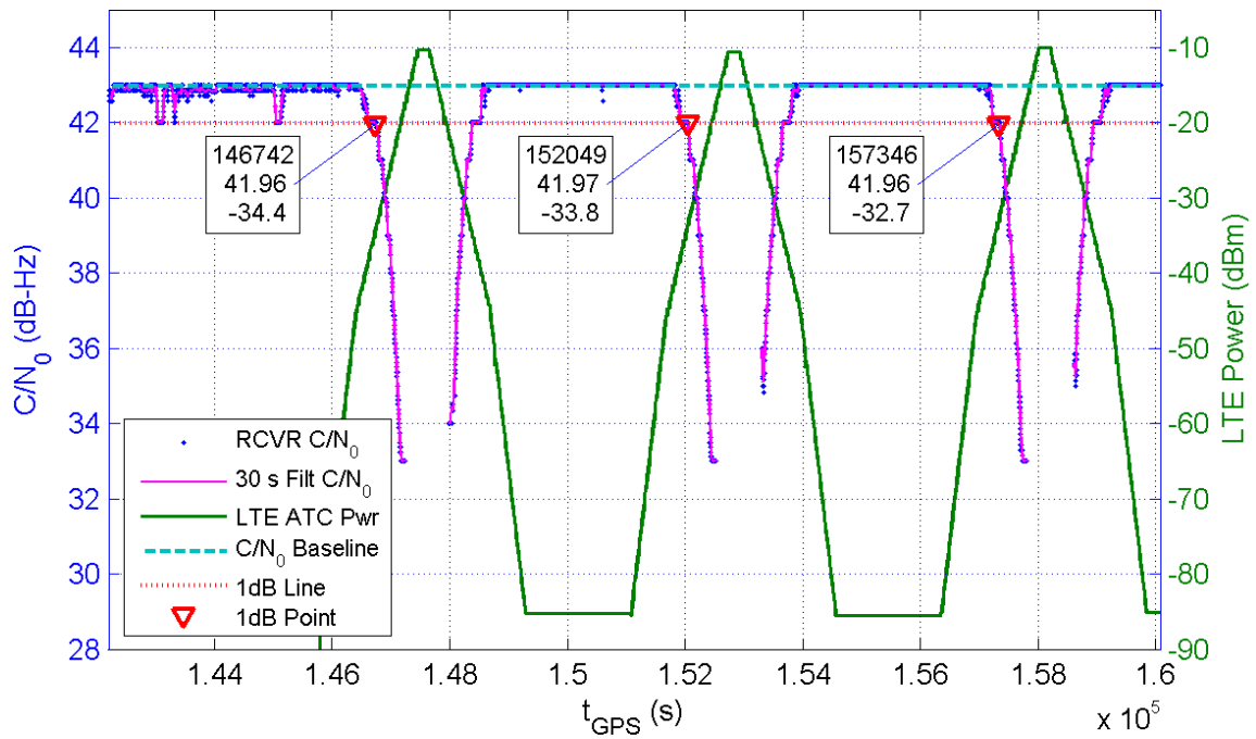
Receiver 125 Average C/N_0 for All Channels and LTE ATC Power at Receiver for TE1
