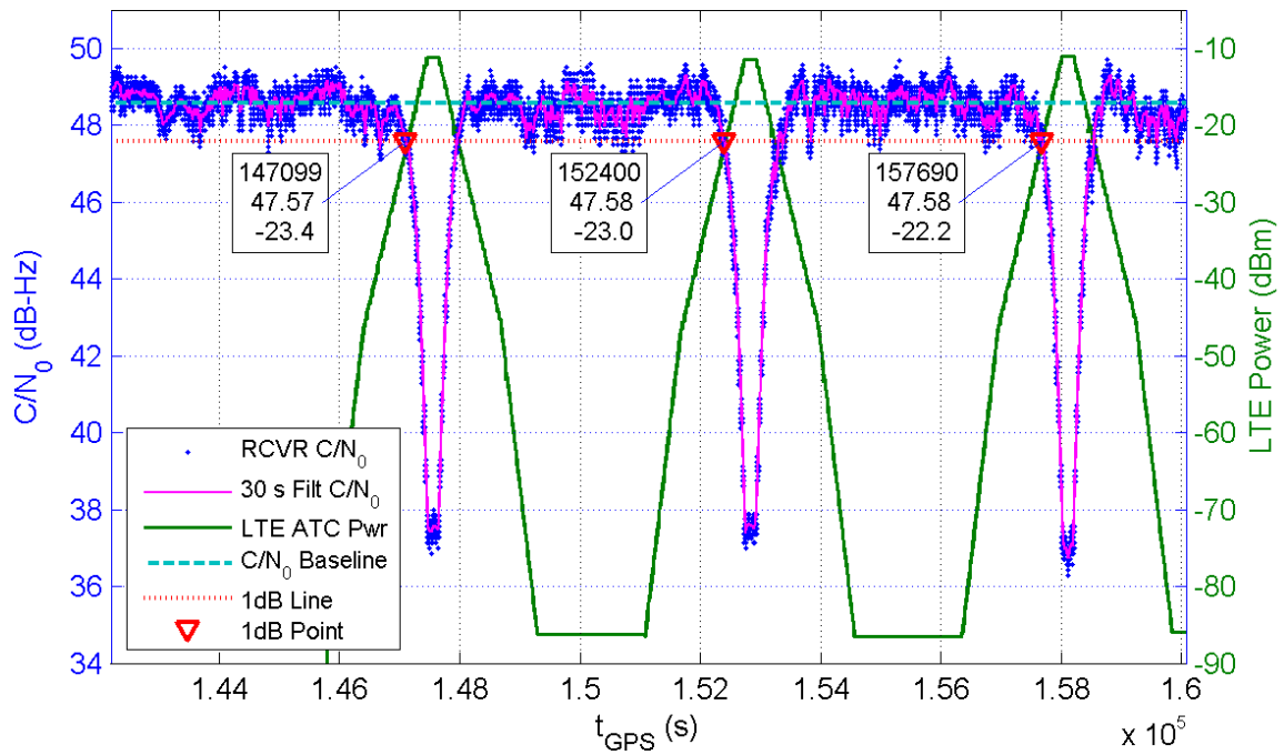
Receiver 346 Average C/N_0 for All Channels and LTE ATC Power at Receiver for TE1
