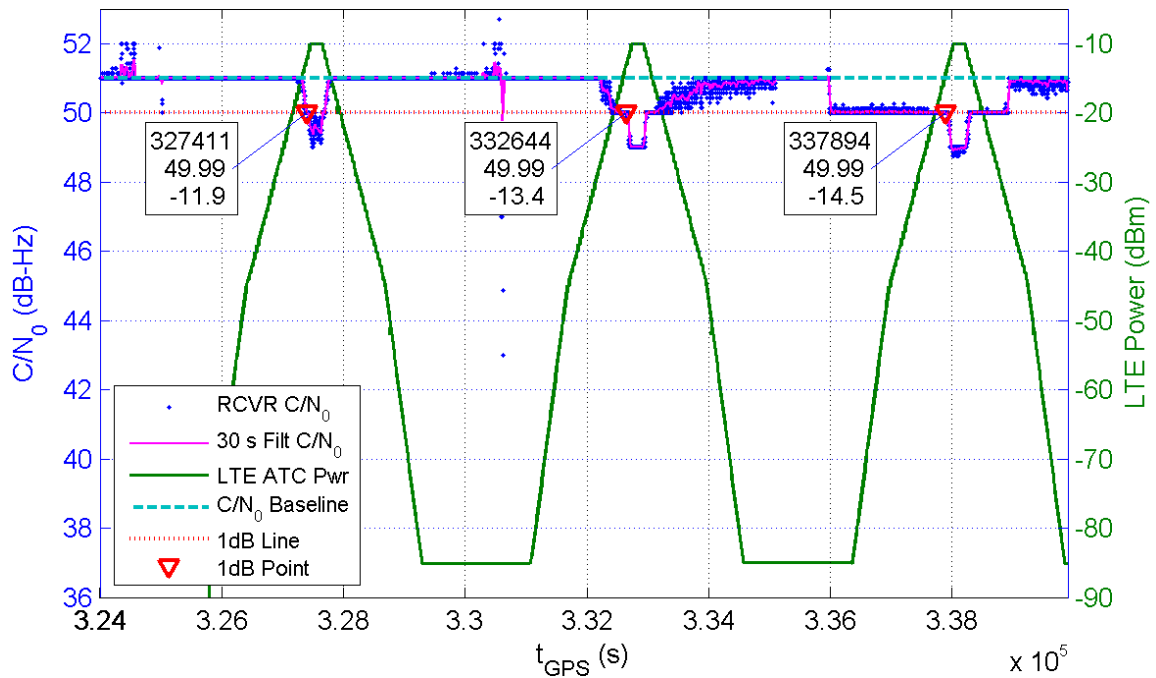
Receiver 108 Average C/N_0 for All Channels and LTE ATC Power at Receiver for TE10
