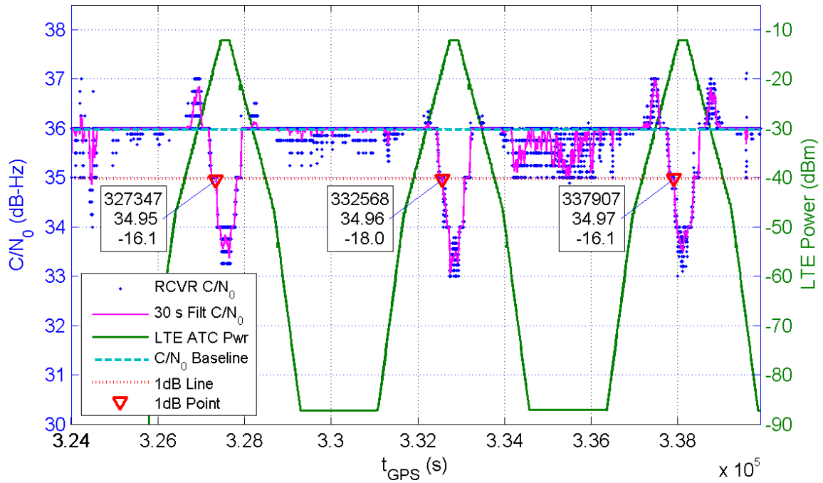
Receiver 307 Average C/N_0 for All Channels and LTE ATC Power at Receiver for TE10
