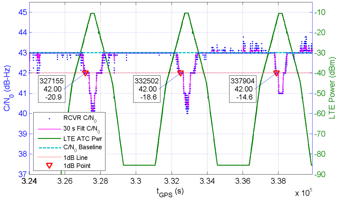
Receiver 397 Average C/N_0 for All Channels and LTE ATC Power at Receiver for TE10
