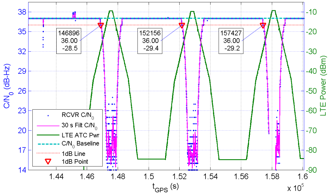
Receiver 320 Average C/N_0 for All Channels and LTE ATC Power at Receiver for TE1
