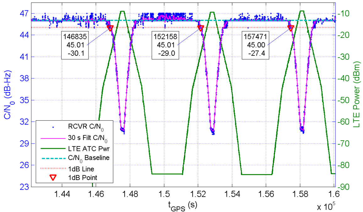
Receiver 373 Average C/N_0 for All Channels and LTE ATC Power at Receiver for TE1
