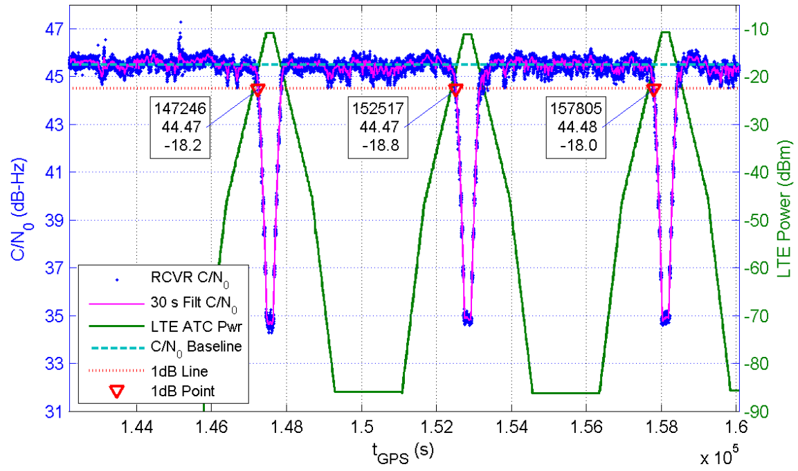
Receiver 396 Average C/N_0 for All Channels and LTE ATC Power at Receiver for TE1
