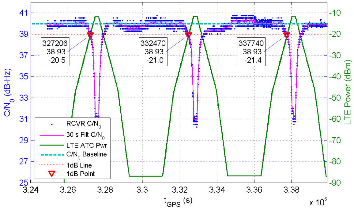
Receiver 301 Average C/N_0 for All Channels and LTE ATC Power at Receiver for TE10
