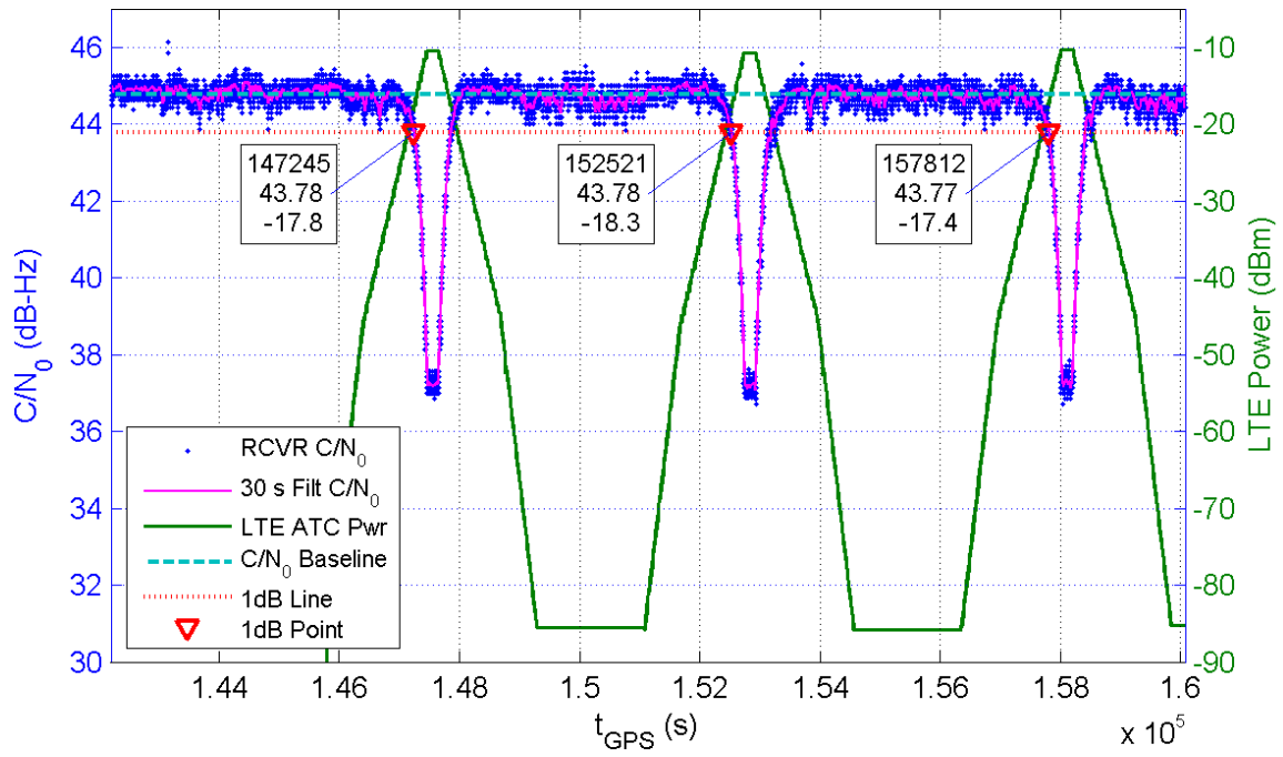
Receiver 364 Average C/N_0 for All Channels and LTE ATC Power at Receiver for TE1
