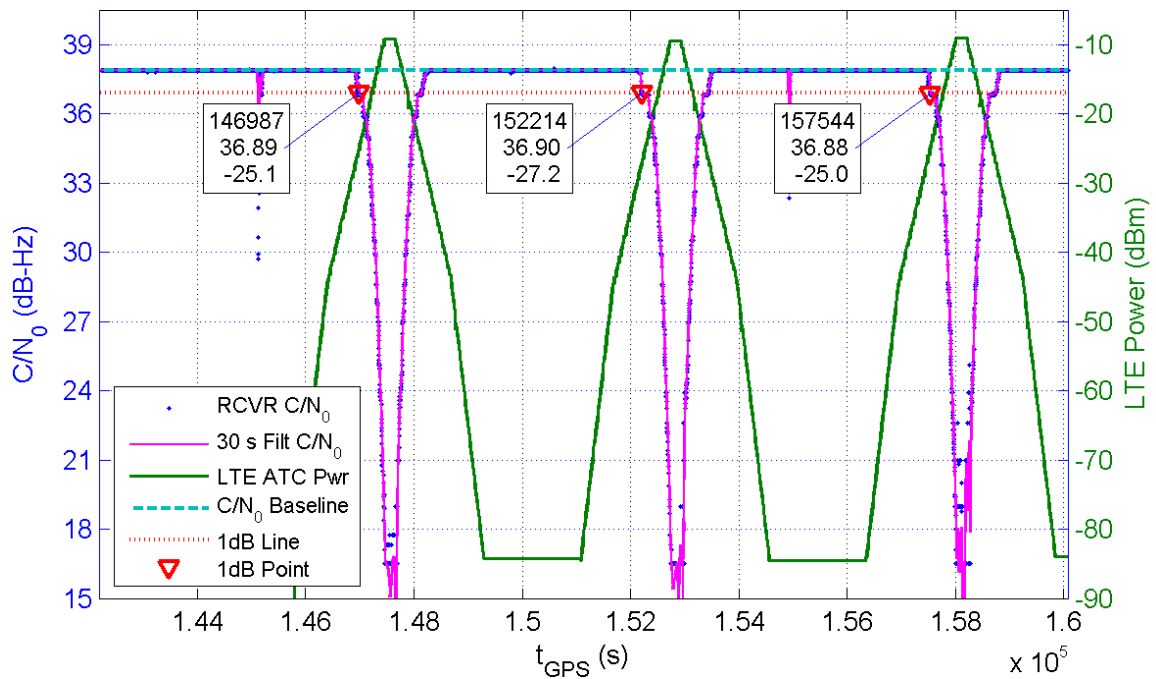
Receiver 388 Average C/N_0 for All Channels and LTE ATC Power at Receiver for TE1
