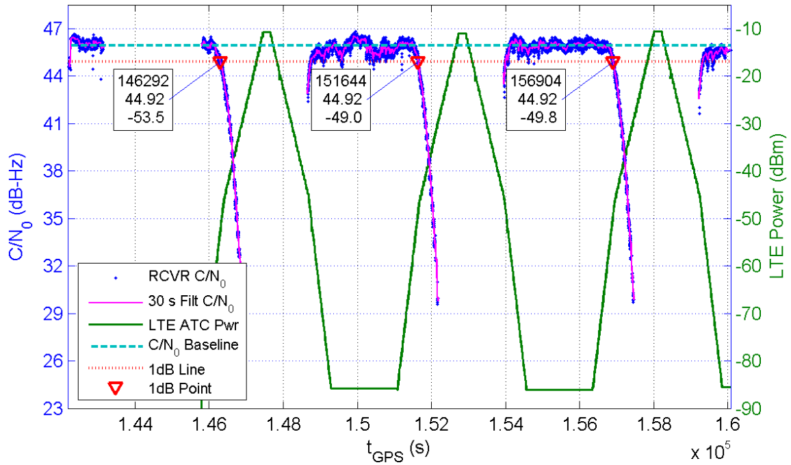
Receiver 350 Average C/N_0 for All Channels and LTE ATC Power at Receiver for TE1
