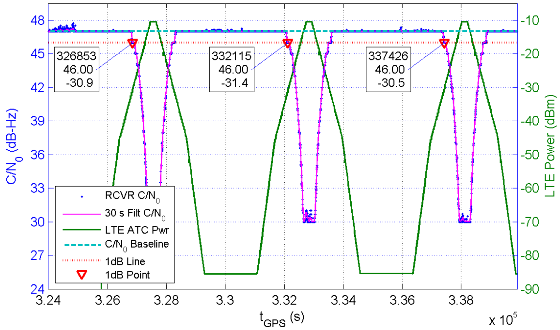
Receiver 248 Average C/N_0 for All Channels and LTE ATC Power at Receiver for TE10
