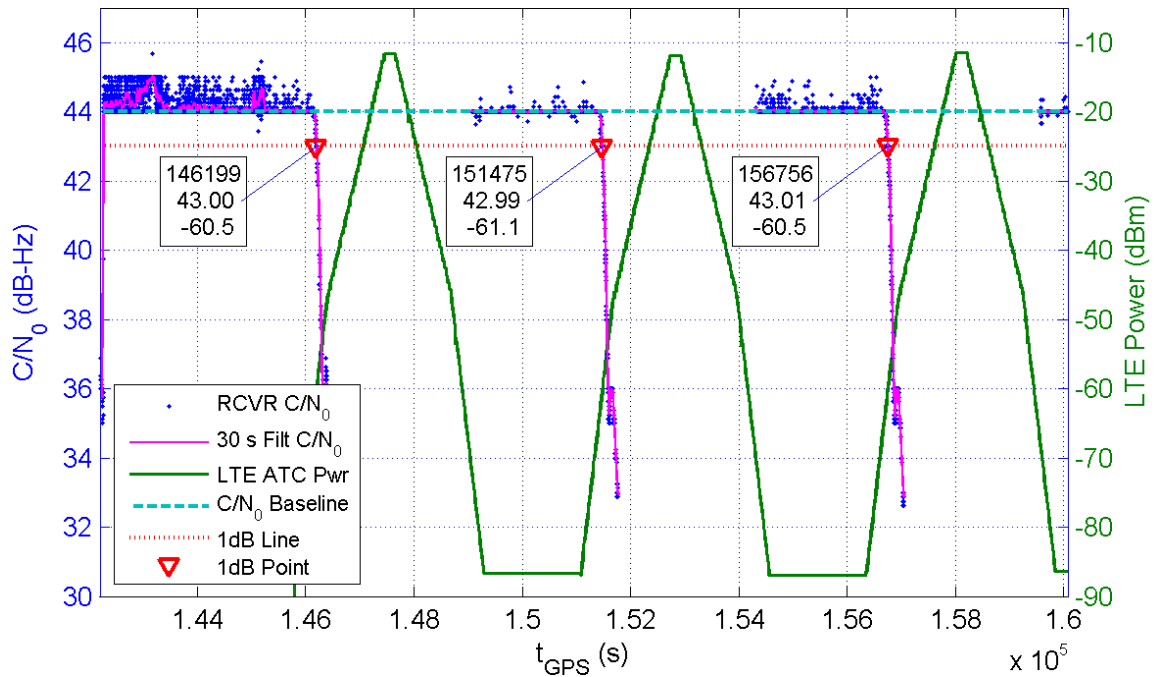
Receiver 357 Average C/N_0 for All Channels and LTE ATC Power at Receiver for TE1
