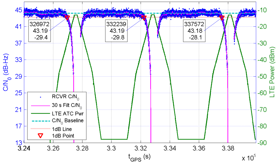
Receiver 235 Average C/N_0 for All Channels and LTE ATC Power at Receiver for TE10
