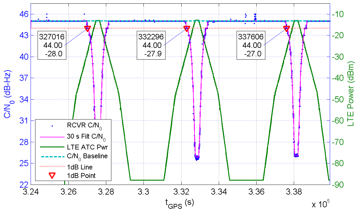
Receiver 112 Average C/N_0 for All Channels and LTE ATC Power at Receiver for TE10
