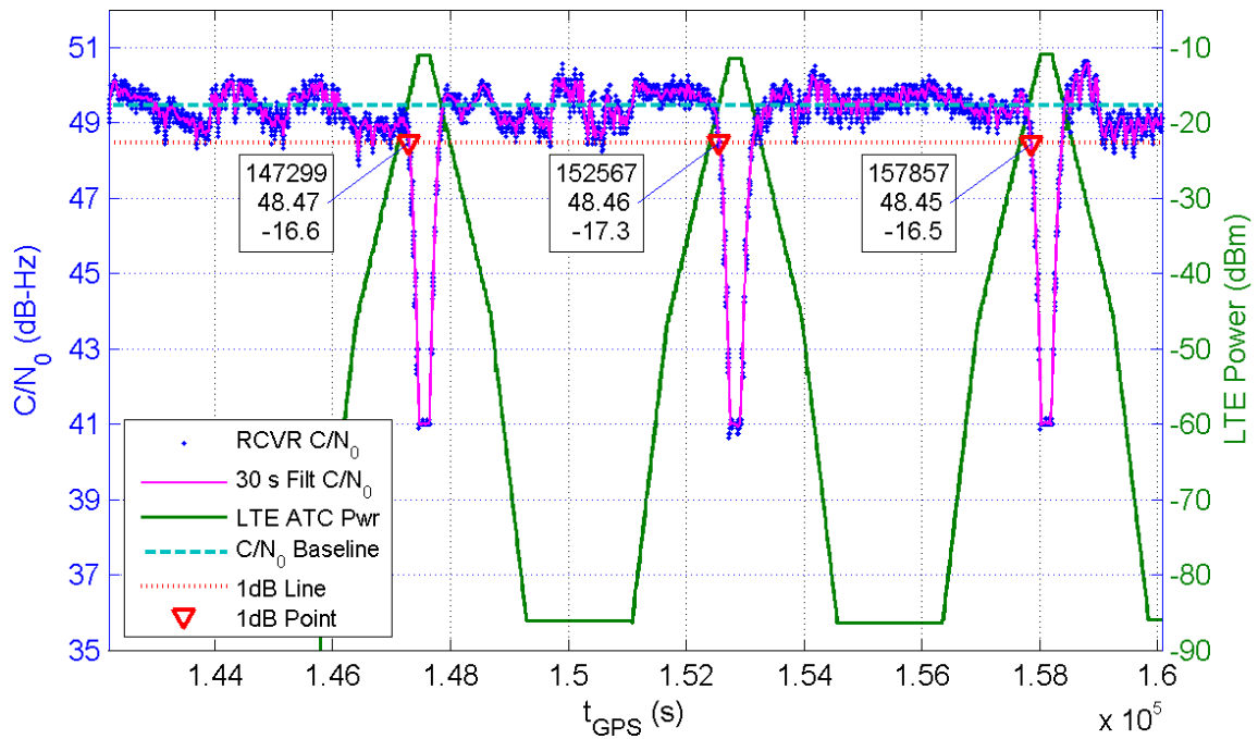
Receiver 329 Average C/N_0 for All Channels and LTE ATC Power at Receiver for TE1
