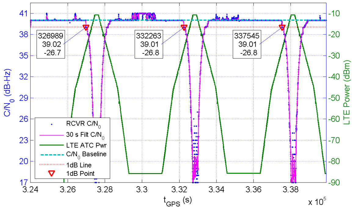
Receiver 208 Average C/N_0 for All Channels and LTE ATC Power at Receiver for TE10
