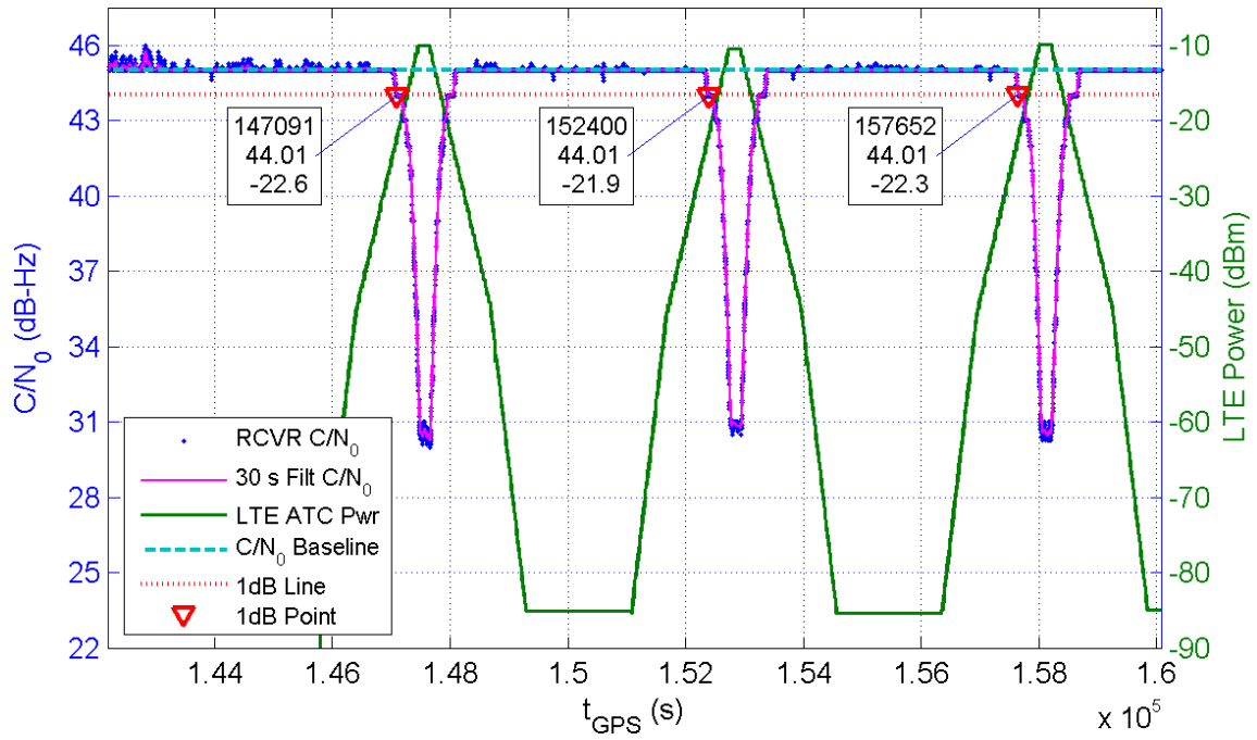
Receiver 389 Average C/N_0 for All Channels and LTE ATC Power at Receiver for TE1
