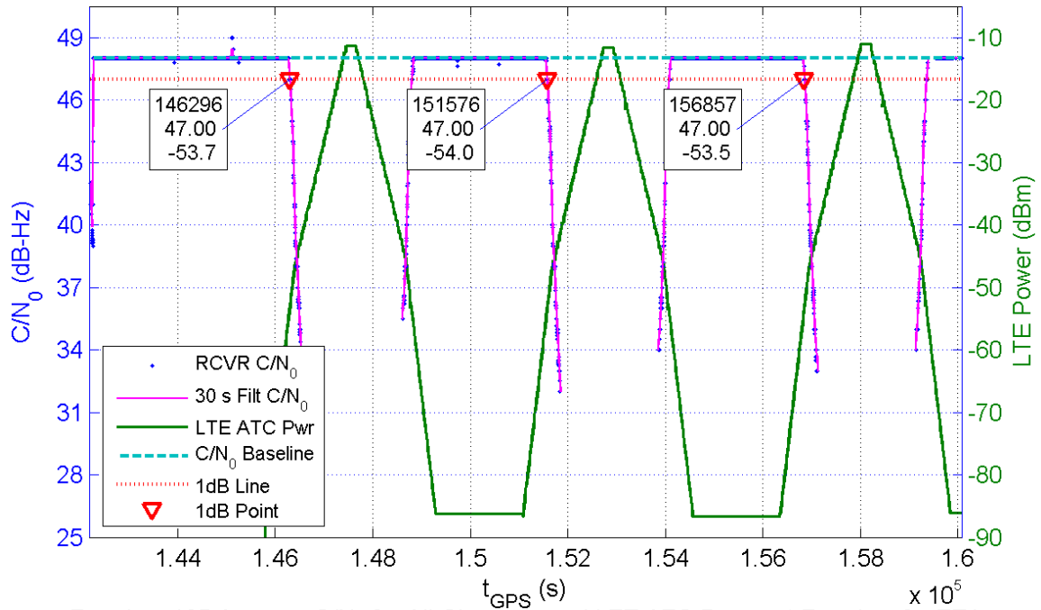
Receiver 105 Average C/N_0 for All Channels and LTE ATC Power at Receiver for TE1
