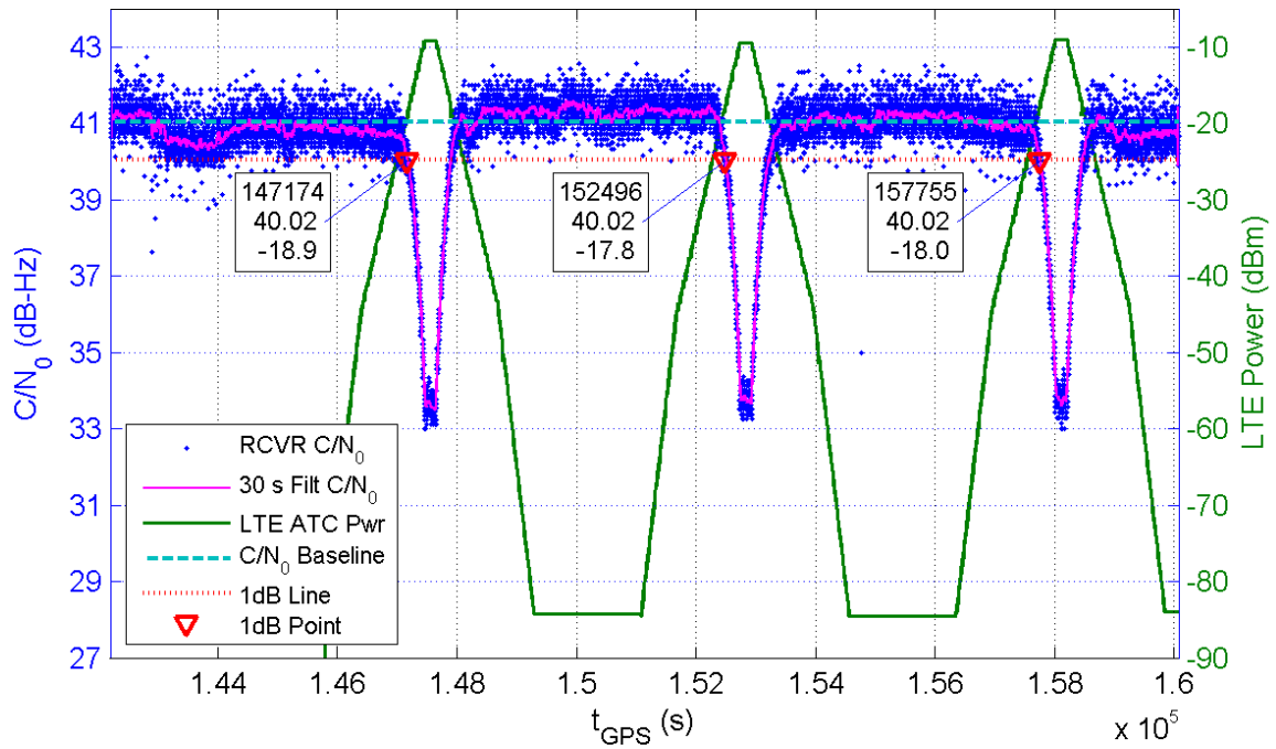
Receiver 324 Average C/N_0 for All Channels and LTE ATC Power at Receiver for TE1
