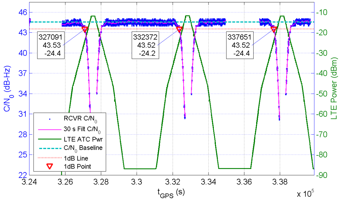
Receiver 317 Average C/N_0 for All Channels and LTE ATC Power at Receiver for TE10
