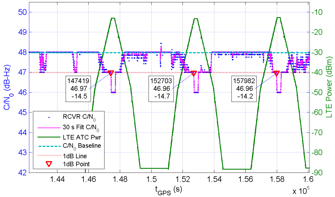
Receiver 369 Average C/N_0 for All Channels and LTE ATC Power at Receiver for TE1
