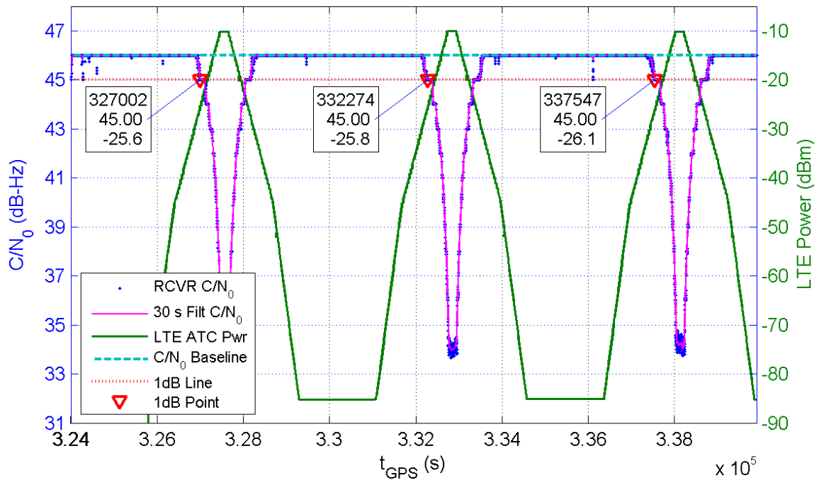
Receiver 218 Average C/N_0 for All Channels and LTE ATC Power at Receiver for TE10
