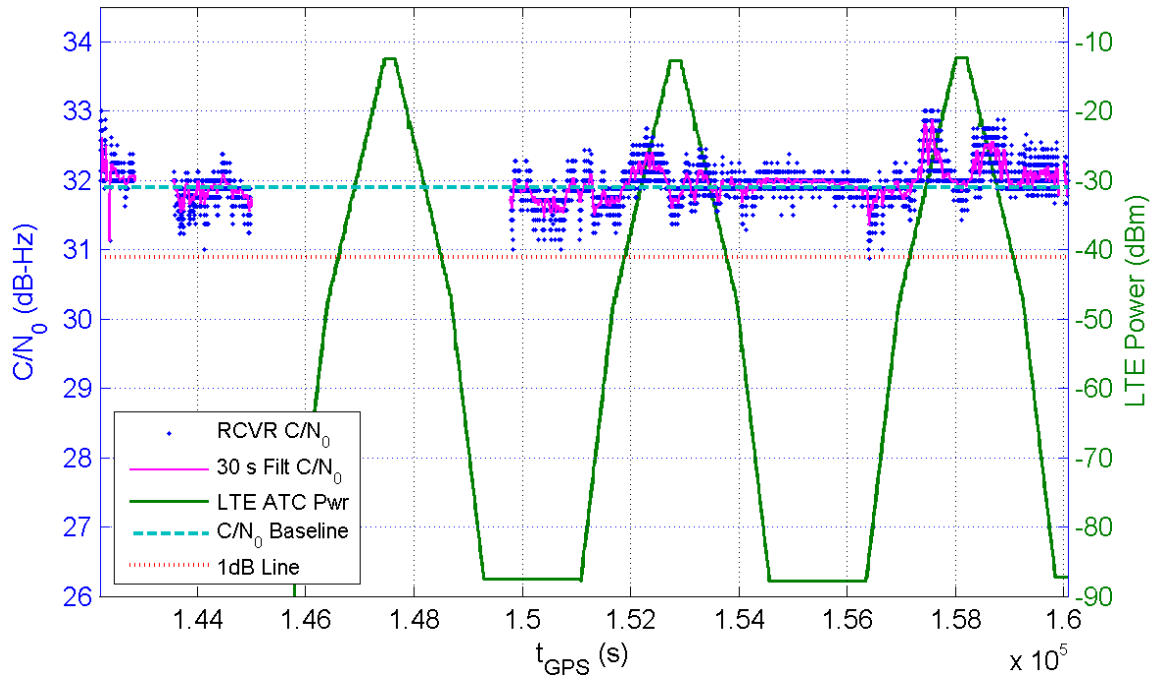
Receiver 322 Average C/N_0 for All Channels and LTE ATC Power at Receiver for TE1
