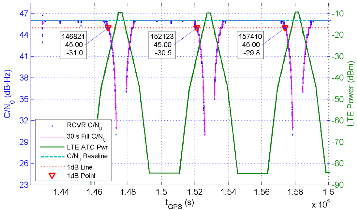
Receiver 332 Average C/N_0 for All Channels and LTE ATC Power at Receiver for TE1
