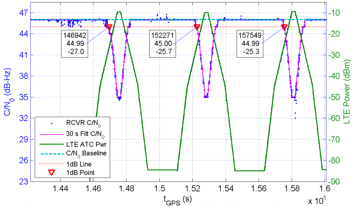
Receiver 334 Average C/N_0 for All Channels and LTE ATC Power at Receiver for TE1
