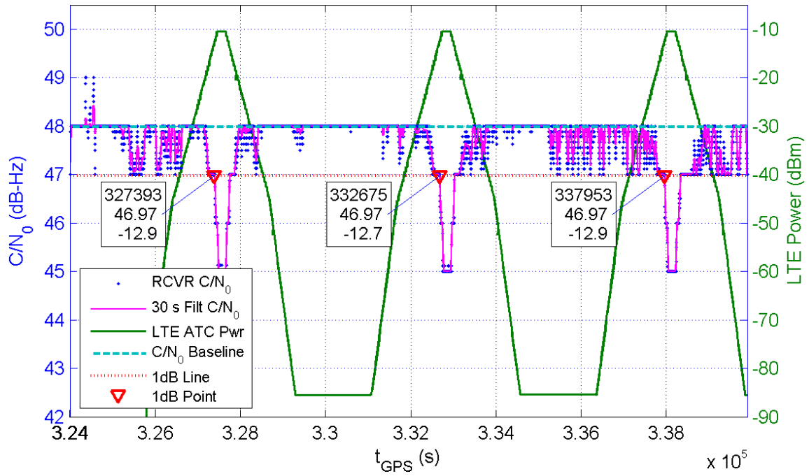
Receiver 119 Average C/N_0 for All Channels and LTE ATC Power at Receiver for TE10
