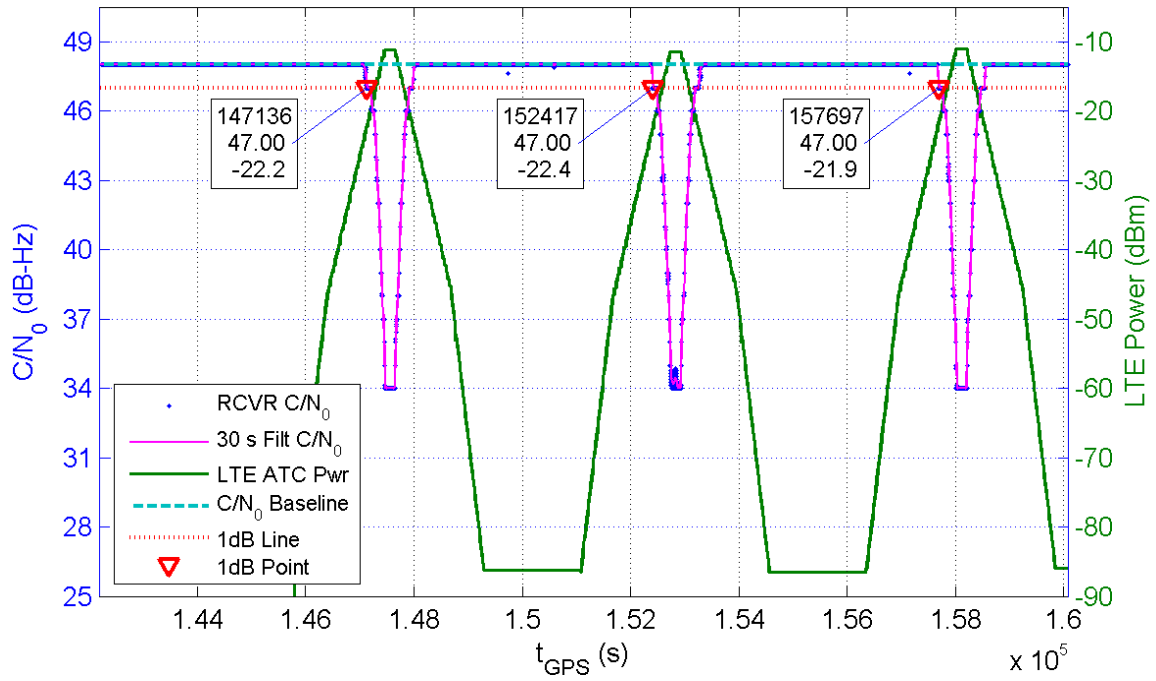
Receiver 116 Average C/N_0 for All Channels and LTE ATC Power at Receiver for TE1
