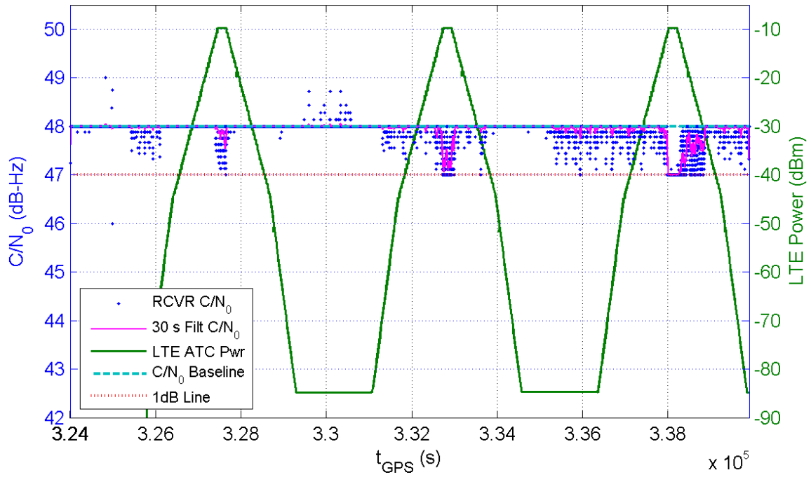
Receiver 113 Average C/N_0 for All Channels and LTE ATC Power at Receiver for TE10
