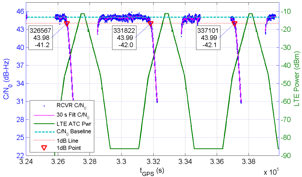
Receiver 104 Average C/N_0 for All Channels and LTE ATC Power at Receiver for TE10
