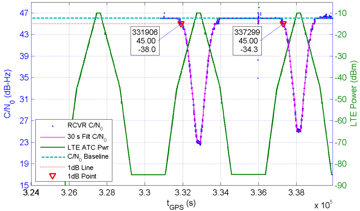
Receiver 115 Average C/N_0 for All Channels and LTE ATC Power at Receiver for TE10
