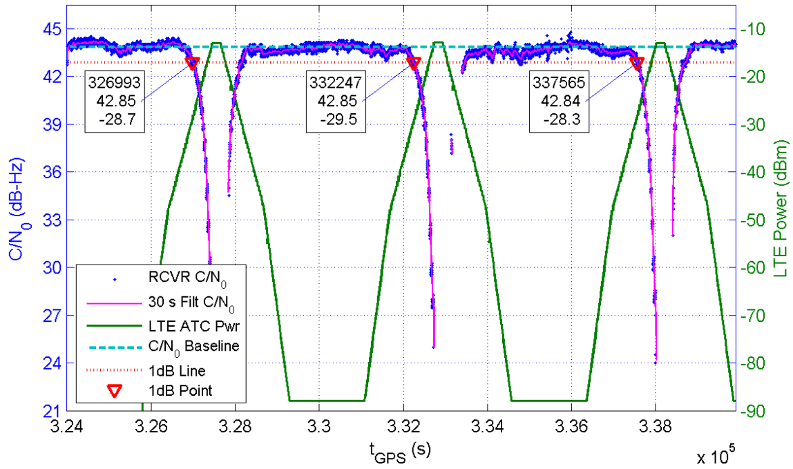
Receiver 394 Average C/N_0 for All Channels and LTE ATC Power at Receiver for TE10
