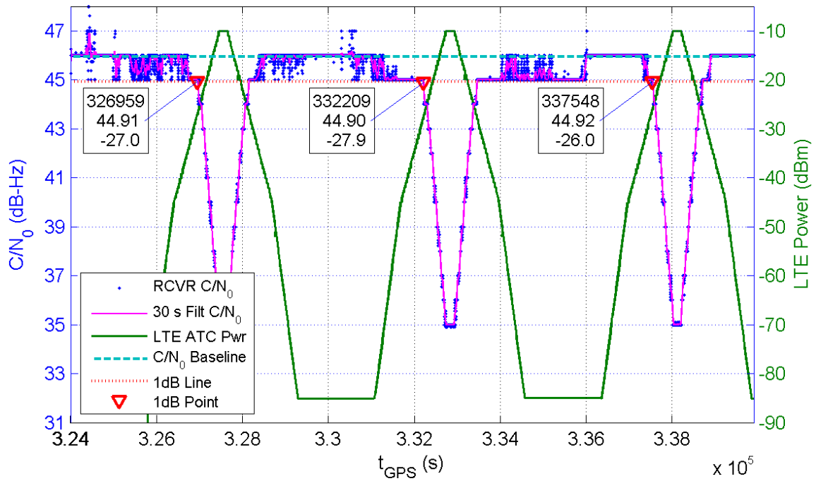
Receiver 362 Average C/N_0 for All Channels and LTE ATC Power at Receiver for TE10
