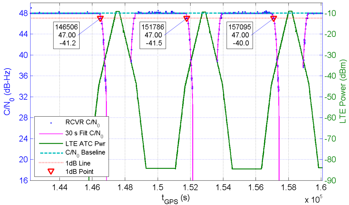
Receiver 382 Average C/N_0 for All Channels and LTE ATC Power at Receiver for TE1
