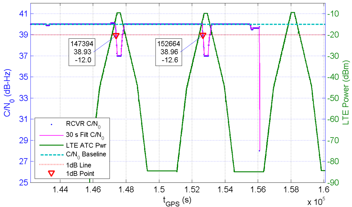
Receiver 128 Average C/N_0 for All Channels and LTE ATC Power at Receiver for TE1
