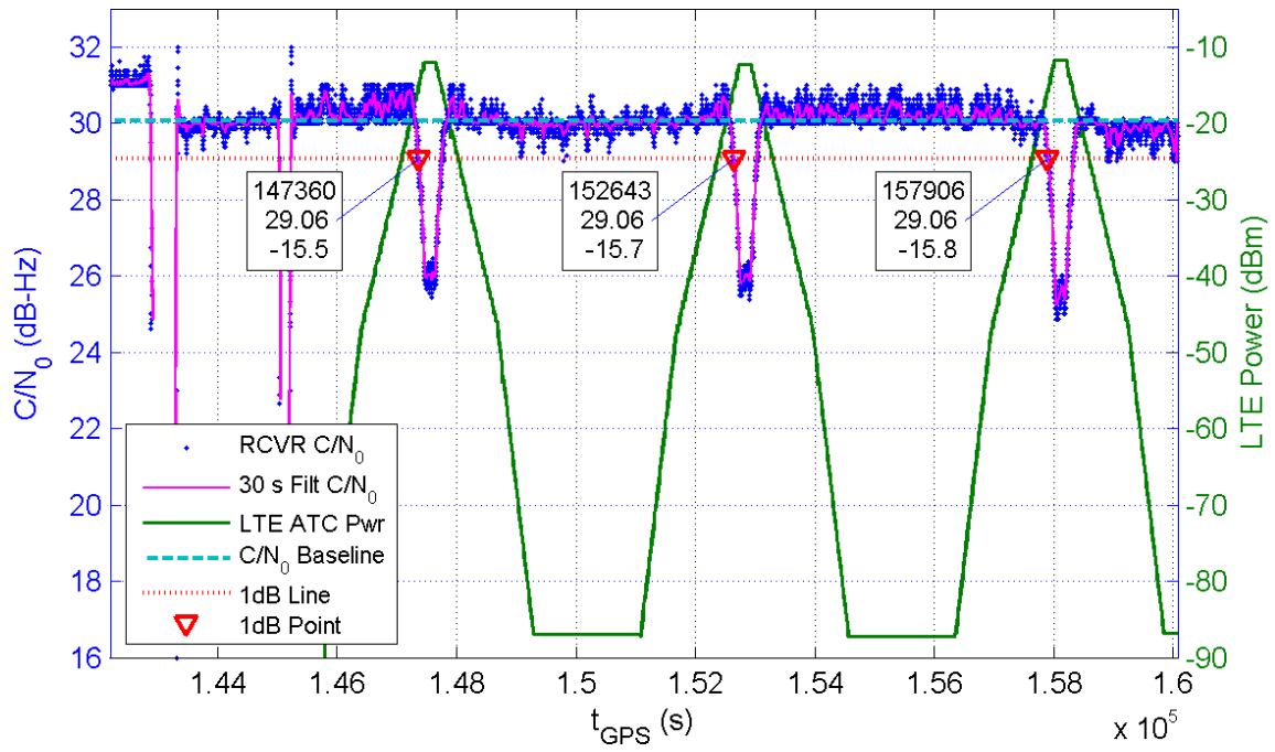
Receiver 377 Average C/N_0 for All Channels and LTE ATC Power at Receiver for TE1
