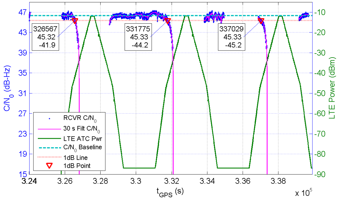
Receiver 135 Average C/N_0 for All Channels and LTE ATC Power at Receiver for TE10
