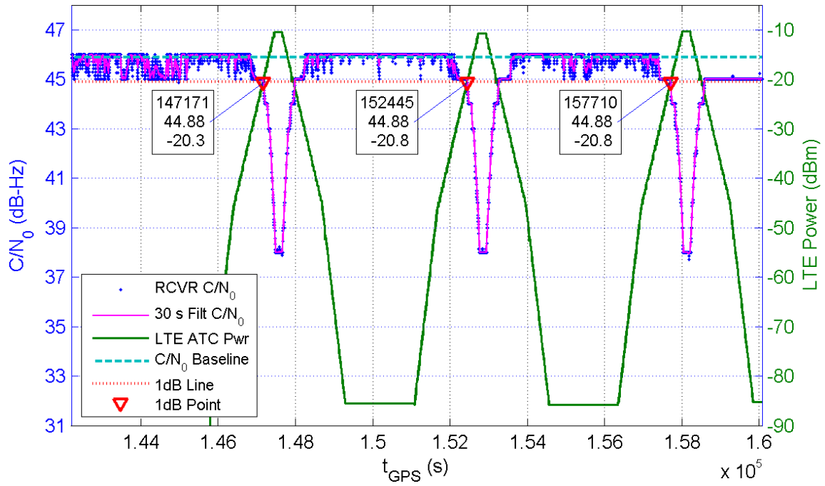
Receiver 314 Average C/N_0 for All Channels and LTE ATC Power at Receiver for TE1
