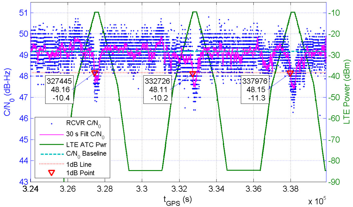
Receiver 363 Average C/N_0 for All Channels and LTE ATC Power at Receiver for TE10
