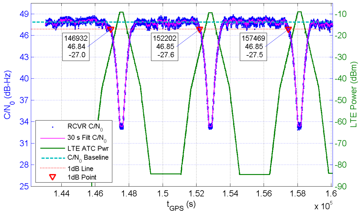
Receiver 370 Average C/N_0 for All Channels and LTE ATC Power at Receiver for TE1
