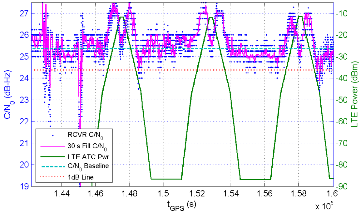
Receiver 395 Average C/N_0 for All Channels and LTE ATC Power at Receiver for TE1
