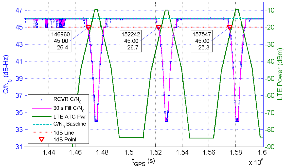
Receiver 360 Average C/N_0 for All Channels and LTE ATC Power at Receiver for TE1
