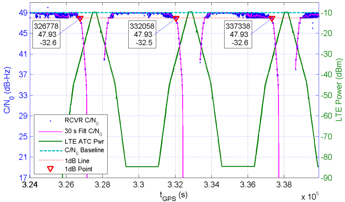
Receiver 304 Average C/N_0 for All Channels and LTE ATC Power at Receiver for TE10
