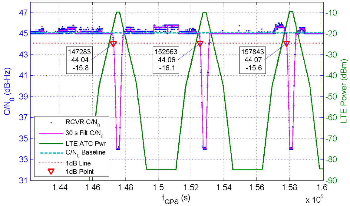
Receiver 124 Average C/N_0 for All Channels and LTE ATC Power at Receiver for TE1
