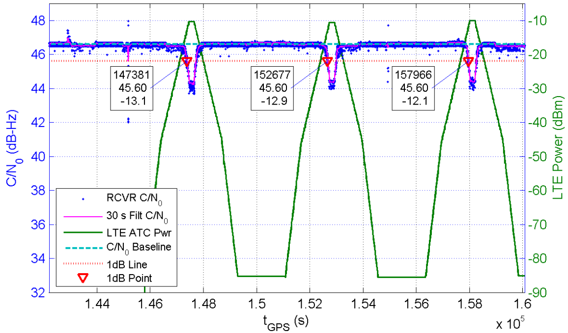
Receiver 118 Average C/N_0 for All Channels and LTE ATC Power at Receiver for TE1
