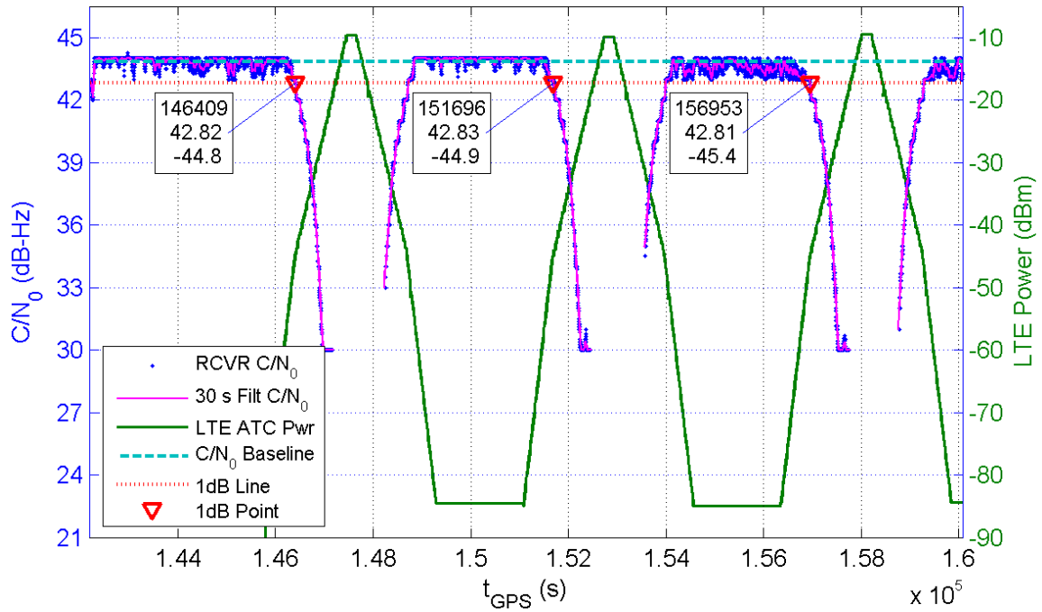
Receiver 366 Average C/N_0 for All Channels and LTE ATC Power at Receiver for TE1
