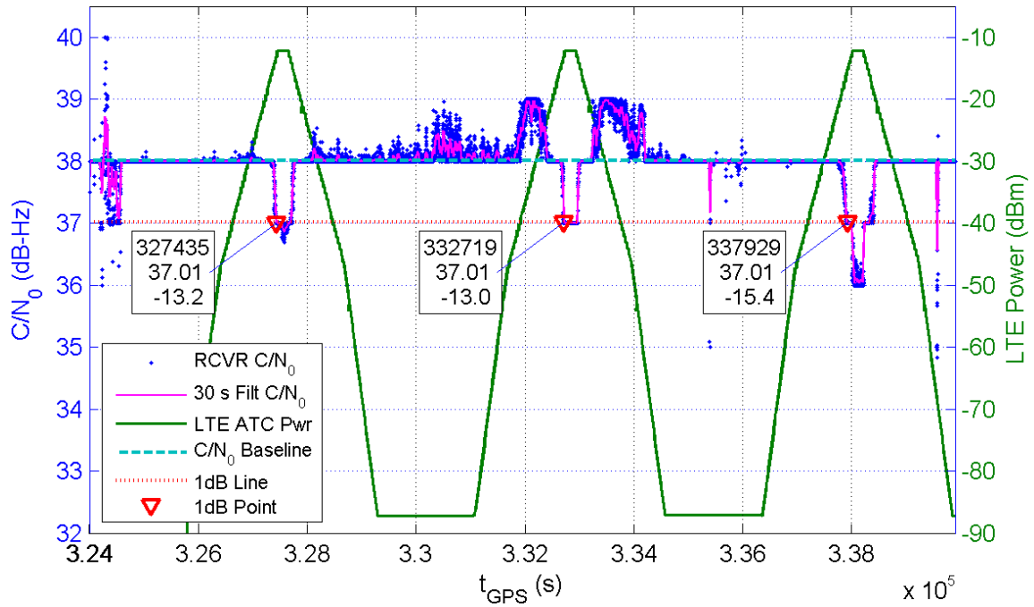
Receiver 330 Average C/N_0 for All Channels and LTE ATC Power at Receiver for TE10
