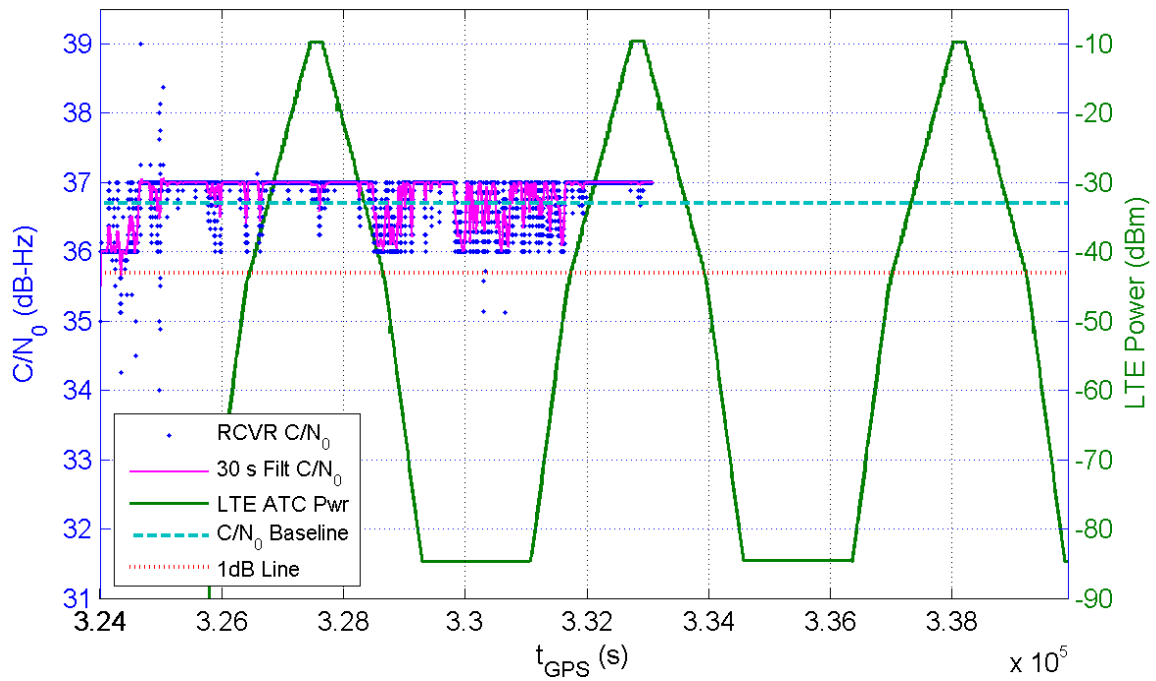
Receiver 217 Average C/N_0 for All Channels and LTE ATC Power at Receiver for TE10
