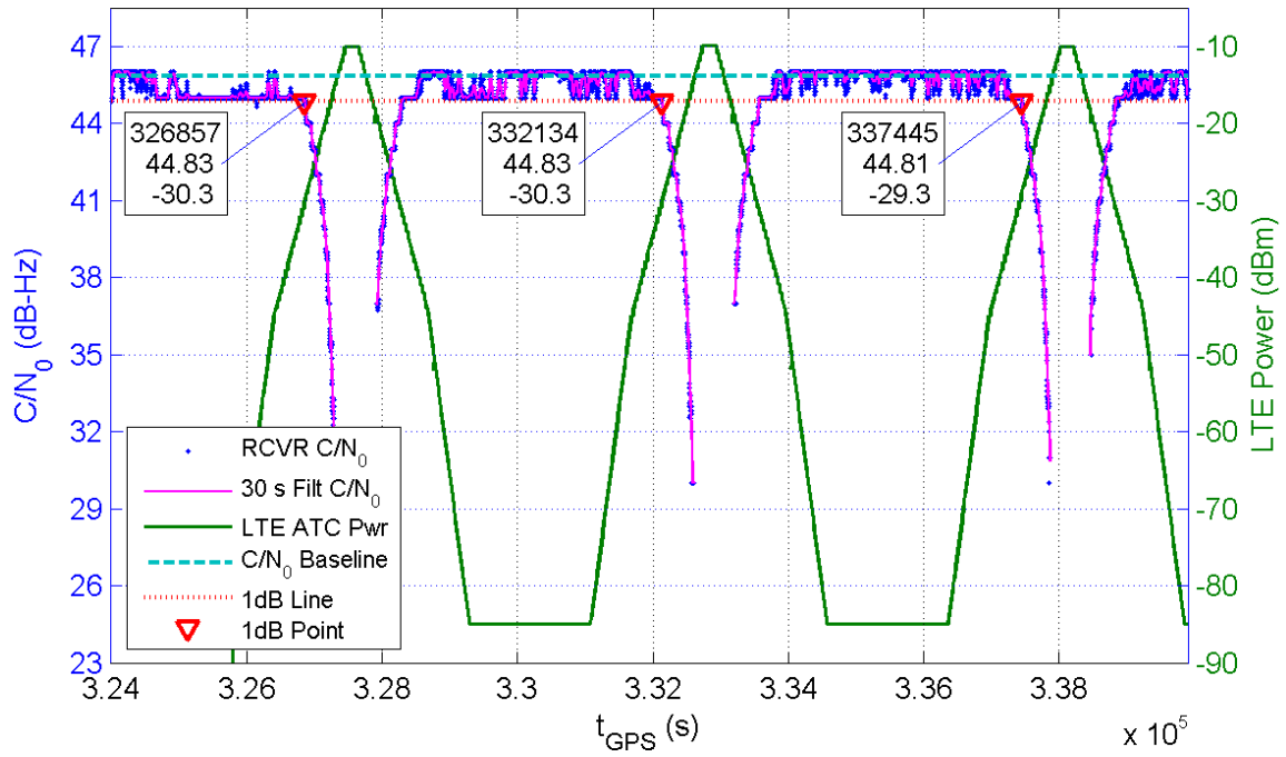
Receiver 319 Average C/N_0 for All Channels and LTE ATC Power at Receiver for TE10
