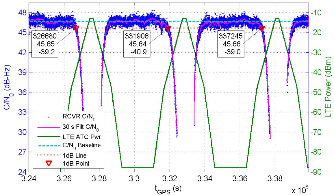
Receiver 247 Average C/N_0 for All Channels and LTE ATC Power at Receiver for TE10
