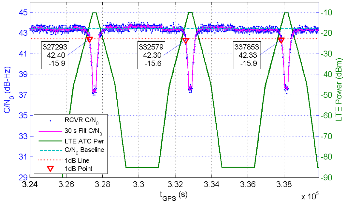
Receiver 203 Average C/N_0 for All Channels and LTE ATC Power at Receiver for TE10
