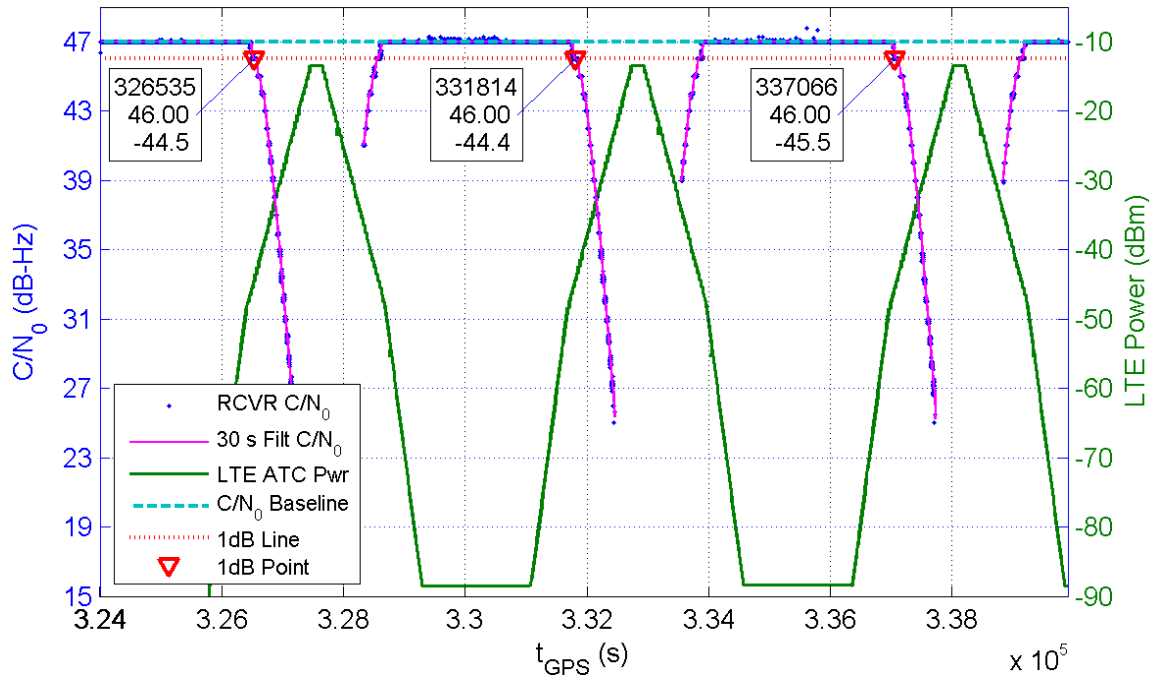
Receiver 231 Average C/N_0 for All Channels and LTE ATC Power at Receiver for TE10
