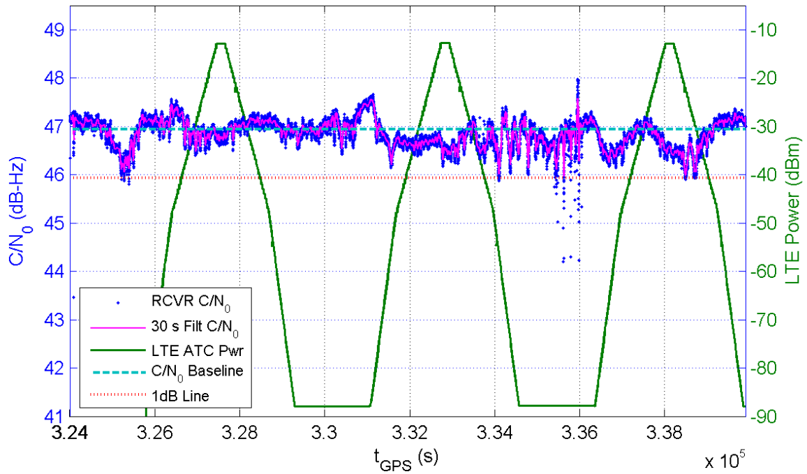
Receiver 234 Average C/N_0 for All Channels and LTE ATC Power at Receiver for TE10
