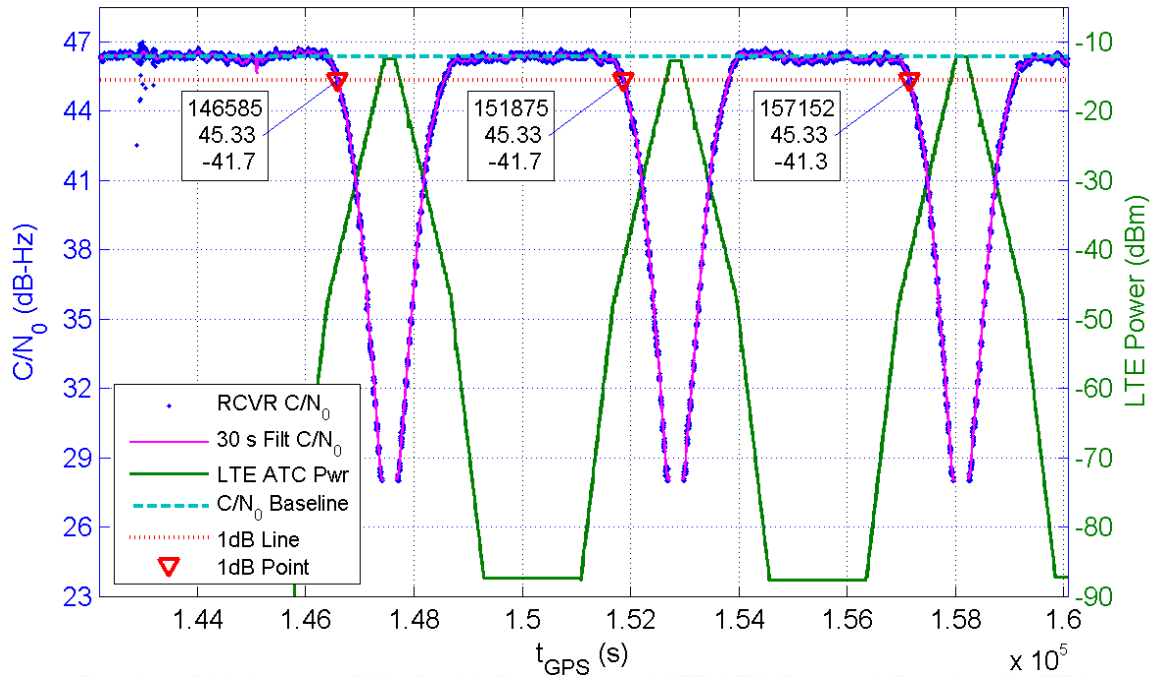
Receiver 341 Average C/N_0 for All Channels and LTE ATC Power at Receiver for TE1
