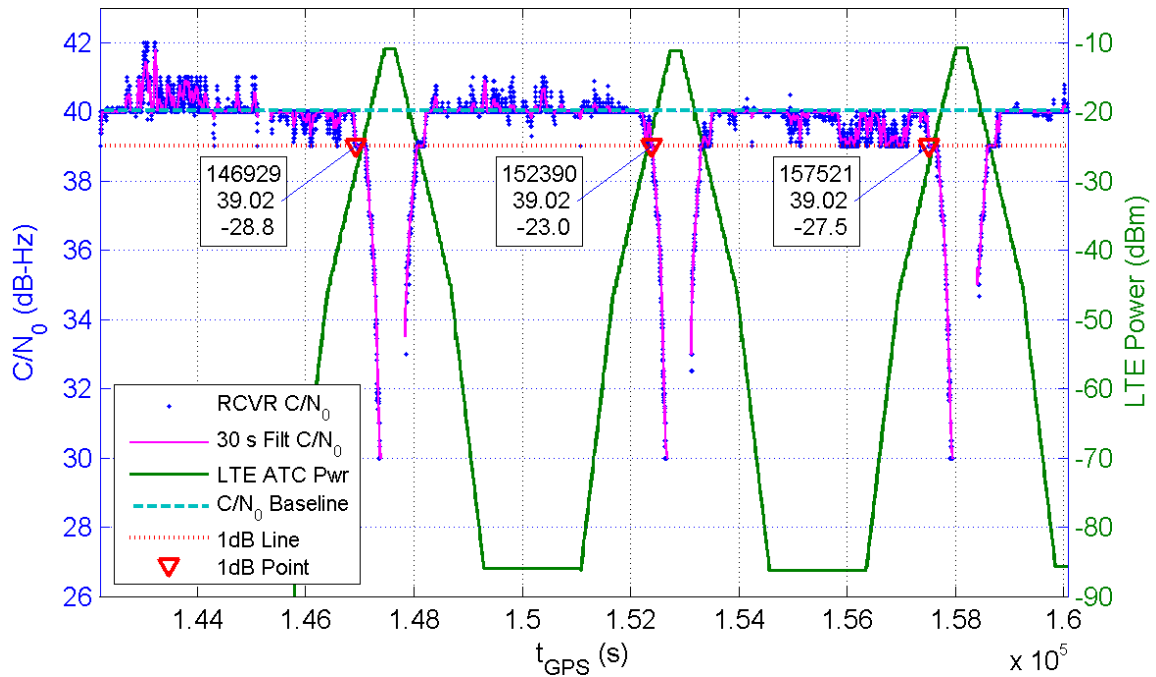
Receiver 368 Average C/N_0 for All Channels and LTE ATC Power at Receiver for TE1
