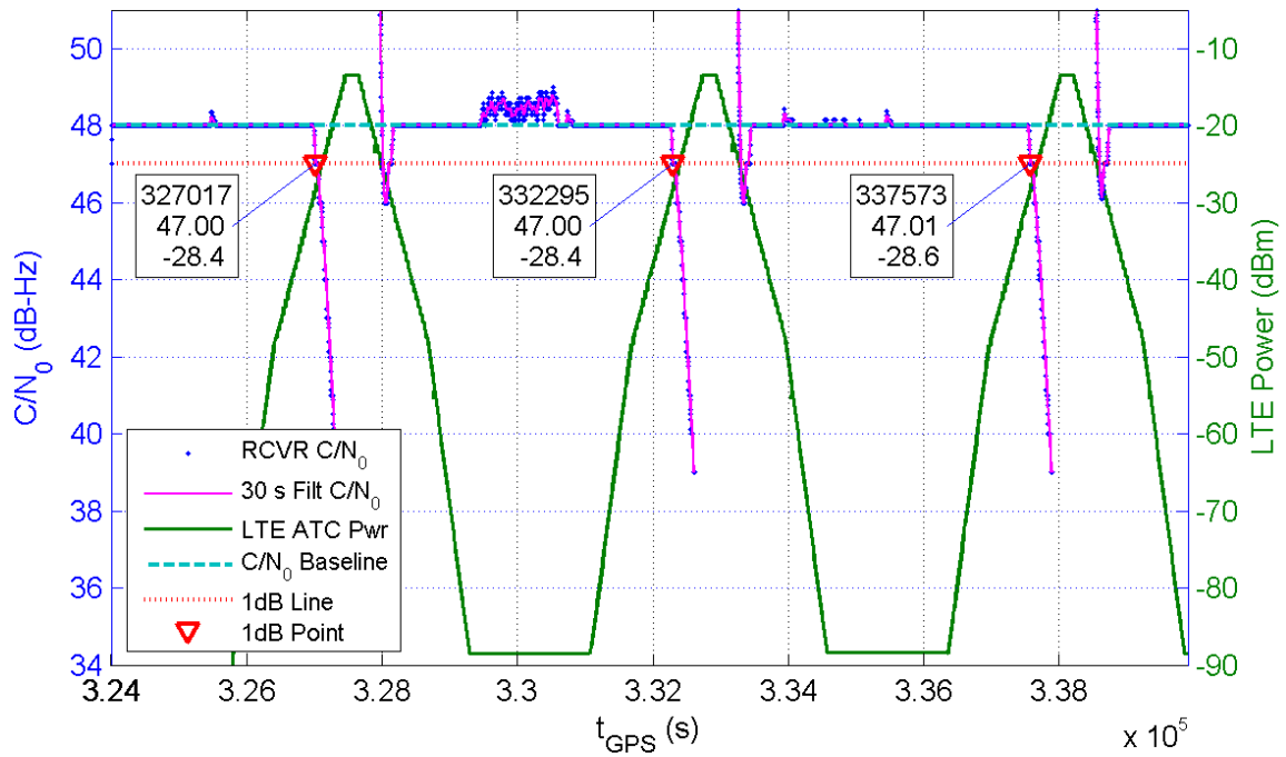
Receiver 246 Average C/N_0 for All Channels and LTE ATC Power at Receiver for TE10
