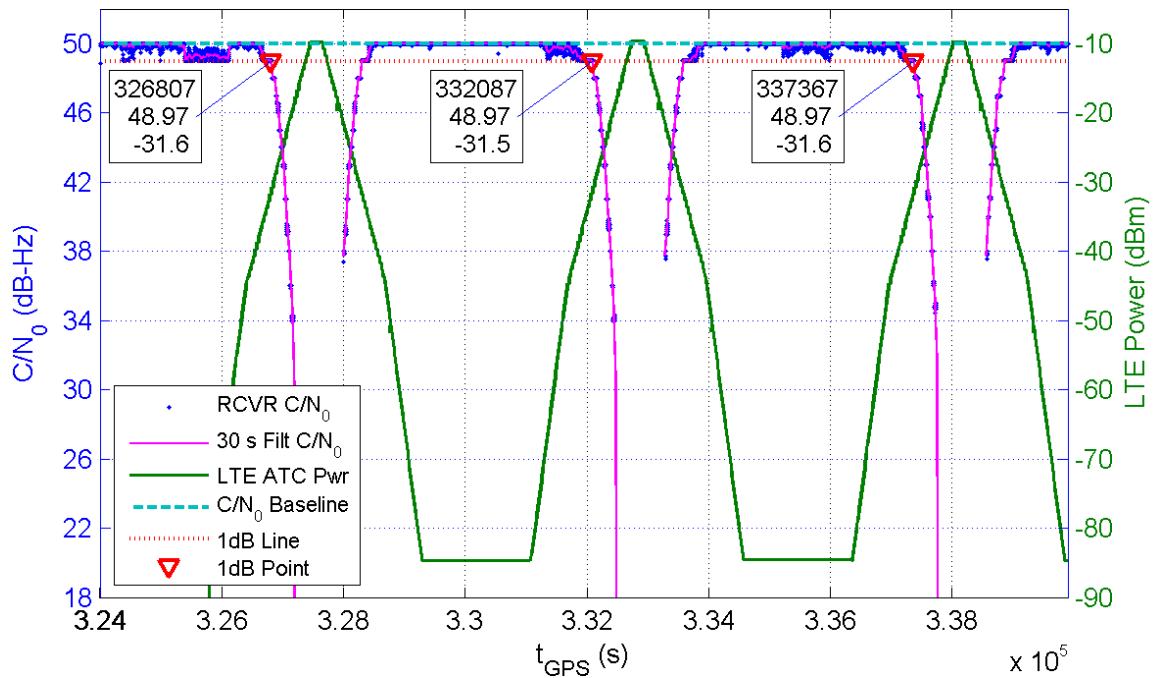
Receiver 220 Average C/N_0 for All Channels and LTE ATC Power at Receiver for TE10
