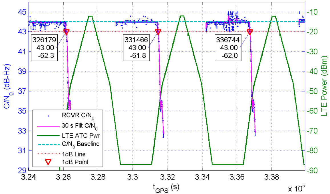
Receiver 359 Average C/N_0 for All Channels and LTE ATC Power at Receiver for TE10
