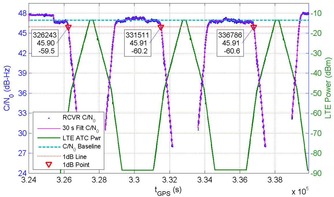
Receiver 215 Average C/N_0 for All Channels and LTE ATC Power at Receiver for TE10
