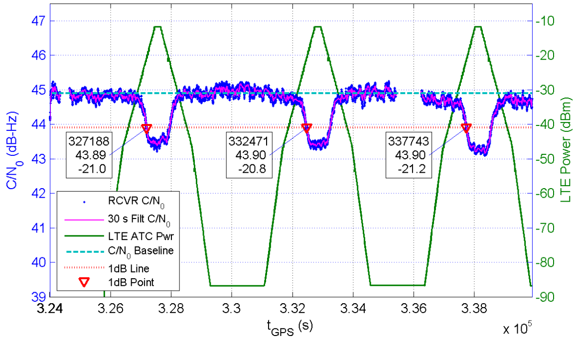
Receiver 302 Average C/N_0 for All Channels and LTE ATC Power at Receiver for TE10
