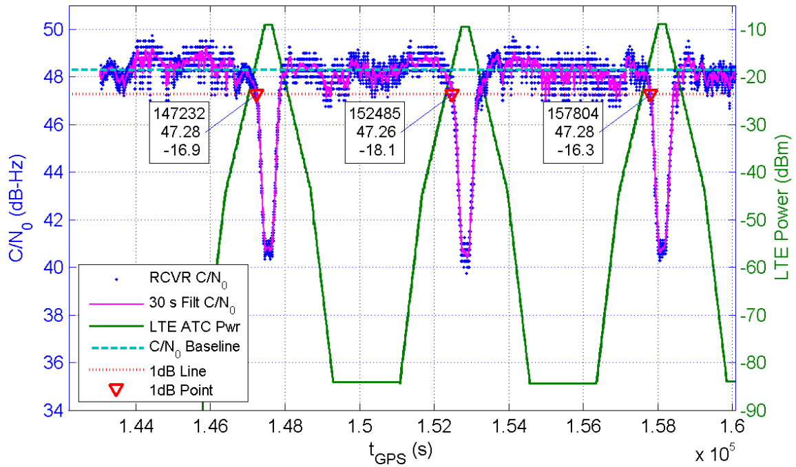
Receiver 351 Average C/N_0 for All Channels and LTE ATC Power at Receiver for TE1
