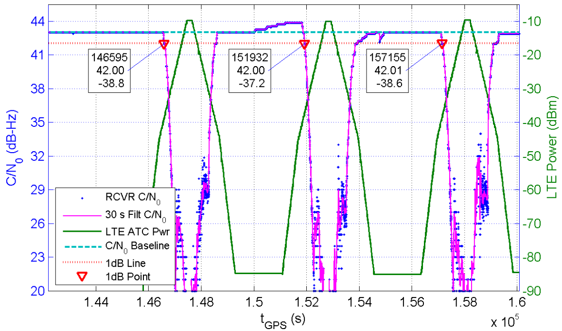
Receiver 207 Average C/N_0 for All Channels and LTE ATC Power at Receiver for TE1
