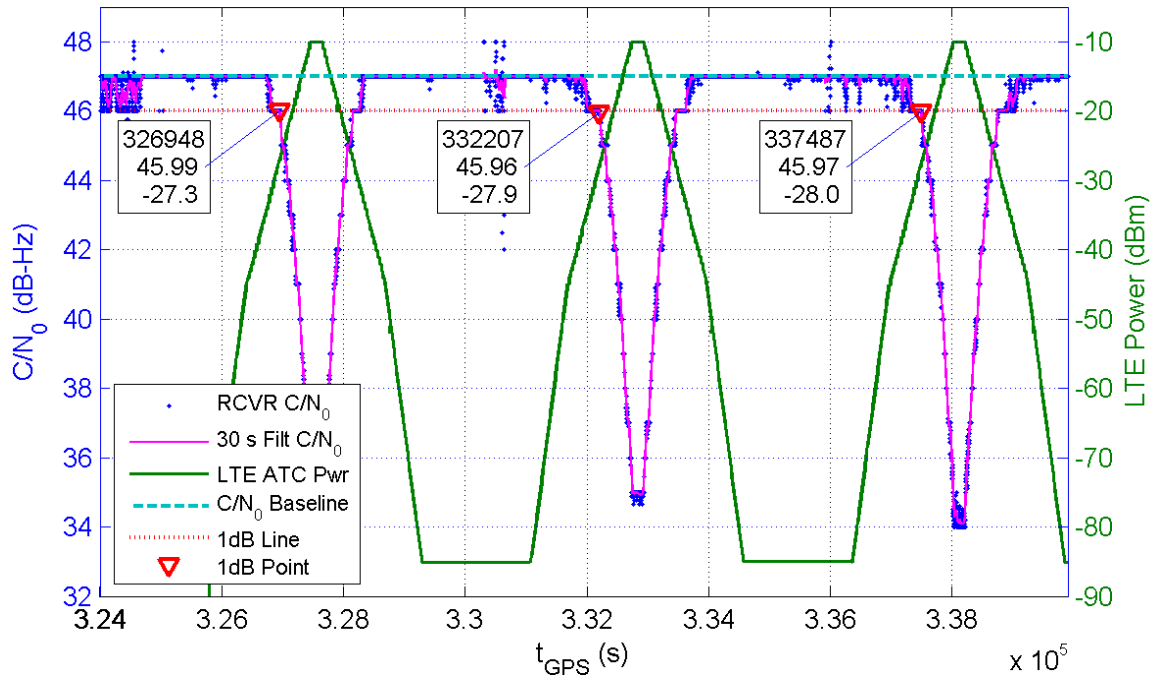
Receiver 335 Average C/N_0 for All Channels and LTE ATC Power at Receiver for TE10
