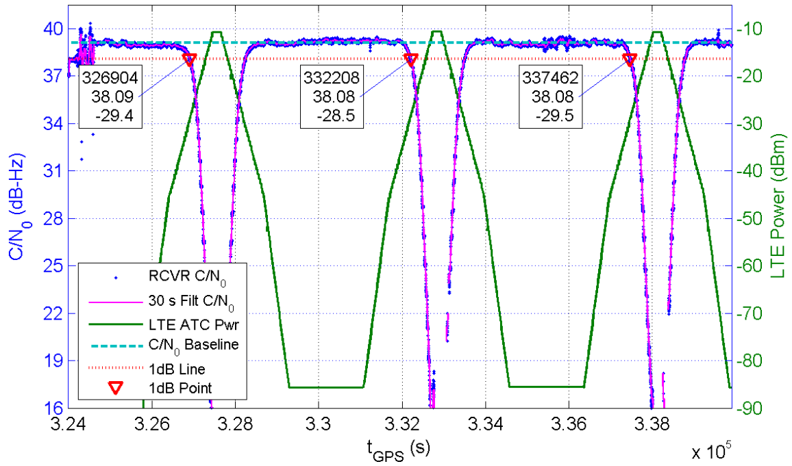
Receiver 211 Average C/N_0 for All Channels and LTE ATC Power at Receiver for TE10
