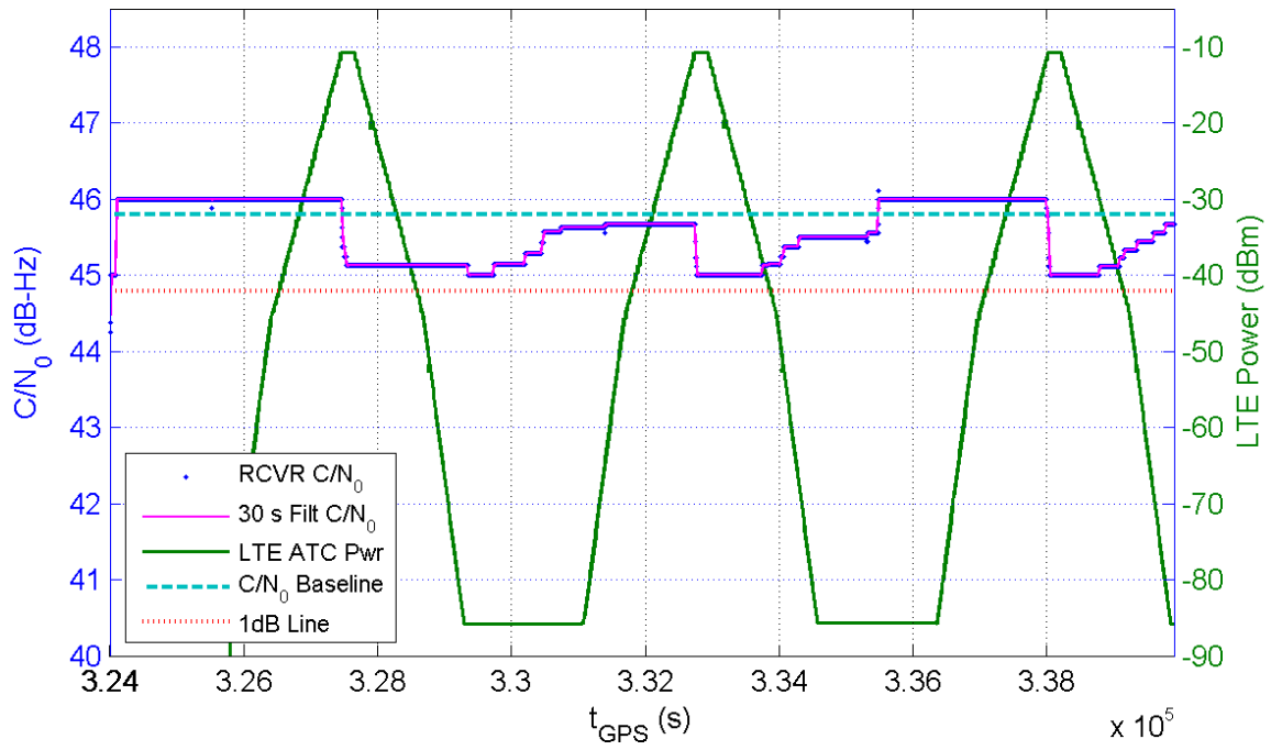
Receiver 392 Average C/N_0 for All Channels and LTE ATC Power at Receiver for TE10
