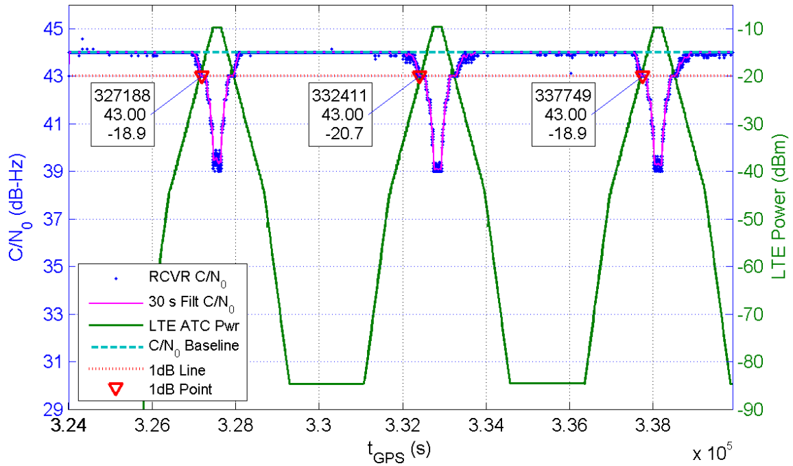
Receiver 326 Average C/N_0 for All Channels and LTE ATC Power at Receiver for TE10
