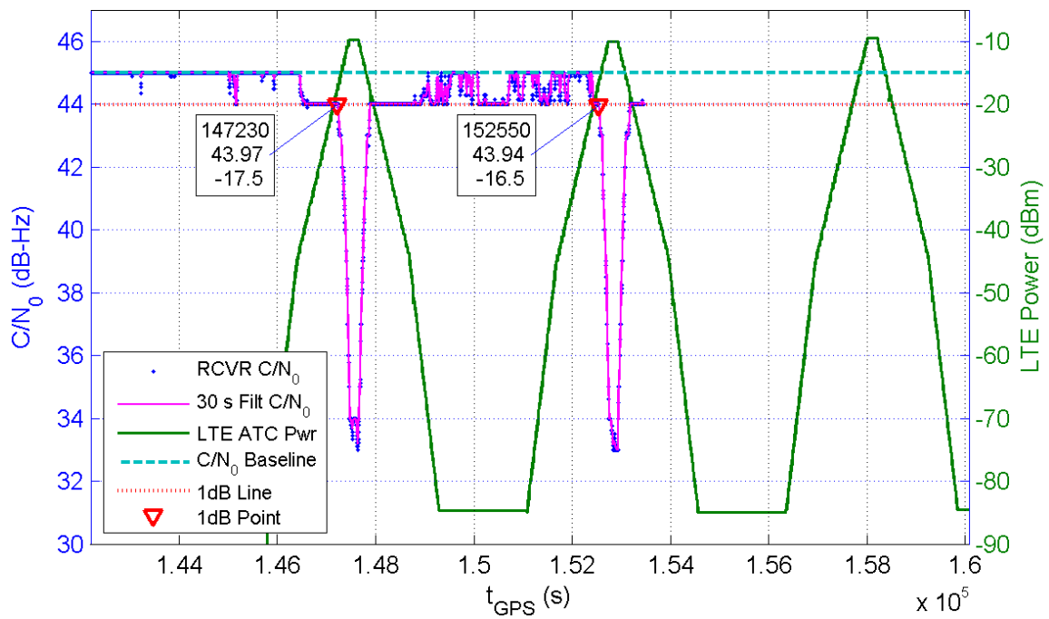
Receiver 338 Average C/N_0 for All Channels and LTE ATC Power at Receiver for TE1
