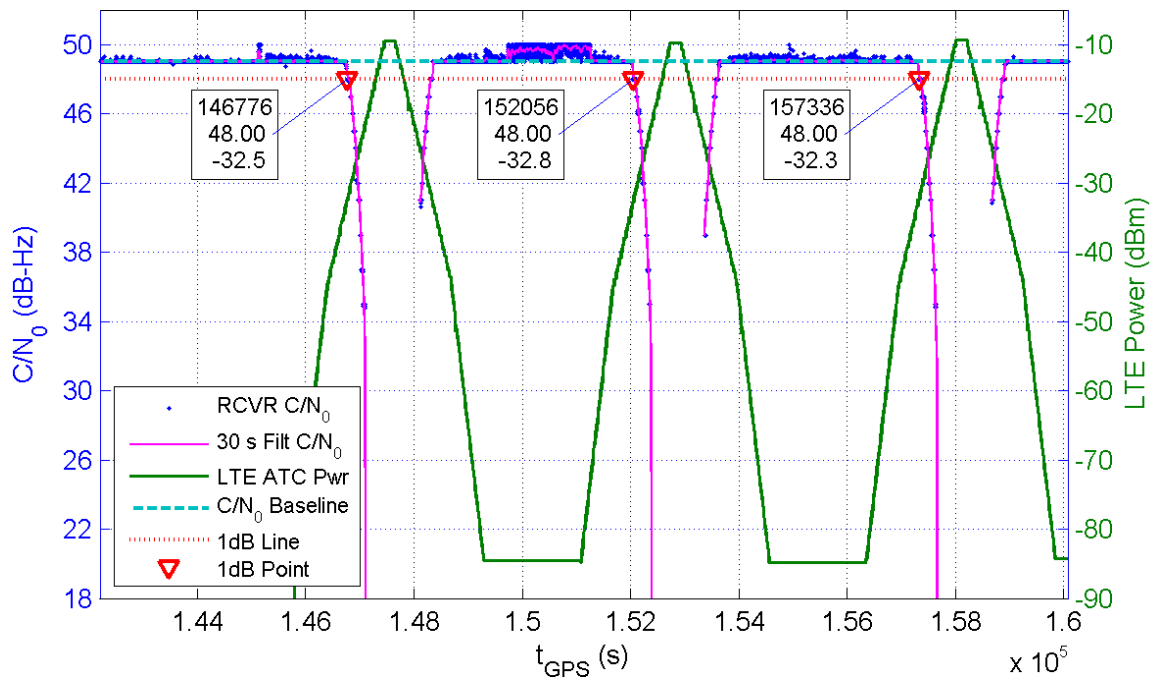
Receiver 348 Average C/N_0 for All Channels and LTE ATC Power at Receiver for TE1
