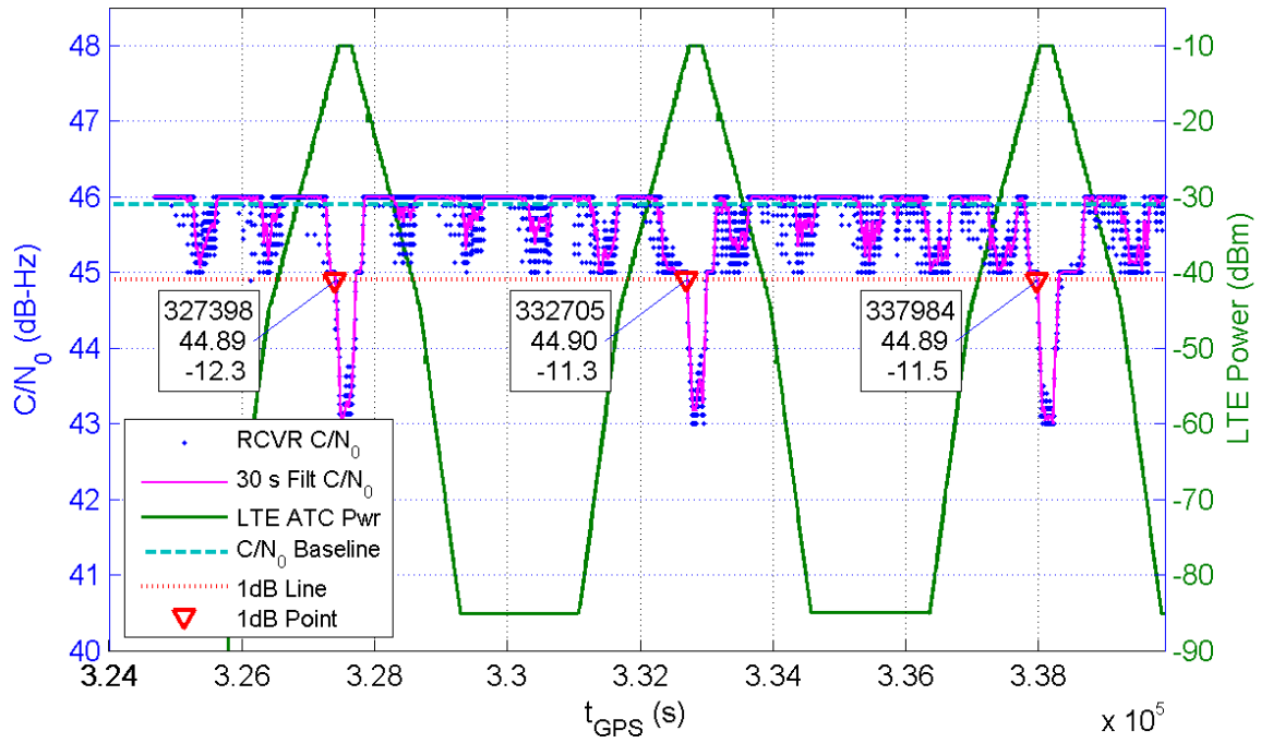
Receiver 306 Average C/N_0 for All Channels and LTE ATC Power at Receiver for TE10
