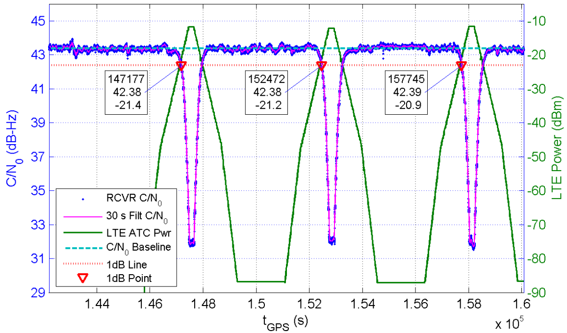
Receiver 201 Average C/N_0 for All Channels and LTE ATC Power at Receiver for TE1
