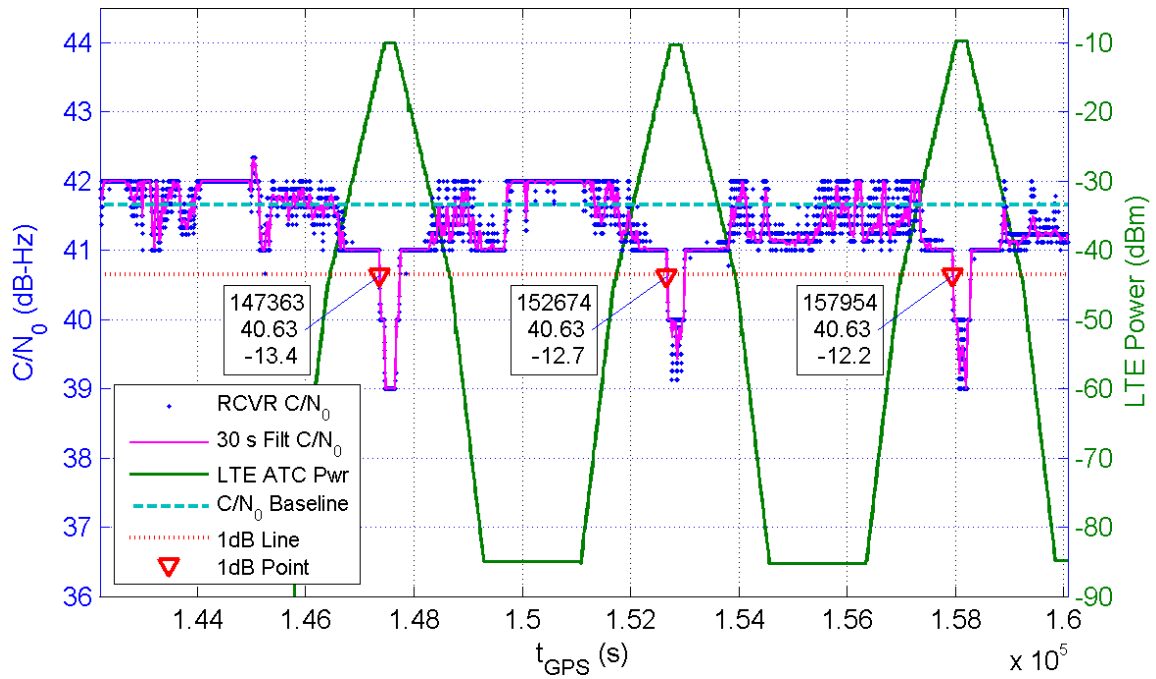
Receiver 361 Average C/N_0 for All Channels and LTE ATC Power at Receiver for TE1
