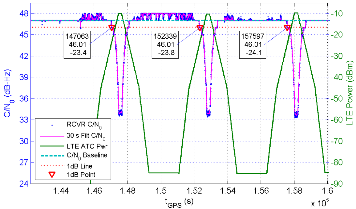
Receiver 337 Average C/N_0 for All Channels and LTE ATC Power at Receiver for TE1
