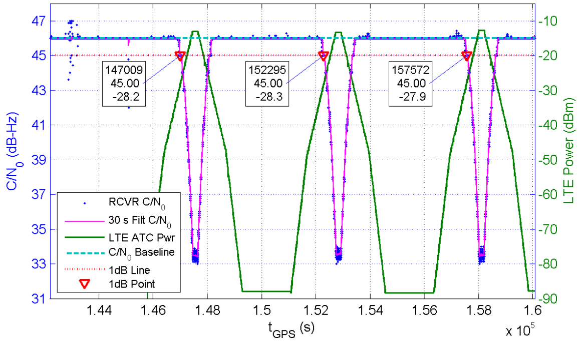
Receiver 114 Average C/N_0 for All Channels and LTE ATC Power at Receiver for TE1
