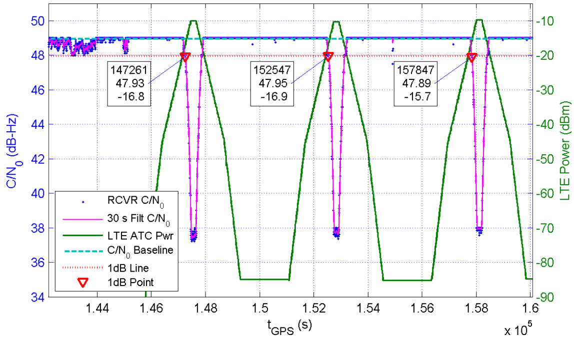
Receiver 379 Average C/N_0 for All Channels and LTE ATC Power at Receiver for TE1
