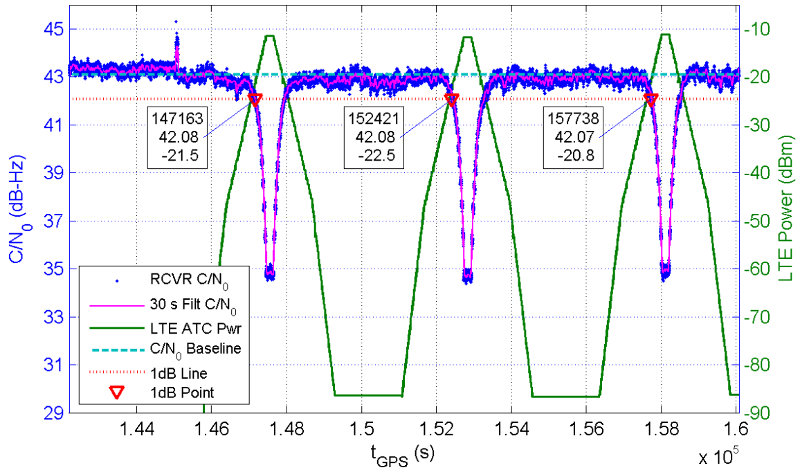
Receiver 316 Average C/N_0 for All Channels and LTE ATC Power at Receiver for TE1
