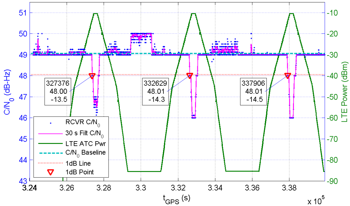
Receiver 384 Average C/N_0 for All Channels and LTE ATC Power at Receiver for TE10
