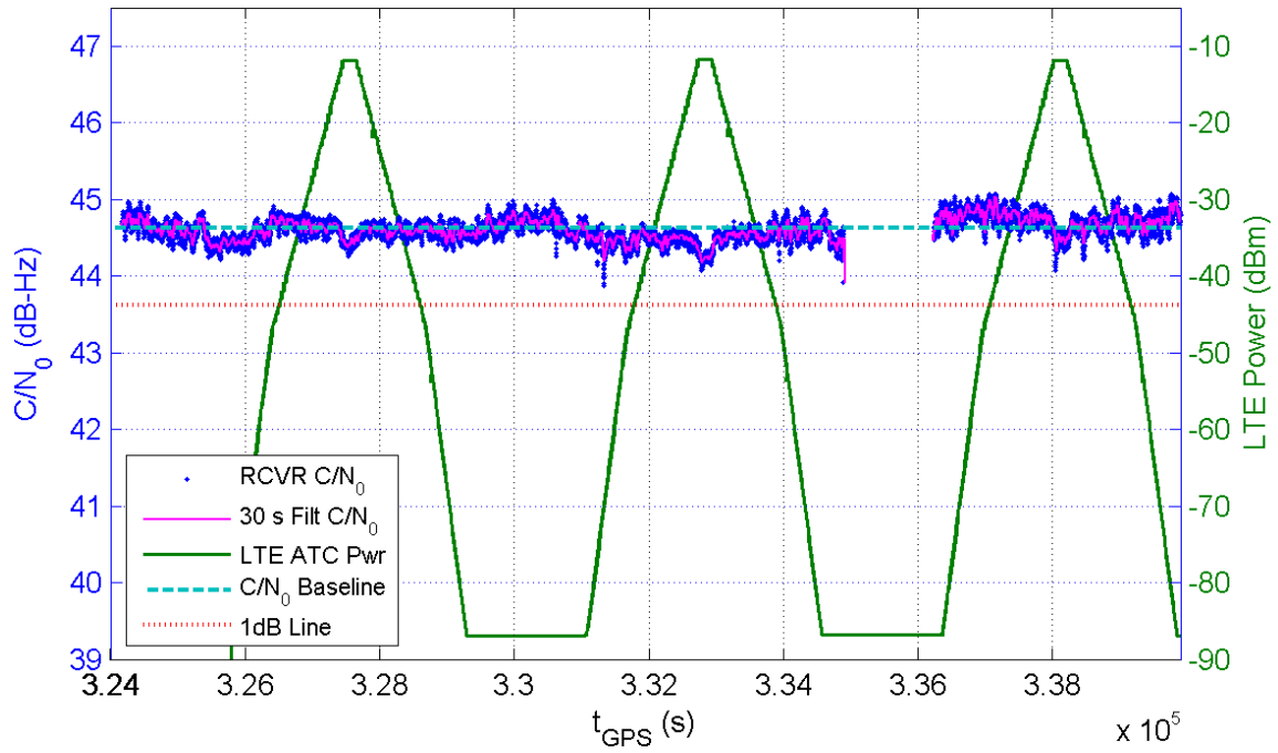
Receiver 385 Average C/N_0 for All Channels and LTE ATC Power at Receiver for TE10
