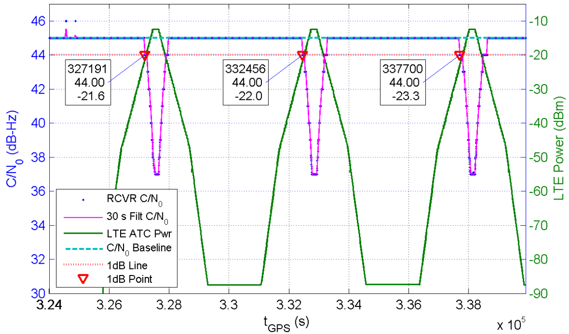
Receiver 232 Average C/N_0 for All Channels and LTE ATC Power at Receiver for TE10
