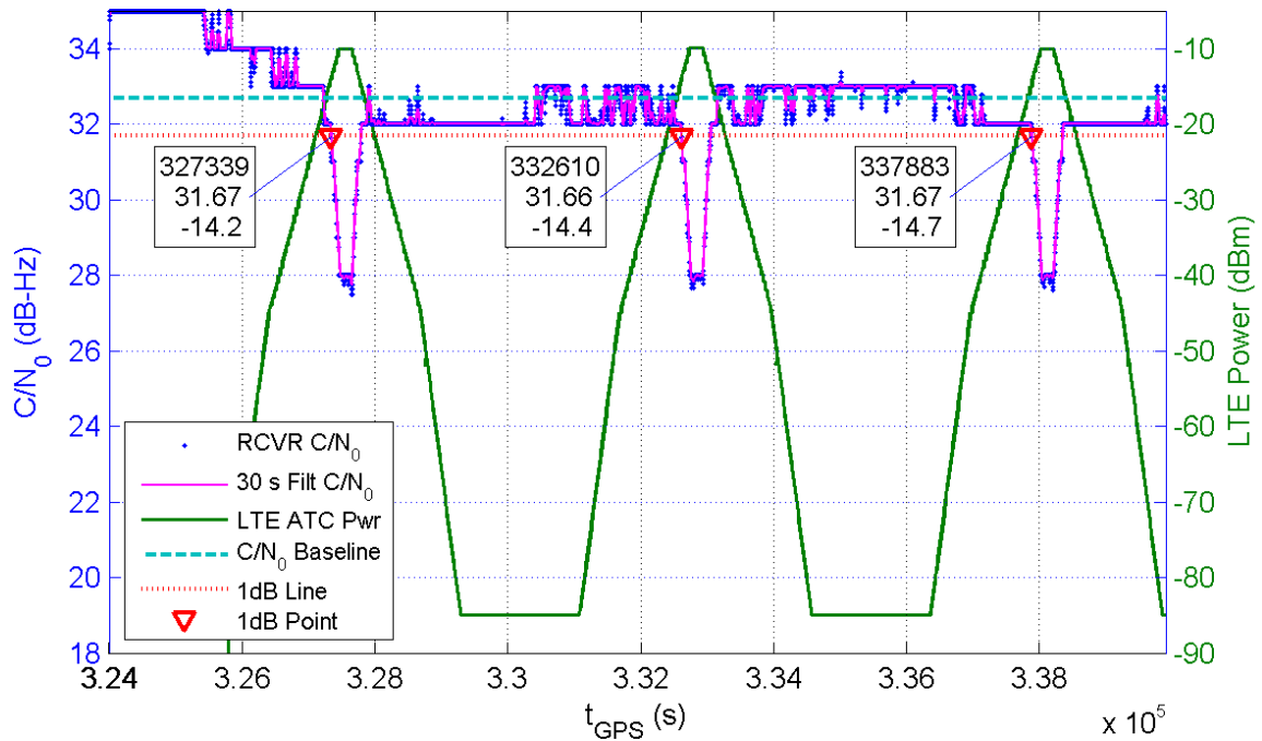
Receiver 378 Average C/N_0 for All Channels and LTE ATC Power at Receiver for TE10
