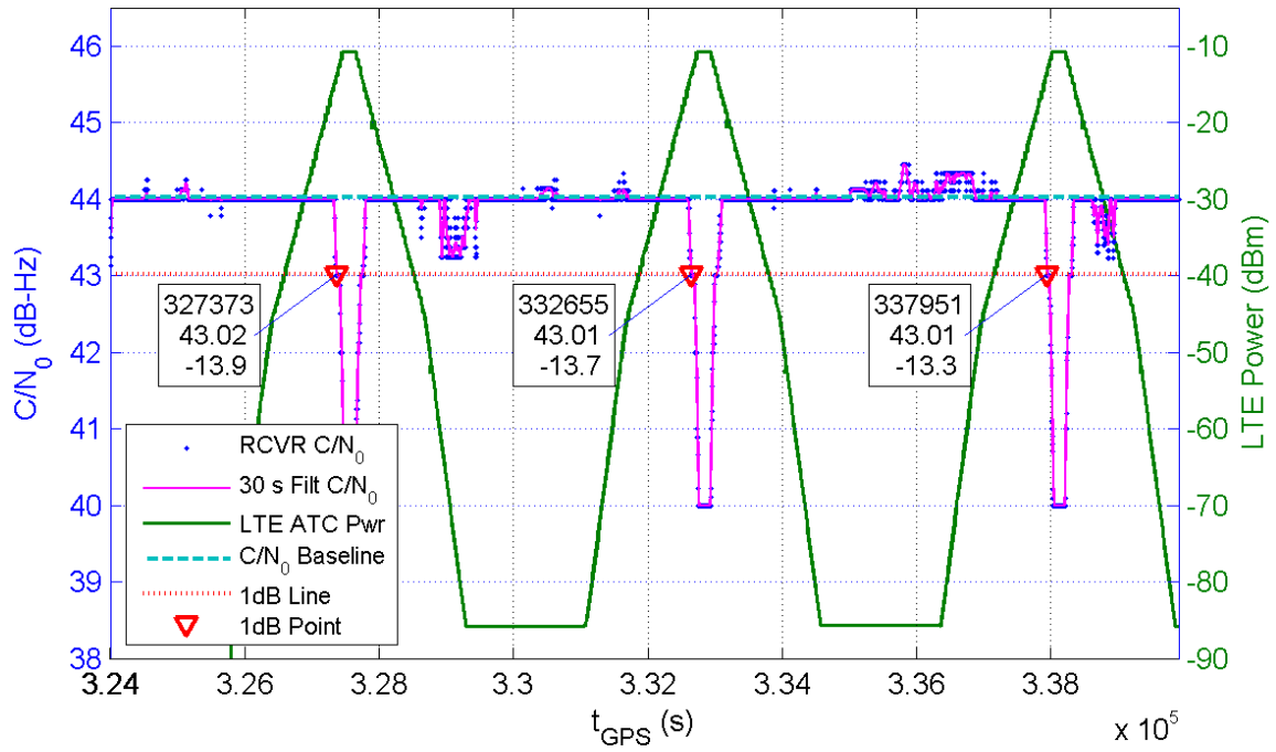
Receiver 308 Average C/N_0 for All Channels and LTE ATC Power at Receiver for TE10
