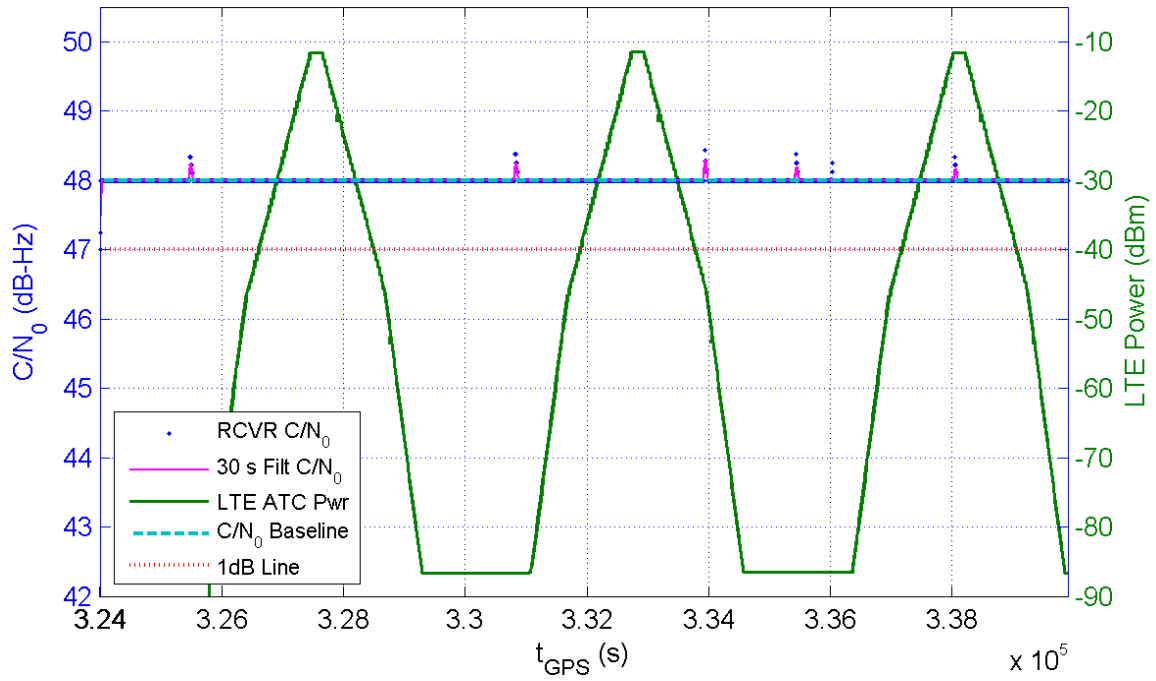
Receiver 219 Average C/N_0 for All Channels and LTE ATC Power at Receiver for TE10
