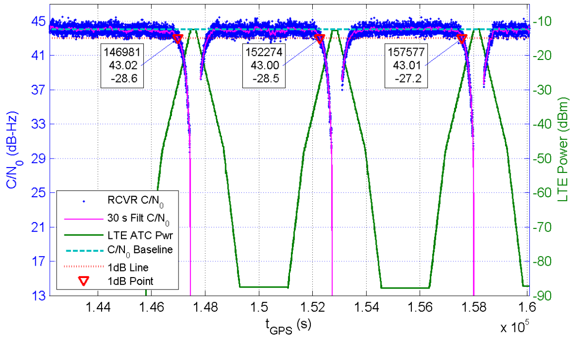
Receiver 235 Average C/N_0 for All Channels and LTE ATC Power at Receiver for TE1
