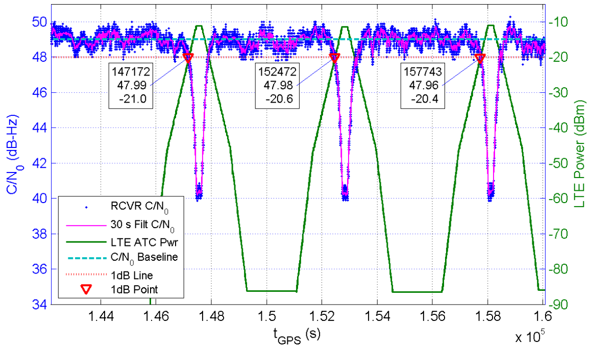
Receiver 321 Average C/N_0 for All Channels and LTE ATC Power at Receiver for TE1
