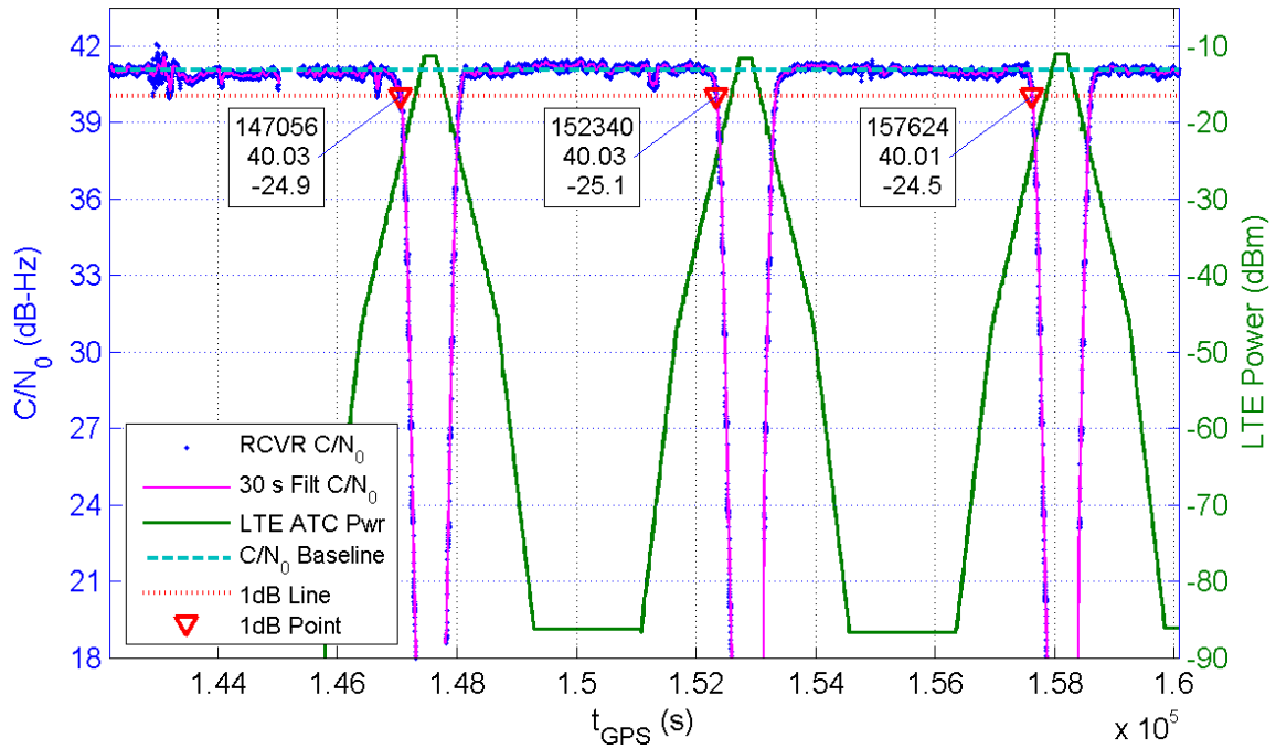
Receiver 371 Average C/N_0 for All Channels and LTE ATC Power at Receiver for TE1
