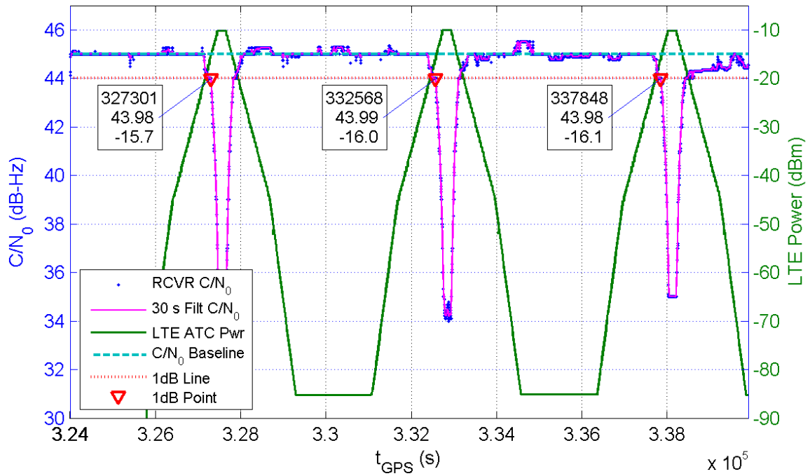
Receiver 338 Average C/N_0 for All Channels and LTE ATC Power at Receiver for TE10
