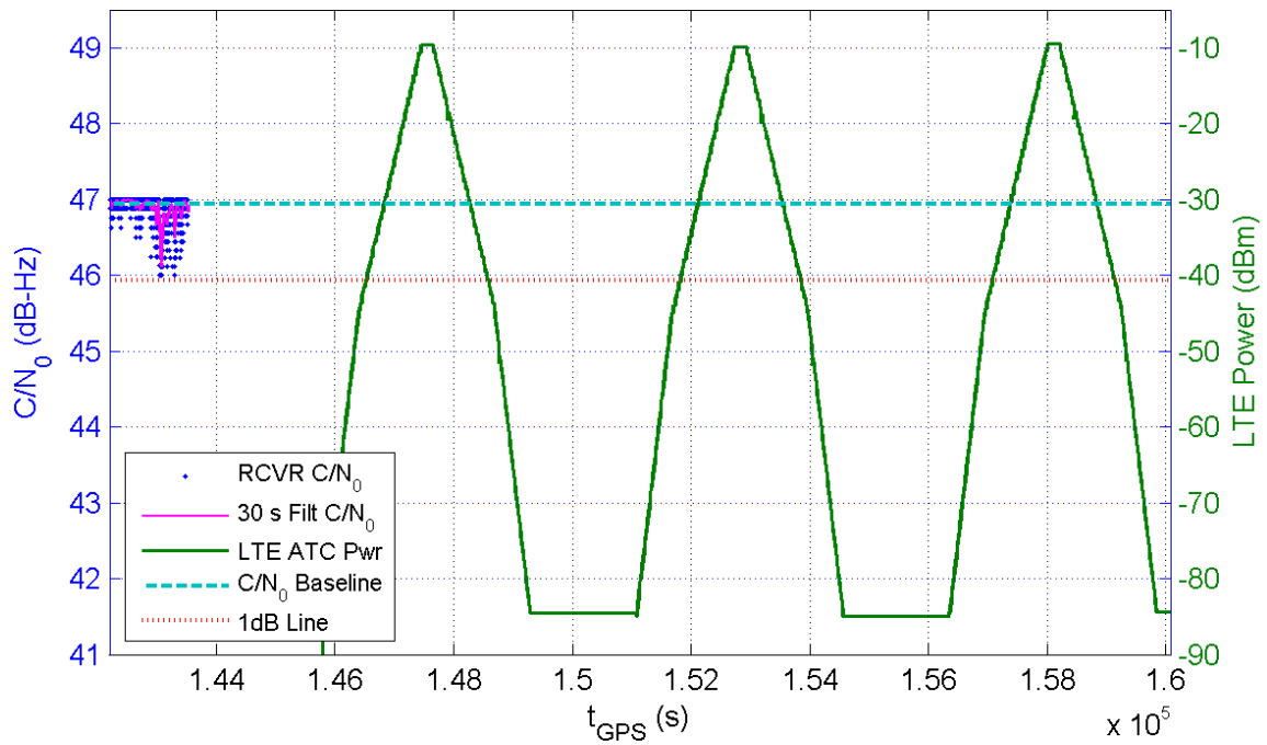
Receiver 115 Average C/N_0 for All Channels and LTE ATC Power at Receiver for TE1
