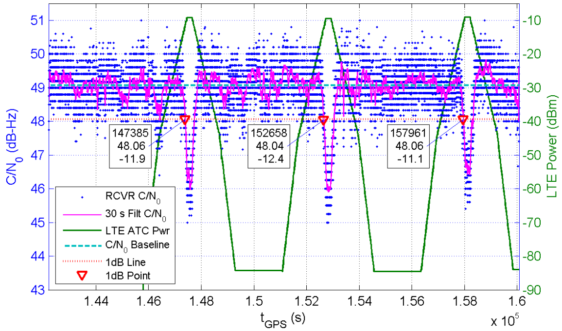
Receiver 363 Average C/N_0 for All Channels and LTE ATC Power at Receiver for TE1
