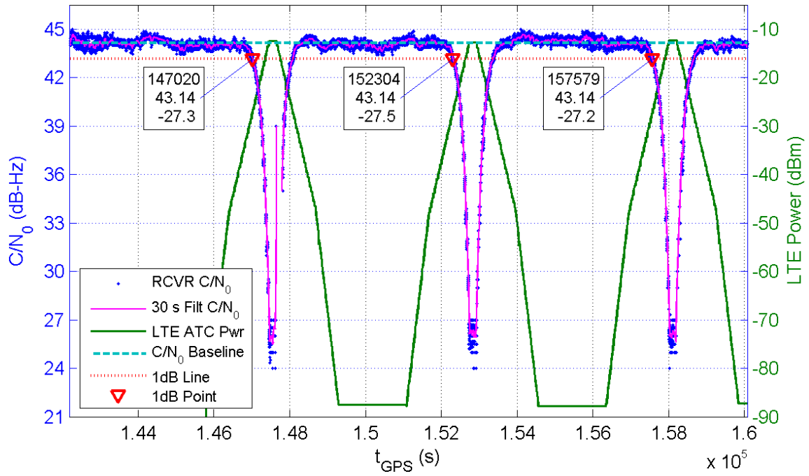
Receiver 394 Average C/N_0 for All Channels and LTE ATC Power at Receiver for TE1
