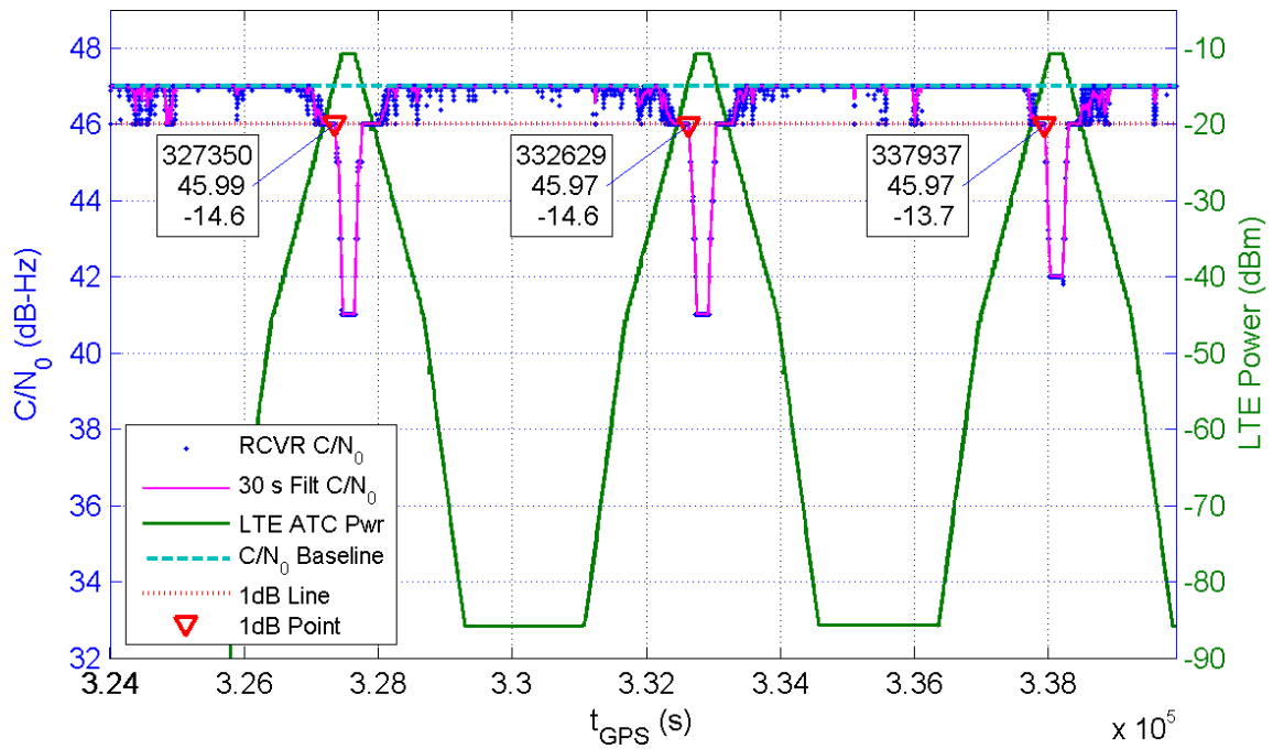
Receiver 205 Average C/N_0 for All Channels and LTE ATC Power at Receiver for TE10
