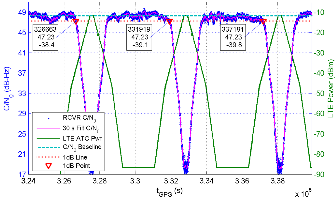
Receiver 312 Average C/N_0 for All Channels and LTE ATC Power at Receiver for TE10
