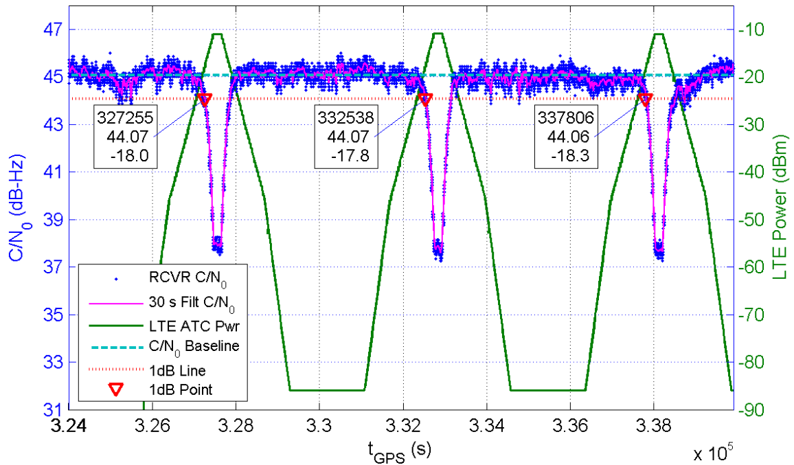
Receiver 364 Average C/N_0 for All Channels and LTE ATC Power at Receiver for TE10
