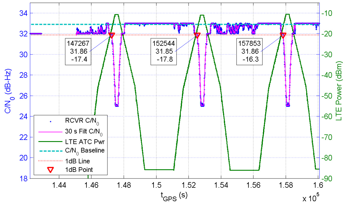
Receiver 110 Average C/N_0 for All Channels and LTE ATC Power at Receiver for TE1
