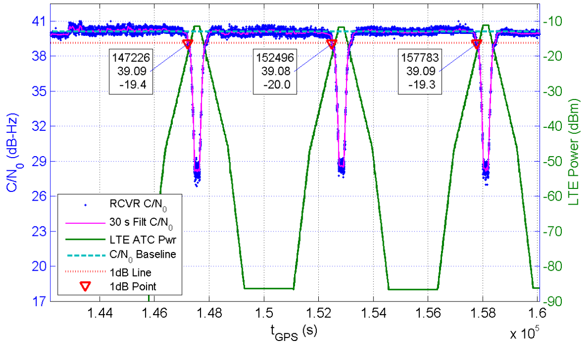
Receiver 374 Average C/N_0 for All Channels and LTE ATC Power at Receiver for TE1
