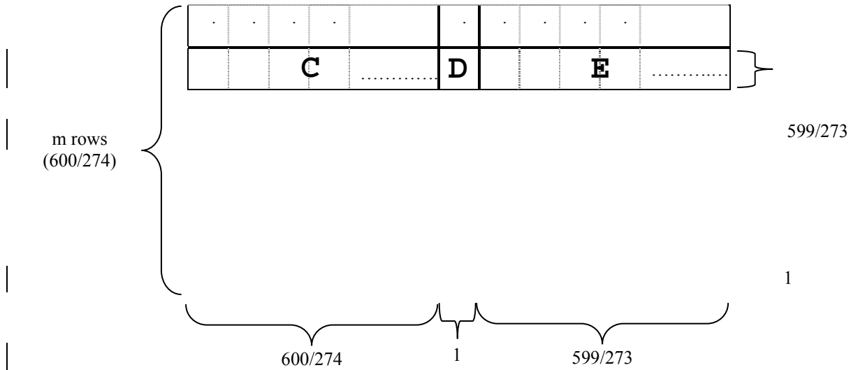
Figure 3.2-5. Parity Check Matrix H for LDPC Code
