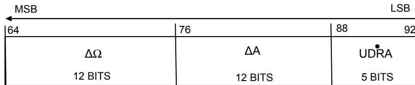
Figure 3.5-10. Differential Correction Data Packet
