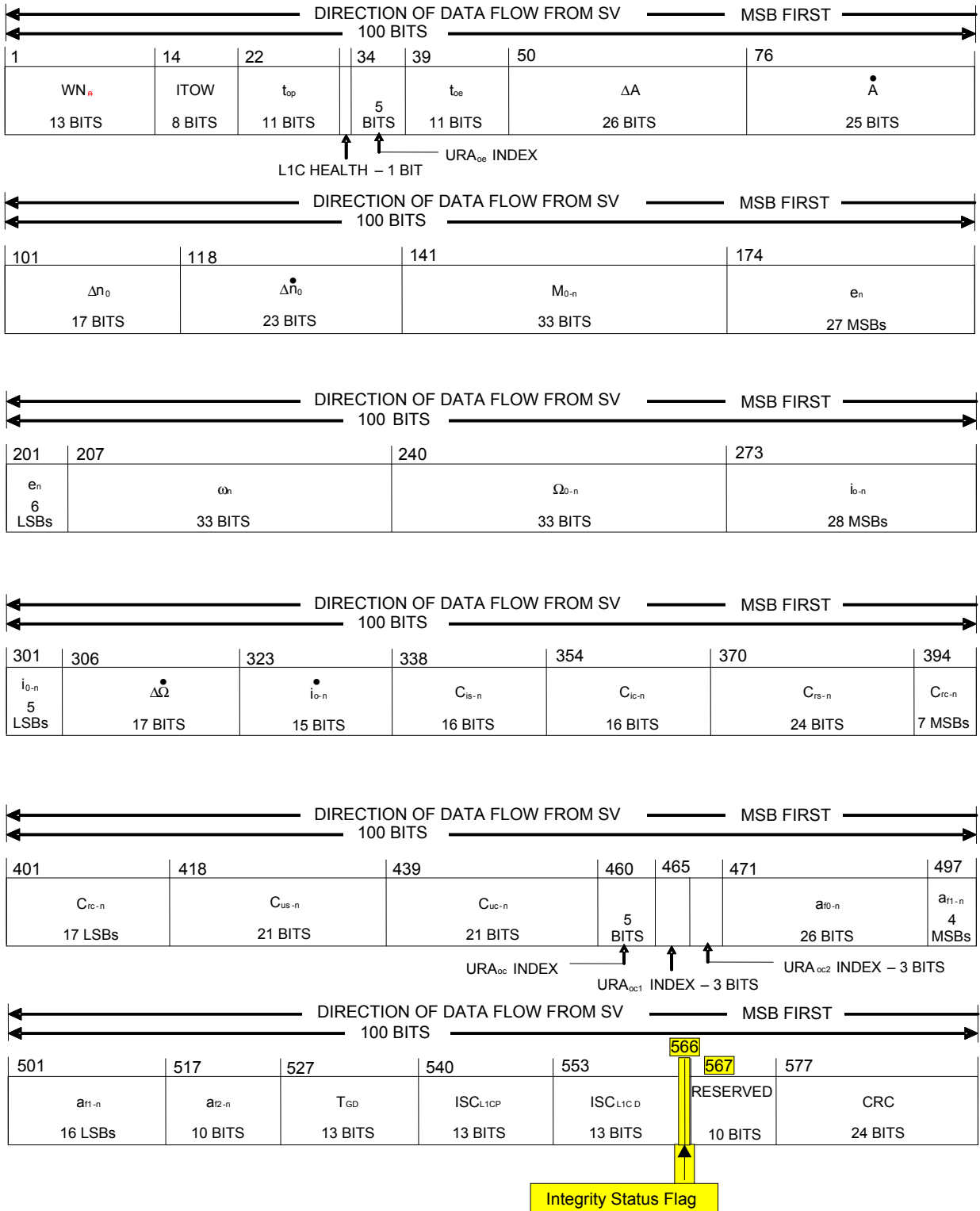
Figure 3.5-1. Subframe 2 – Clock, Ephemeris, ITOW
