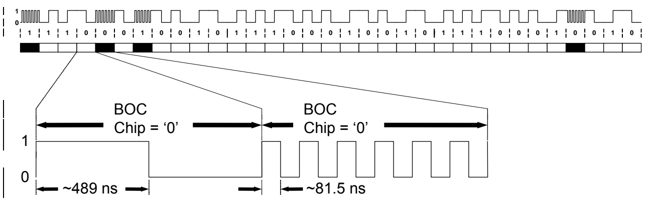
(c) Combined 33 symbol sequence showing BOC (6,1) chips at 0,4,6, and 29
