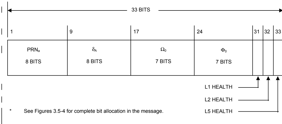
Figure 3.5-9. Reduced Almanac Packet Content
