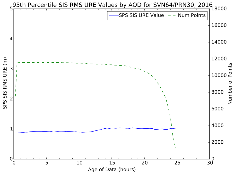
Figure 3.7: Best Performing Block IIF SV in Terms of Any AOD (SVN 64/PRN 30)
