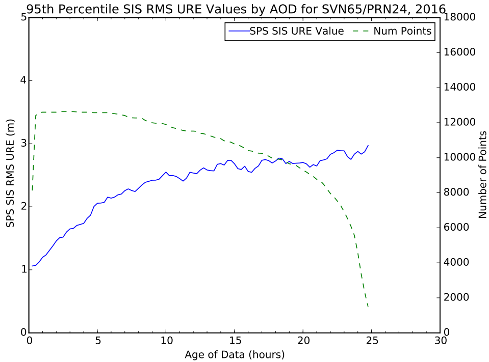
Figure 3.5: Worst Performing Block IIF SV in Terms of Any AOD (SVN 65/PRN 24)
