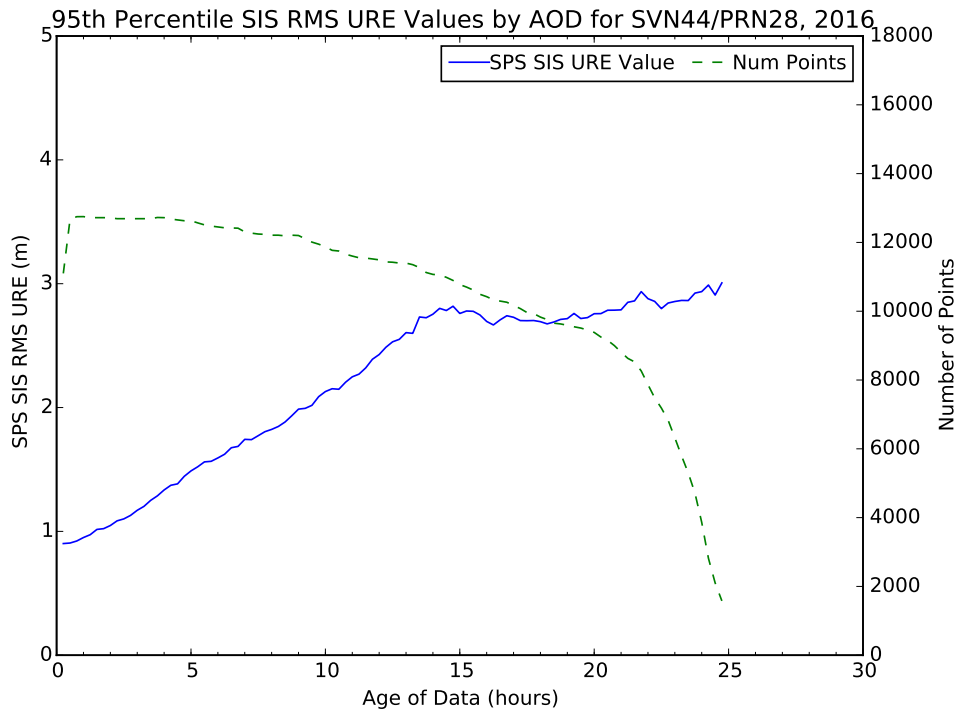
Figure 3.4: Worst Performing Block IIR/IIR-M SV in Terms of Any AOD (SVN 44/PRN 28)
