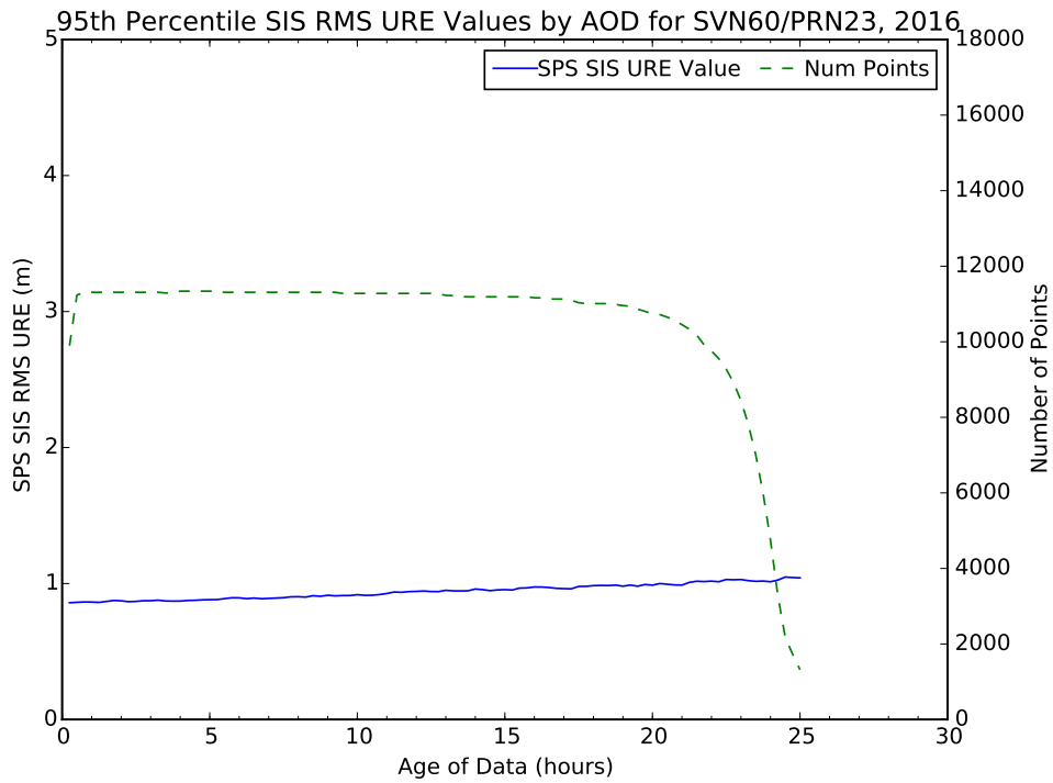
Figure 3.6: Best Performing Block IIR/IIR-M SV in Terms of Any AOD (SVN 60/PRN 23)
