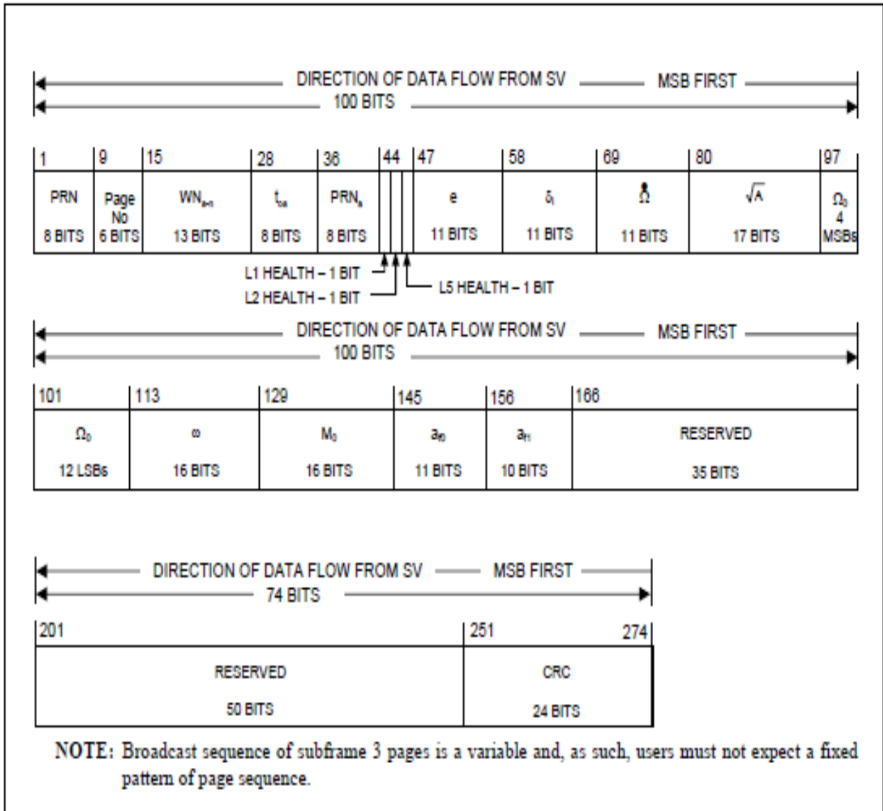
Figure 3.5-5. Subframe 3, Page 4 - Midi Almanac
