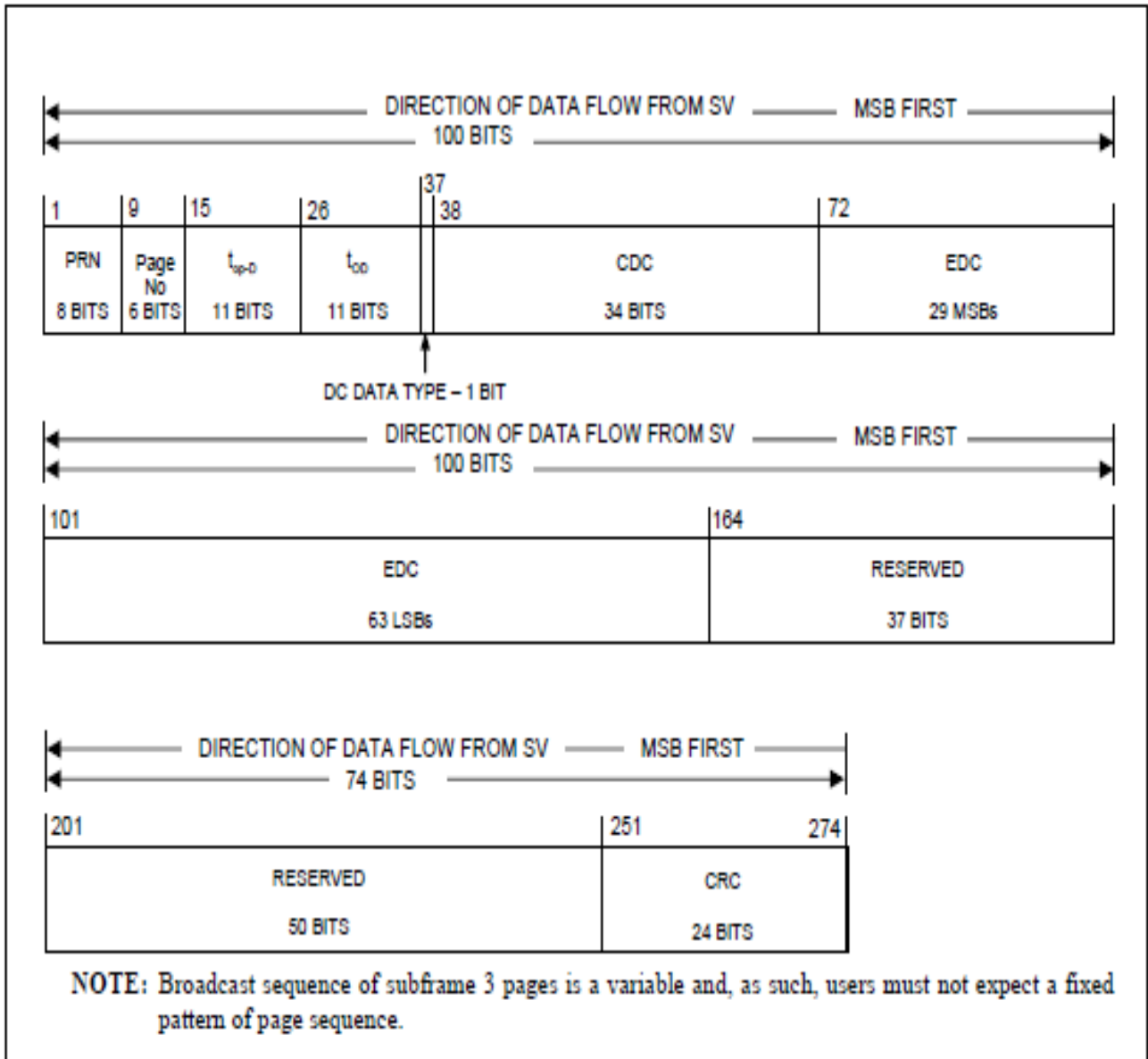
Figure 3.5-6. Subframe 3, Page 5 - Differential Correction
