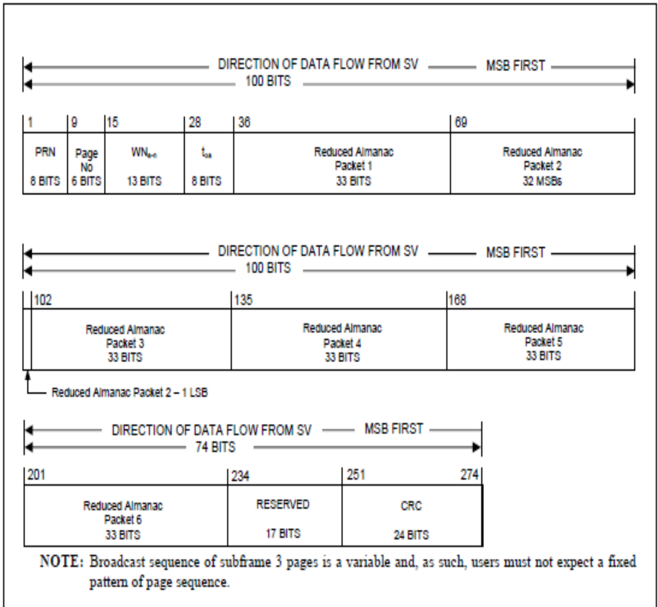
Figure 3.5-4. Subframe 3, Page 3 - Reduced Almanac
