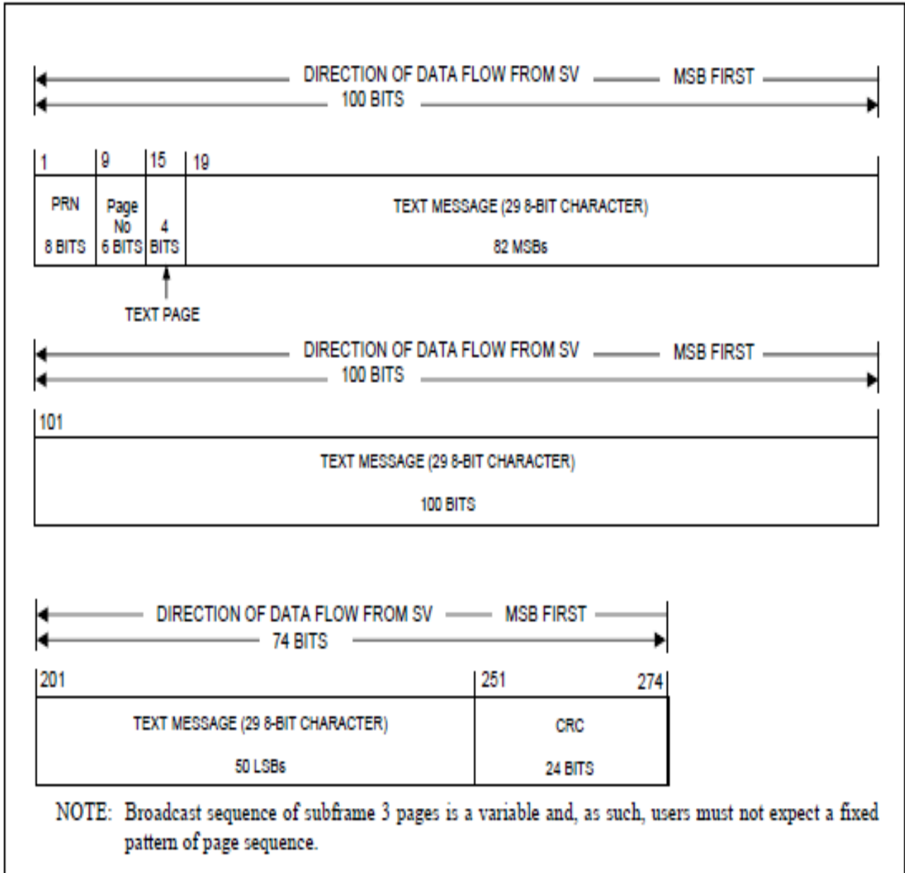
Figure 3.5-7. Subframe 3, Page 6 – Text
