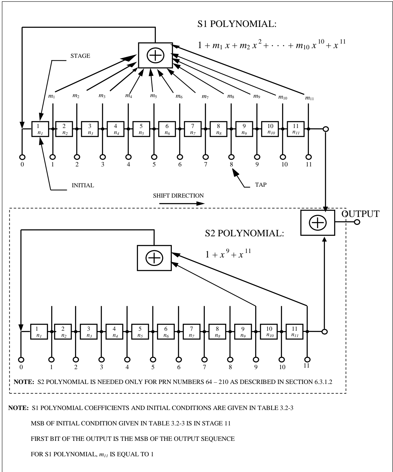
Figure 3.2-2. L1C 0 -Code Generator Configuration
