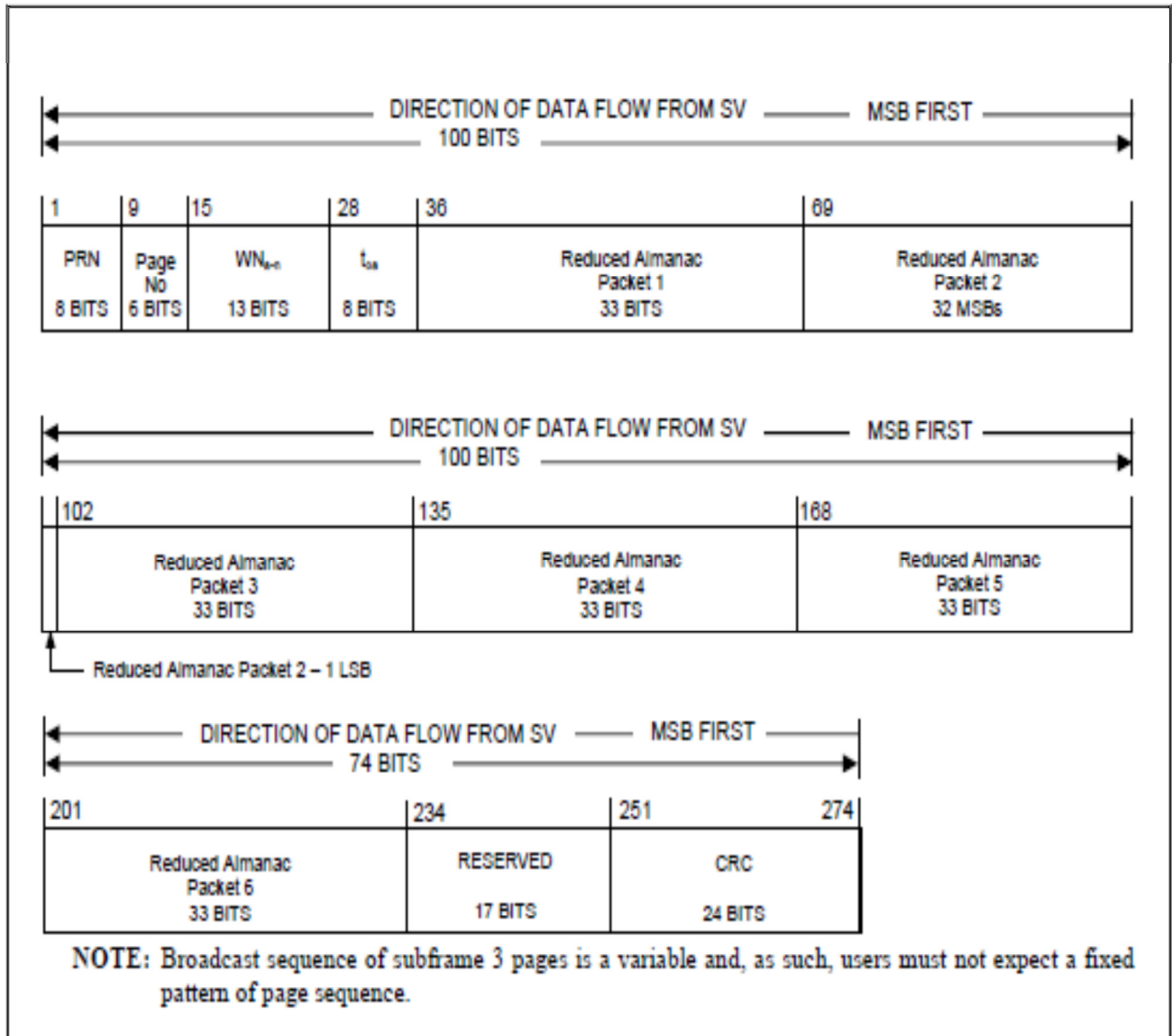
Figure 3.5-4. Subframe 3, Page 3 - Reduced Almanac
