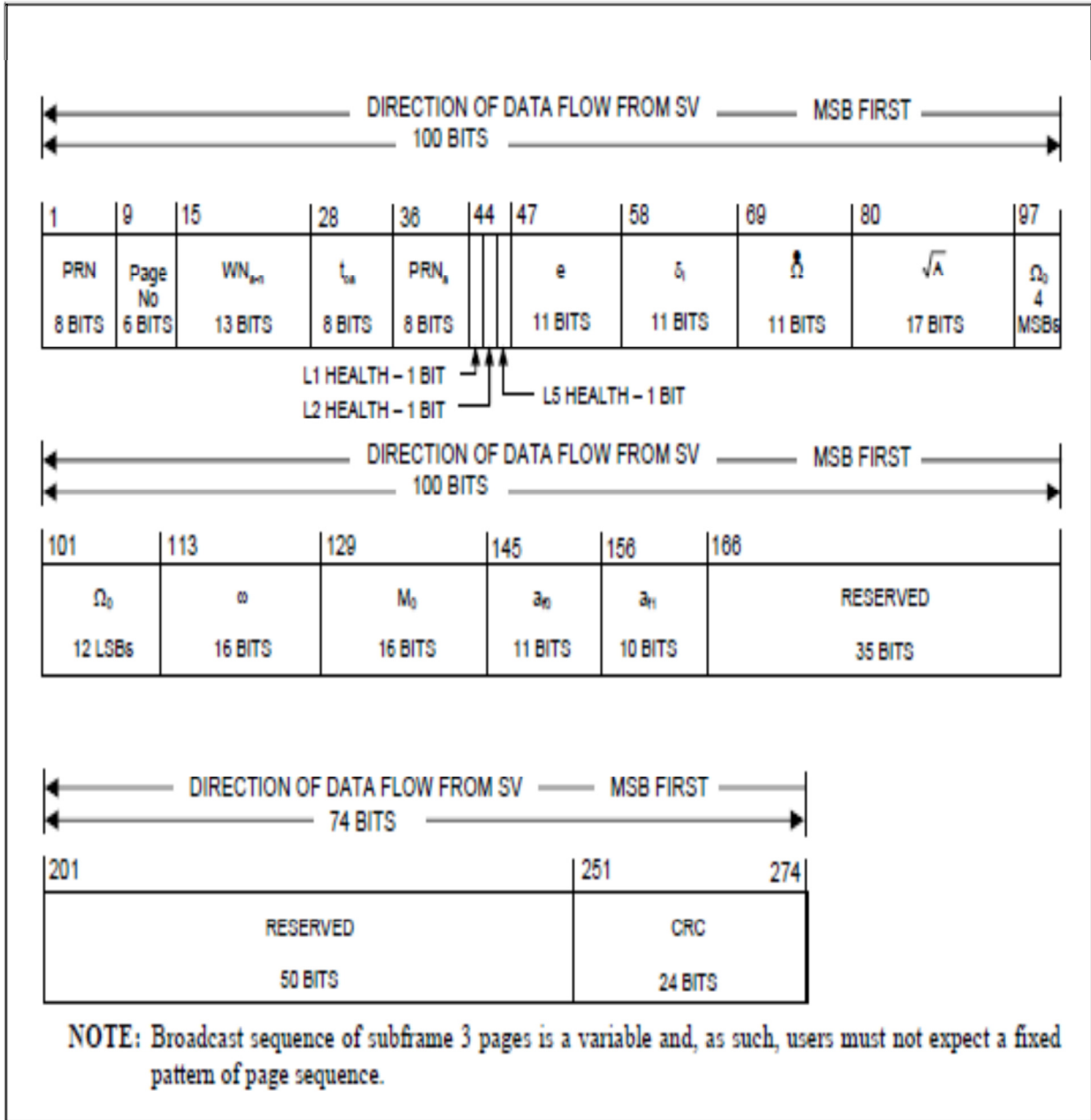
Figure 3.5-5. Subframe 3, Page 4 - Midi Almanac
