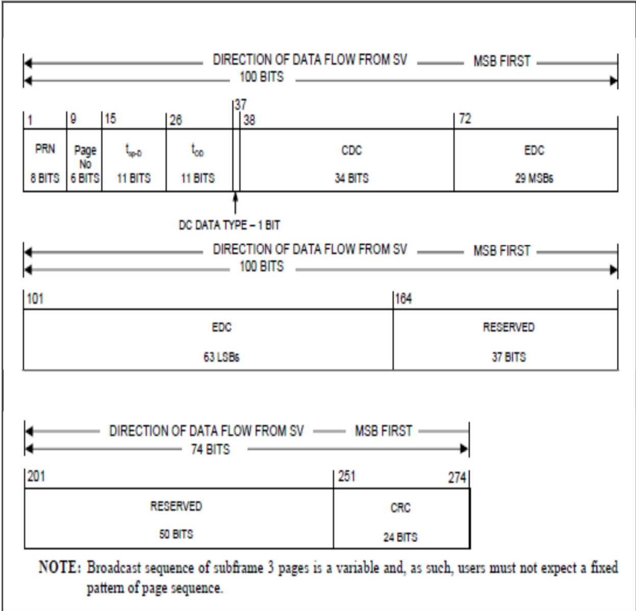
Figure 3.5-6. Subframe 3, Page 5 - Differential Correction
