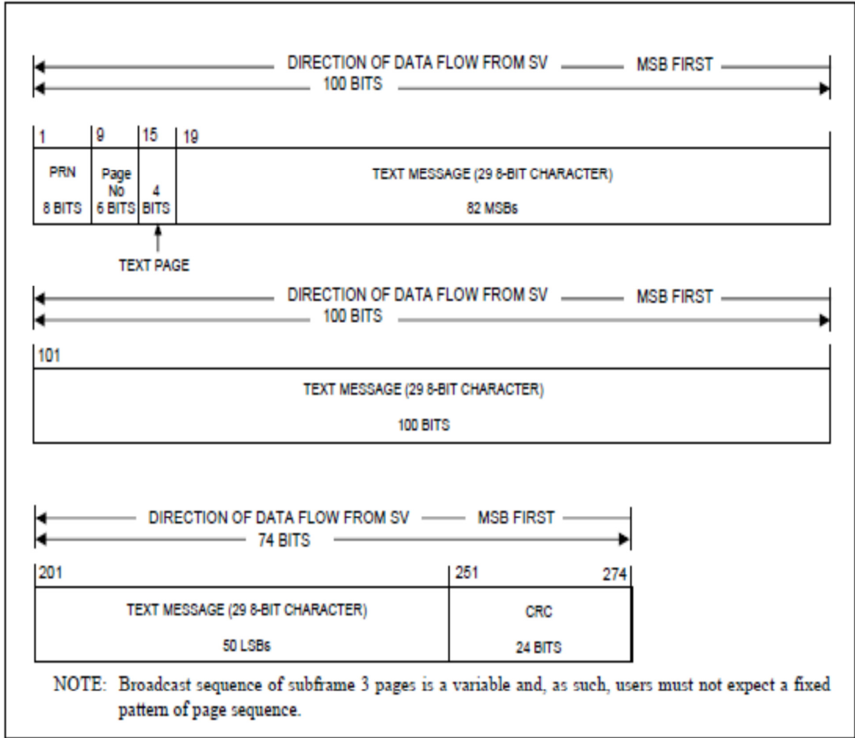
Figure 3.5-7. Subframe 3, Page 6 - Text
