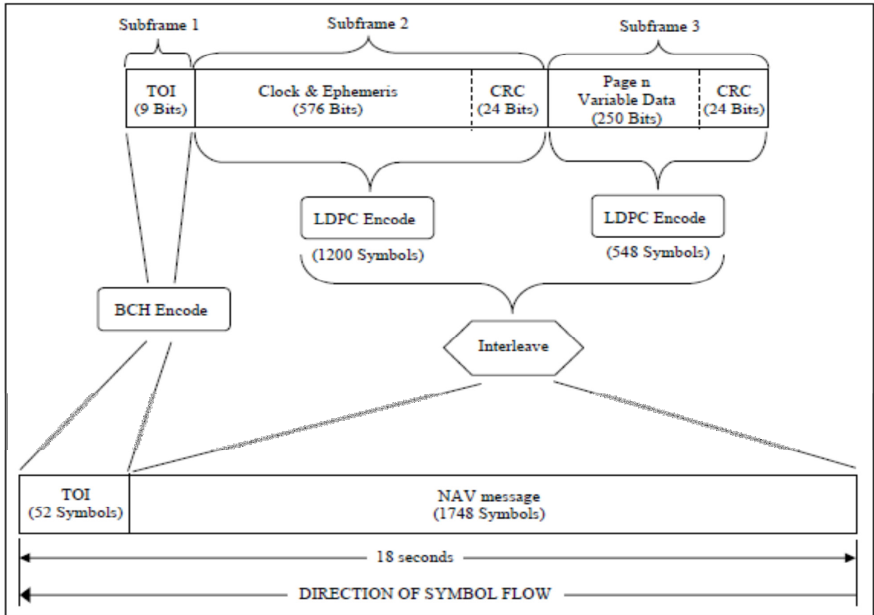
Figure 3.2-3. L1C Message Structure
