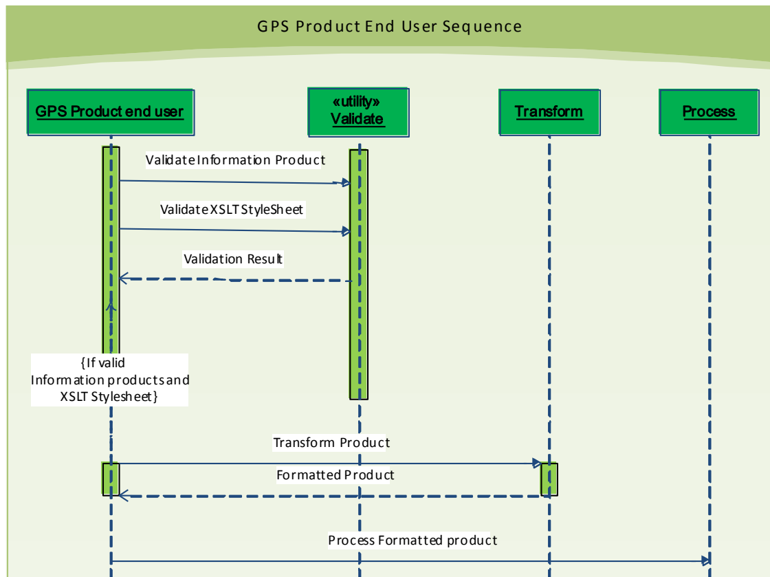
Figure 3-2 GPS Product End User Sequence Diagram
